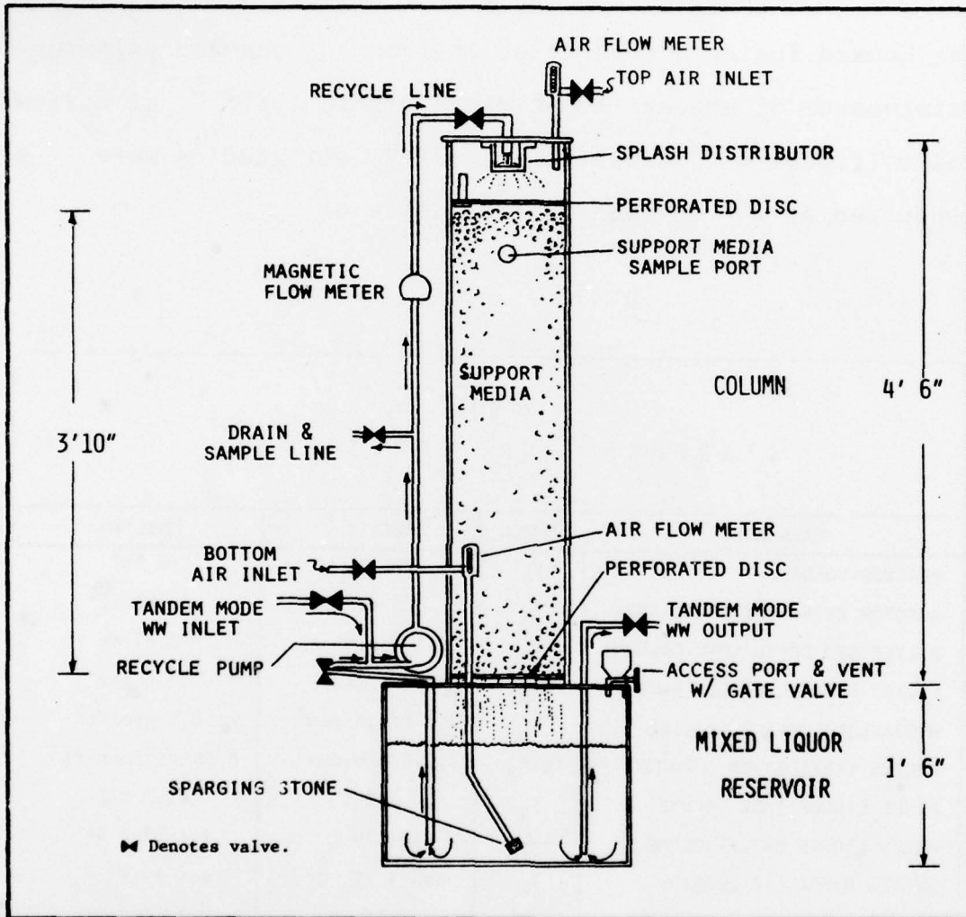
FIGURE 3. Trickle filter pilot plant schematic.
