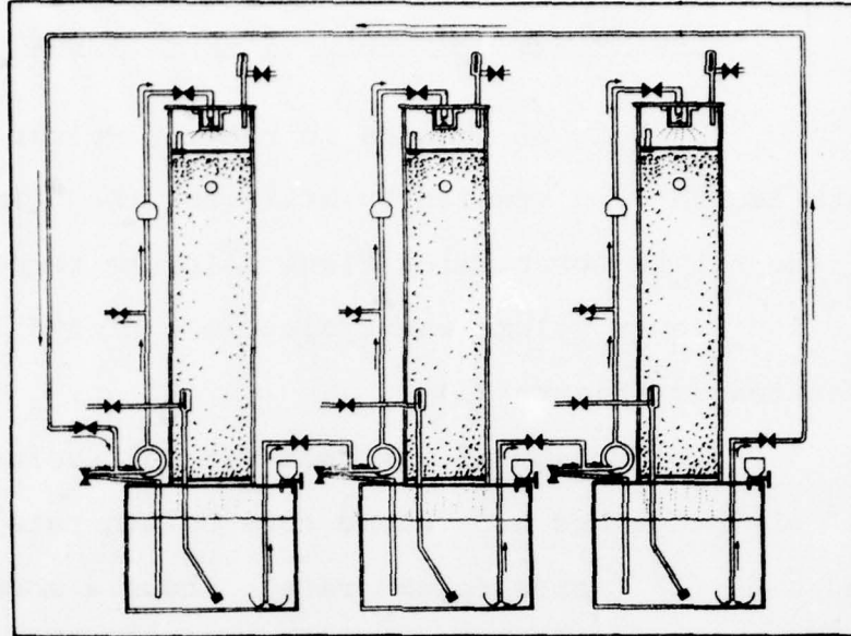
FIGURE 21. Tandem mode operation. Arrows indicate flow direction of waste water. 120 L was the total batch volume for both the tandem and isolated column run.
