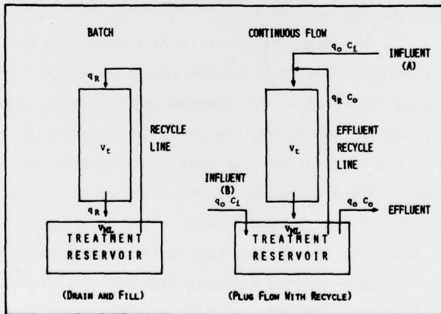
FIGURE 24. Batch and continuous flow schematics for trickling filters. Continuous flow applications may use either influent injection site A or B.
