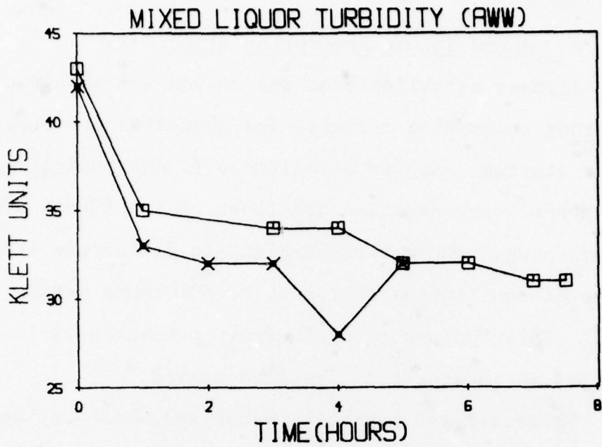
FIGURE 7. Mixed liquor turbidity from mature column runs at a batch volume of 80L.
