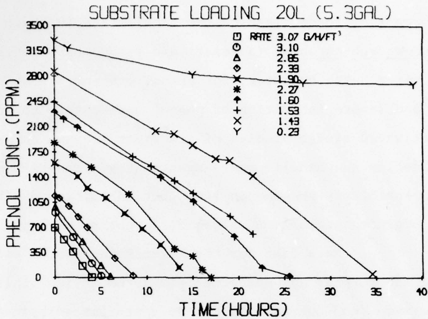
FIGURE 16a. Raw data for substrate loading runs.
