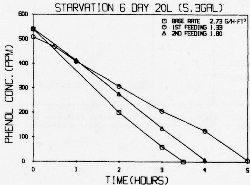
FIGURE 19. Six day starvation test.
