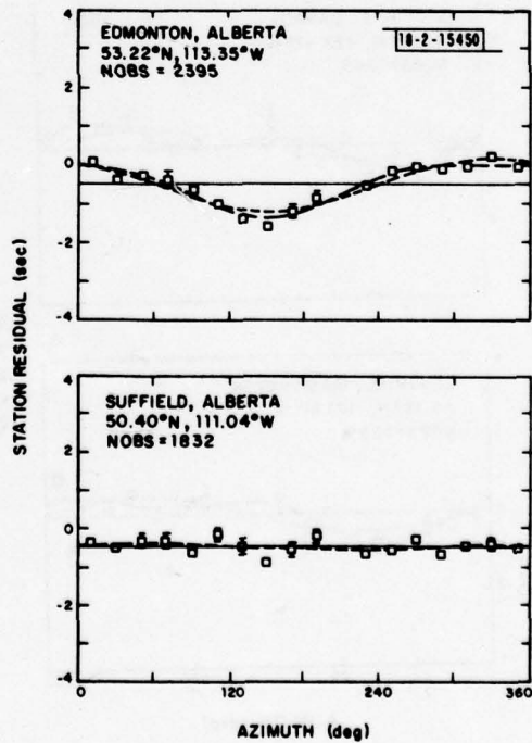
Fig. II-13. Same as Fig. II-9 but for stations Edmonton, Alberta and Suffield, Alberta. Distance between stations is 320 km. Note that pattern of residuals is entirely different at both stations. This should be compared with coherent pattern of residuals in Figs. II-10 through II-12. Inference is that source of anomaly observed at Edmonton must be rather shallow.
