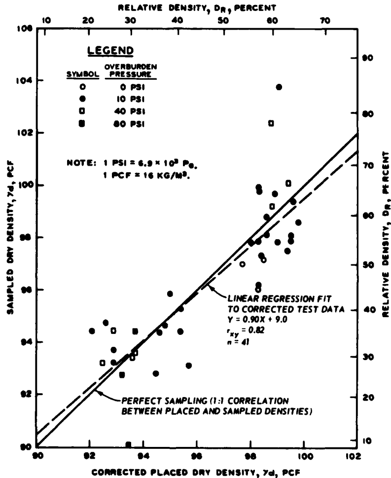
Figure 4. Effects of sampling on density of sand
