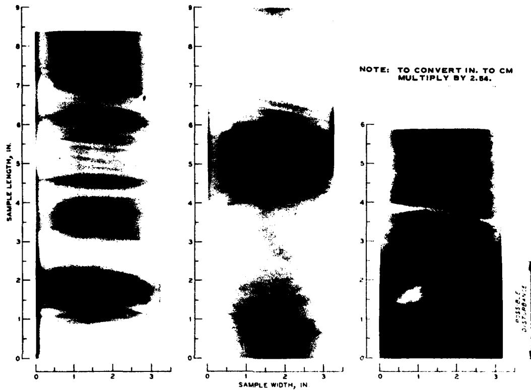
Figure 7. Use of radiograph to evaluate sample disturbance
