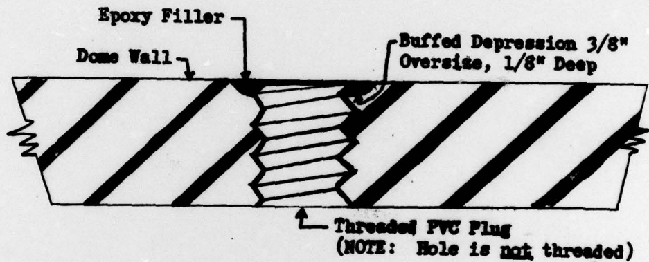
b. REPAIR OF PUNCTURE LESS THAN 1" DIA.
