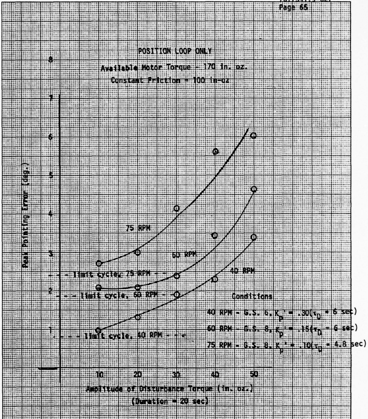
Figure 3-20. Peak Pointing Error vs. Amplitude of Disturbance Torques (Ground Position Loop Only)
