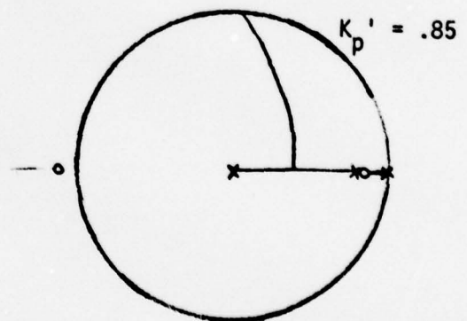
poles - (.86, 0), (.01, 0), (1, 0) GAIN STATE 8
