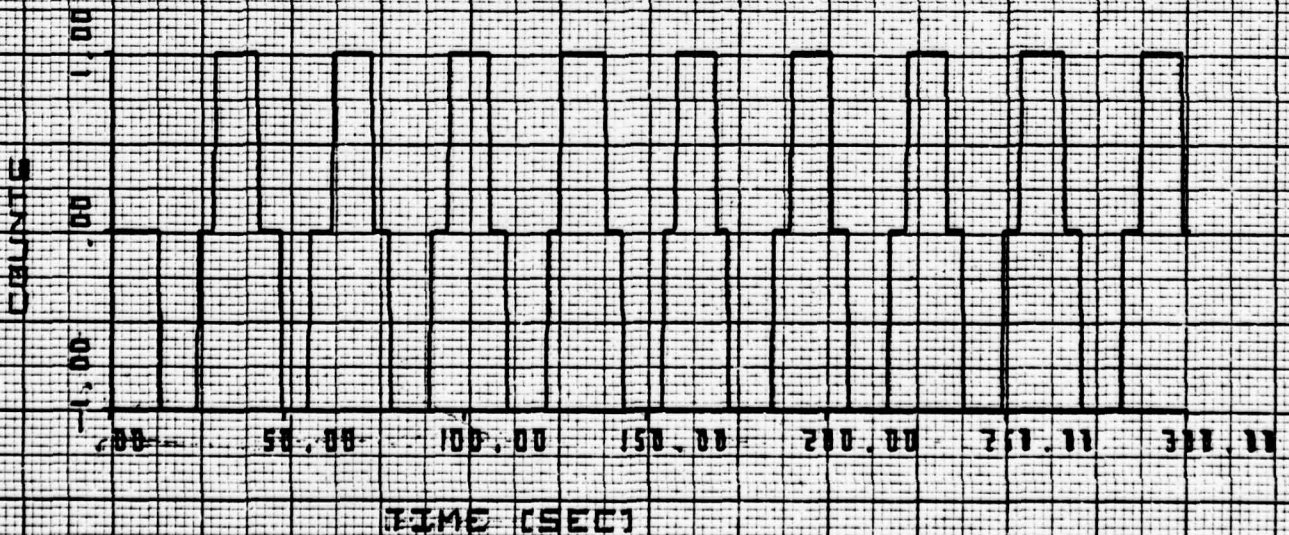
Figure 3-17 Response of Control System at 75 RPM
