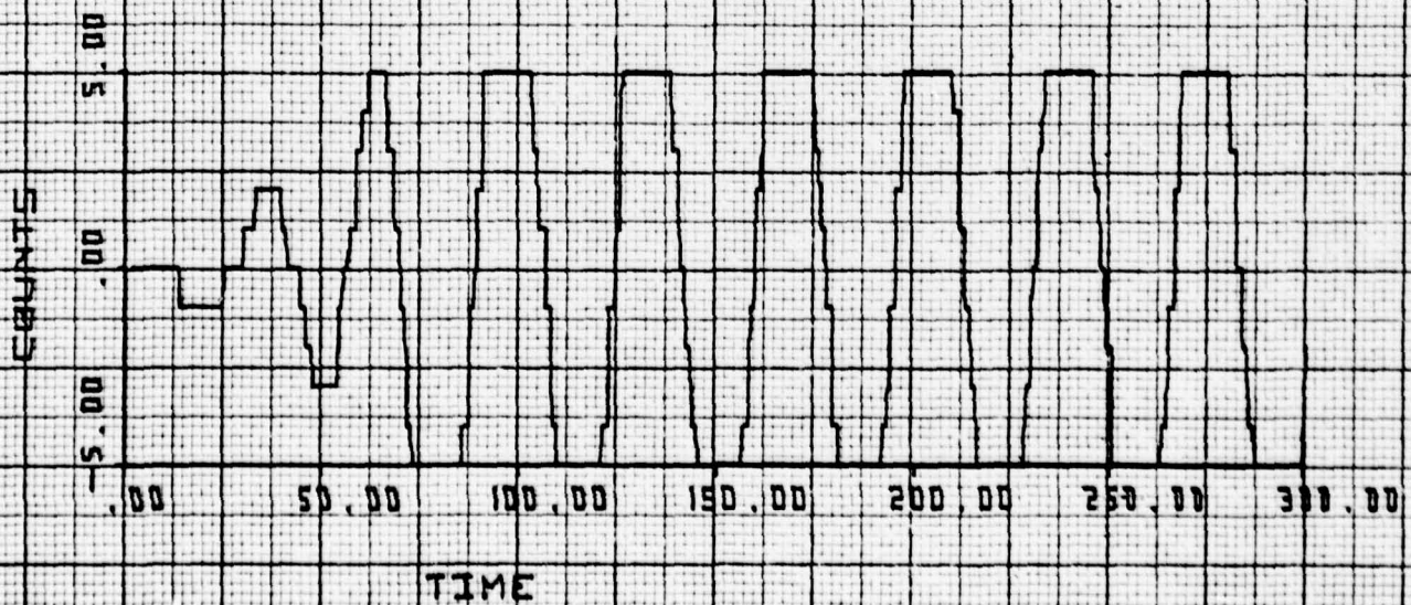
Figure 3-16 Response of Control System at 75 RPM
