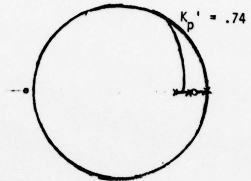
poles - (.81, 0), (.62, 0), (1, 0) GAIN STATE 6
