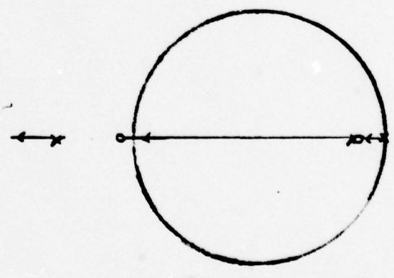
poles - (-1.57, 0), (.804, 0), (1, 0) (Unstable for all K_p' ) GAIN STATE 7
