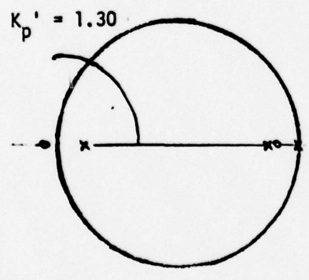
poles - (.79, 0), (-.76, 0), (1, 0) GAIN STATE 6
