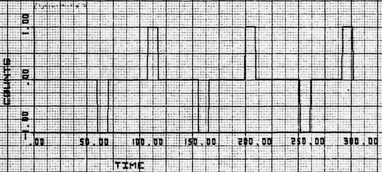
Figure 3-12. Response of System to Disturbance of 10 in. oz. for 20 sec, 60 RPM
