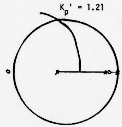
poles - (.78, 0), (-.16, 0), (1, 0) GAIN STATE 5
