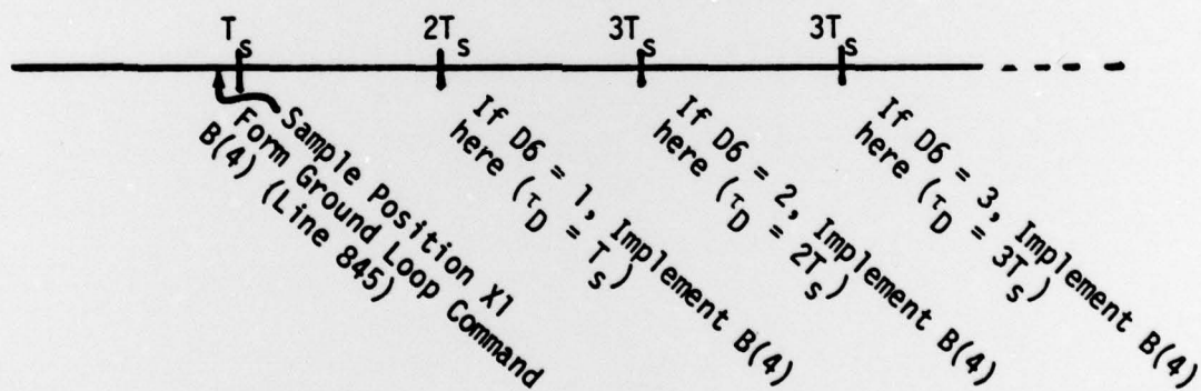
Figure B-4. Implementation of Ground Loop Relay in Simulation (Position Loop)
