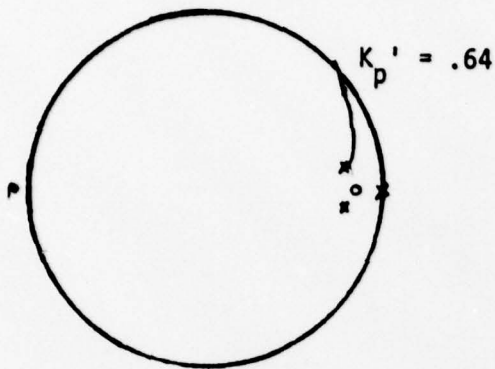
poles - (.80, ± .10), (1,0) GAIN STATE 5
