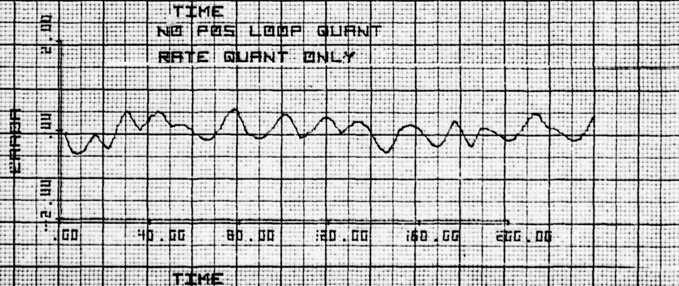
Figure 2-11. Effects of Removing Quantization, Zero-Delay System, 60 RPM
