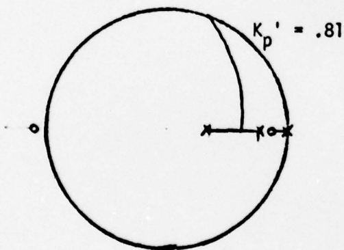
poles - (.84, 0), (.36, 0), (1,0) GAIN STATE 7
