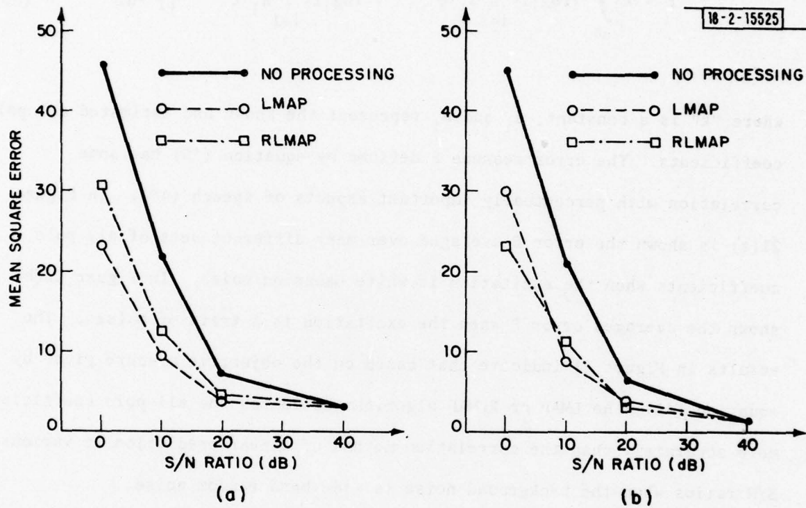
Fig. 21. Performance comparison of correlation method, LMAP and RLMAP techniques in estimating all-pole parameters from noisy synthetic data. After Lim (18). (a) Random noise excitation. (b) Pulse train excitation.
