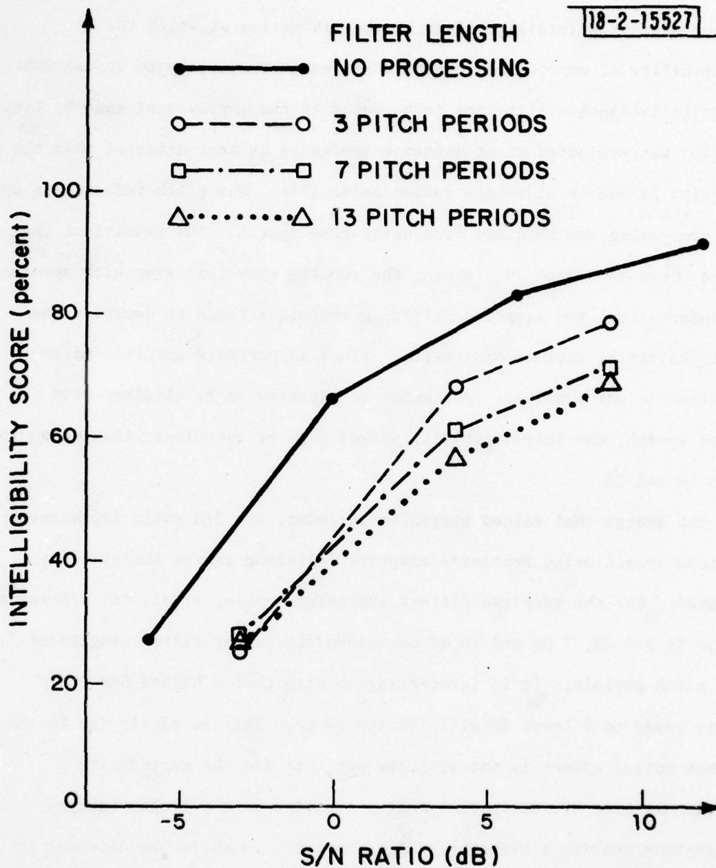
Fig. 19. Intelligibility scores of Frazier's filtering technique for enhancement of speech degraded by a competing speaker. After Perlmutter, et al (68).
