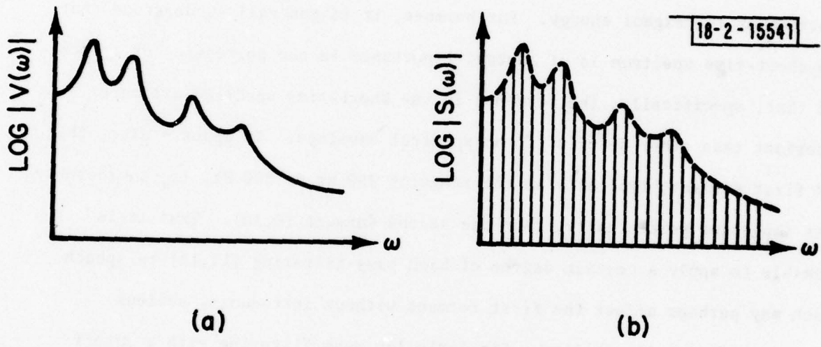
Fig. 2. An example of resonant frequencies of an acoustic cavity. (a) Vocal tract transfer function. (b) Magnitude spectrum of a speech sound with the resonant frequencies shown in Figure 2(a).
