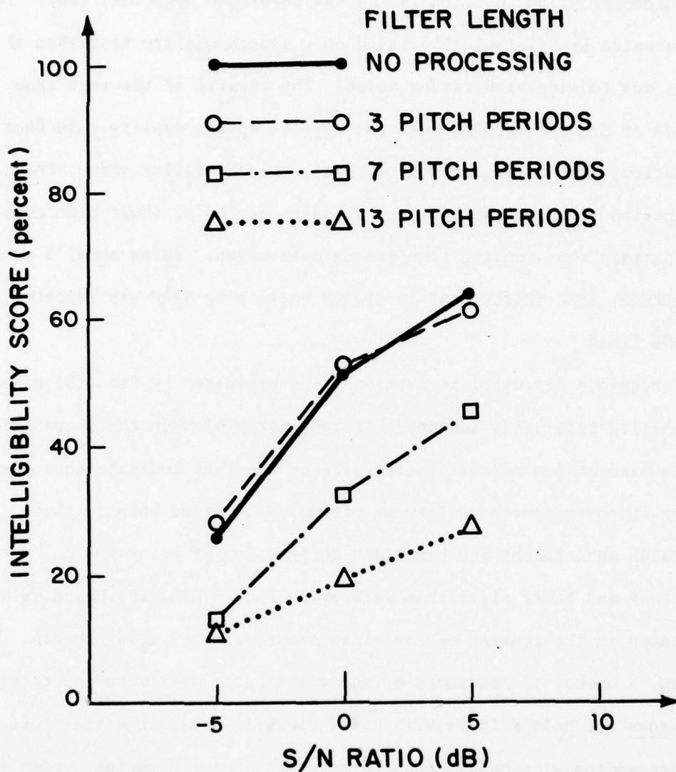
Fig. 20. Intelligibility scores of Frazier's adaptive filtering technique improved by Lim, et al (69) for enhancement of speech degraded by wide-band random noise. After Lim, et al (69).
