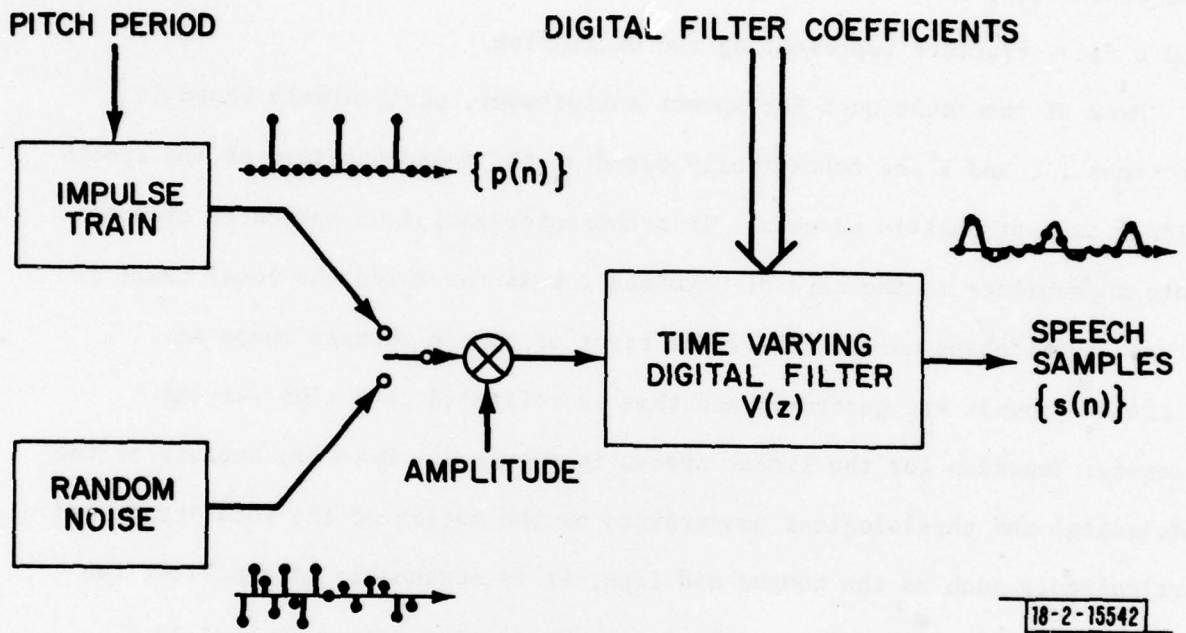
Fig. 1. A speech production model.
