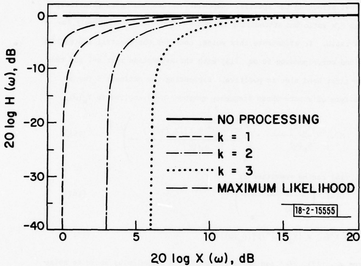
Fig. 6. Attenuation curves for two spectral subtraction techniques (eq. 13 and 14). See text for details.
