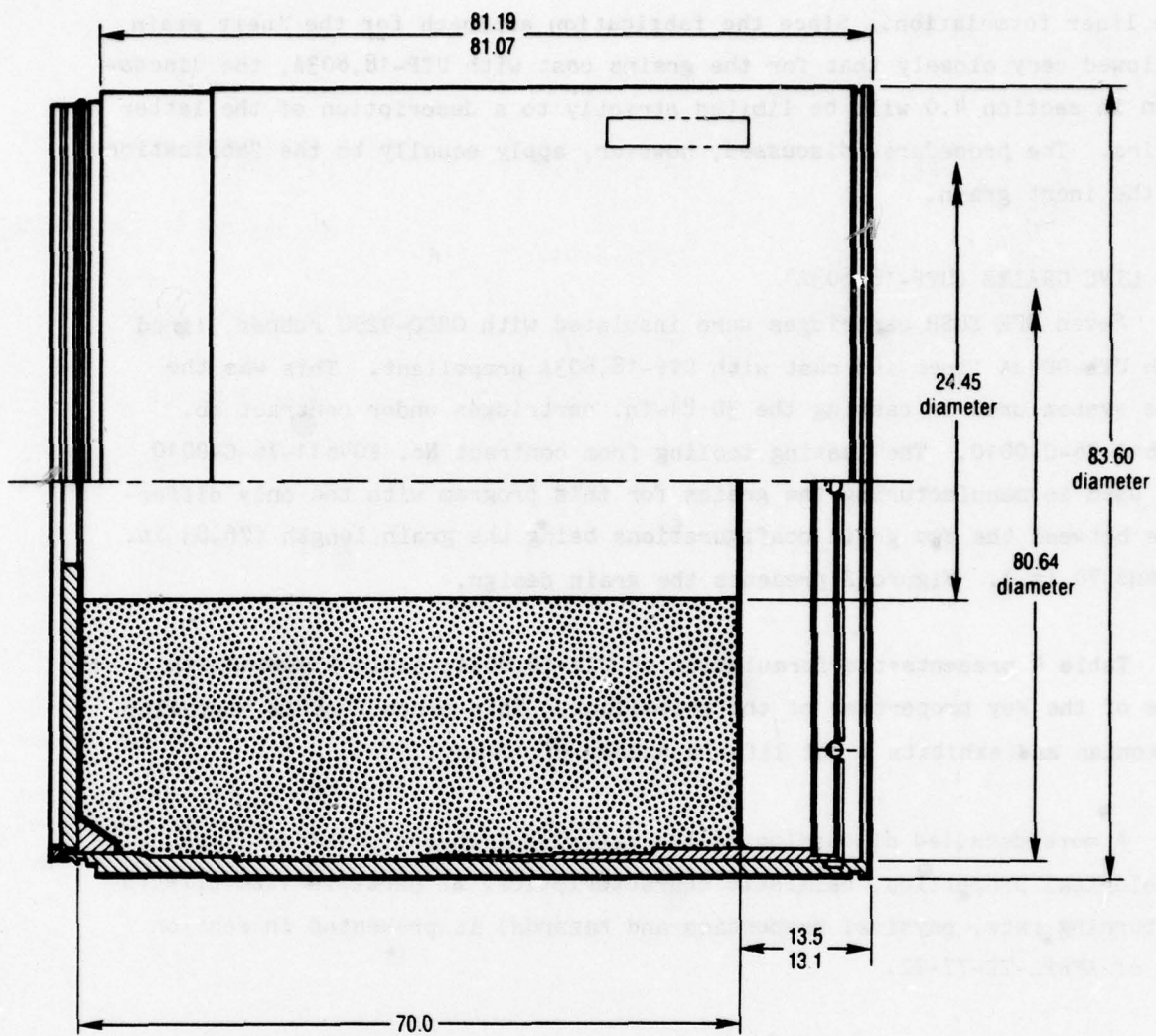
Figure 2. SLSH Grain Configuration
