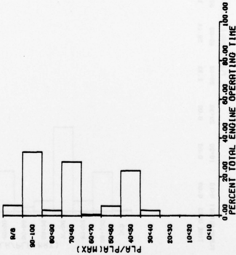
FIGURE 10. F404 TEST CYCLE 7 THROTTLE POSITION SUMMARY
