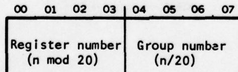
Figure 3.9 CE.n Encoding
