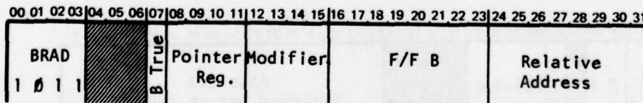
Figure 3.16 BRAD Ministep
