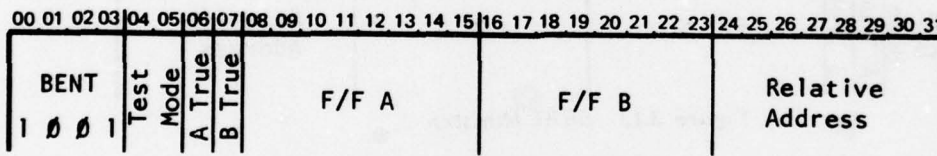
Figure 3.14 BENT Ministeop
