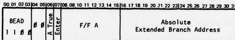
Figure 3.17 BEAD0 Ministeop
