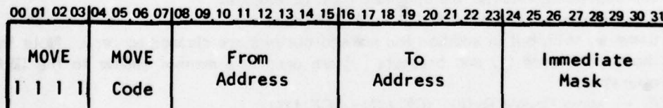
Figure 3.23 MOVE Ministep
