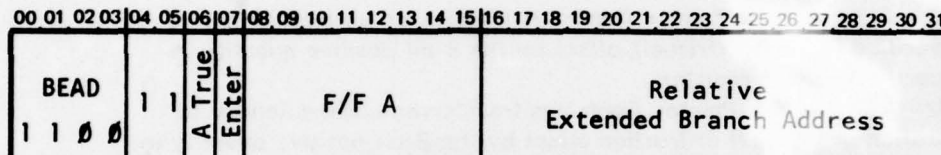
Figure 3.20 BEAD3 Ministep
