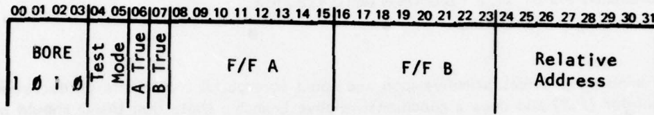
Figure 3.15 BORE Ministep
