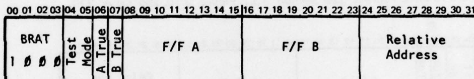
Figure 3.13 BRAT Ministep
