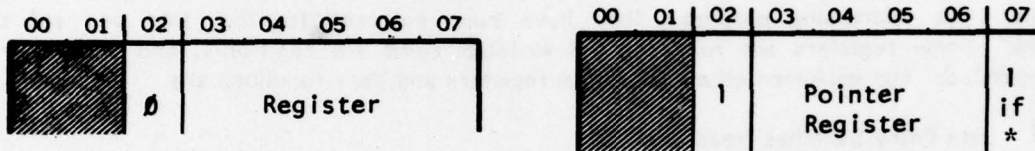
Figure 3.1 A-Operand Formats
