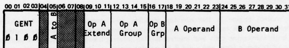
Figure 3.8 GENT Ministeop
