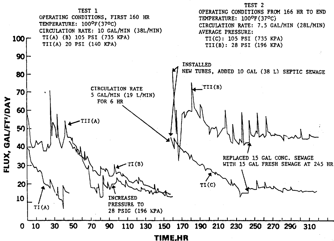
Figure 4 - Flux Vs Time Performance of Half-Inch Tubular Ultrafiltration Membranes Processing Nonaerated Raw Sewage
