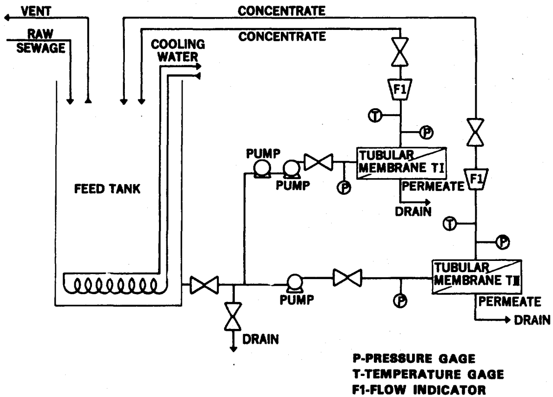
FIGURE 1 UTRAFILTRATION TEST SYSTEM SCHEMATIC
