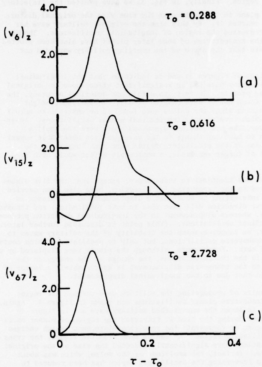
Figure 3. Effects of longitudinal planar oscillations on solitary-wave profile. (a), (b), and (c) represent solitary wave before, during, and after traversing the oscillatory region, respectively.
