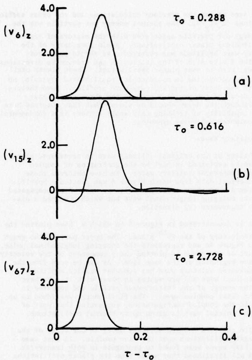
Figure 4. Effects of transverse and longitudinal oscillations on solitary-wave profile. (a), (b), and (c) represent solitary wave before, during, and after traversing oscillatory region, respectively.
