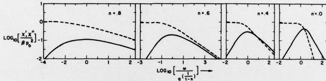
Fig. 5. The behavior of \chi' , \chi'' in the present theory for several different values of n . Note the peak shape is independent of a \equiv e^{-n\gamma} / (1-n)\tau_0 E_c^n but strongly dependent on n . The slope m of each of these \log(\chi'') versus \log(\omega) plots varies continuously from zero to one for \log(\omega) < \log(\omega_p) , where \omega_p is the post peak position. m for a fixed decrement of \log(\omega) , i.e. at a value of \omega with \log(\omega/\omega_p) < 0 and fixed) decreases as n increases. In view of this property one should not take the asymptote of the lowest available frequency measurements of \chi''(\omega) and attach a universal meaning to the slope of that asymptote but rather analyze the local slope m at a fixed decrement below the post peak.
