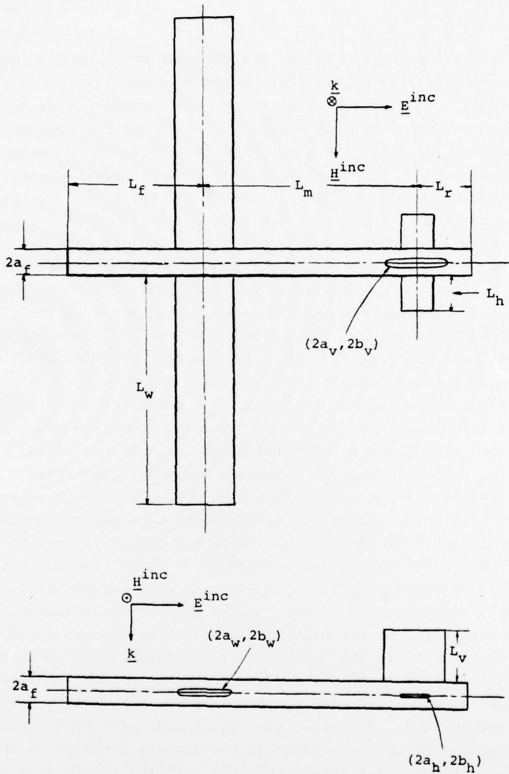
Figure 10. Magnetic Field Integral Equation Aircraft Model.
