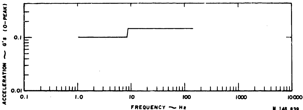
Figure 15.--Vibration spectrum envelope--ship.
