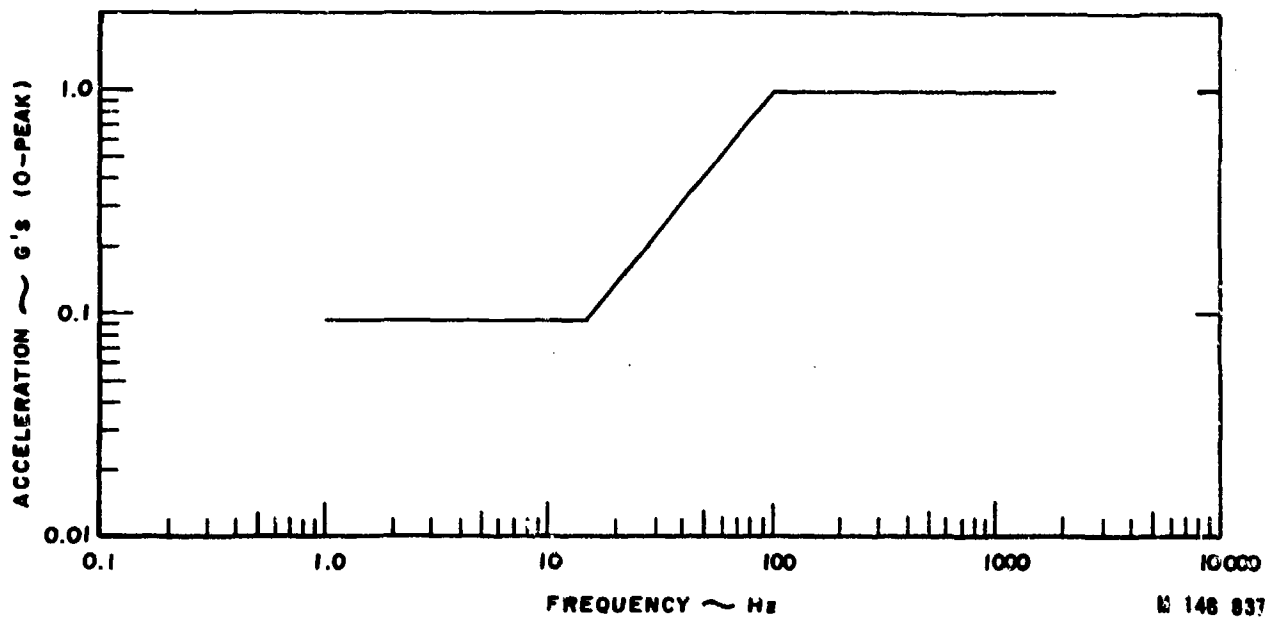
Figure 13.--Acceleration envelope--aircraft.
