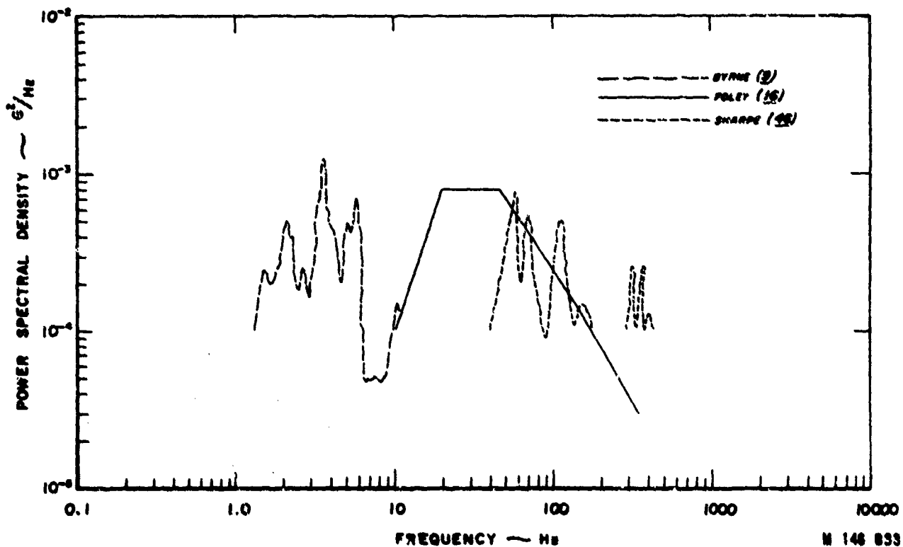
Figure 9.--Railcar frequency spectra--summary of PSD data.
