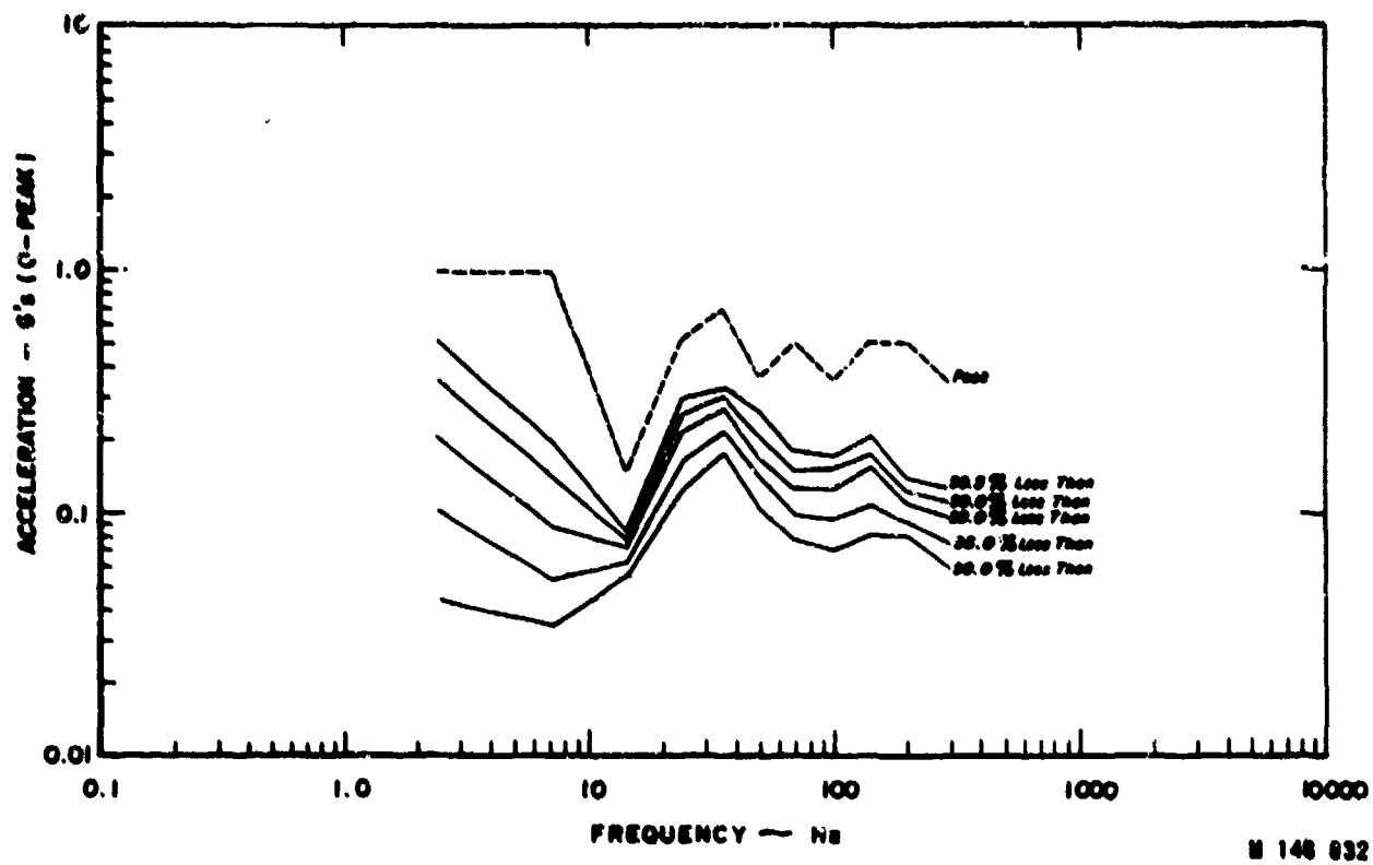
Figure 5.--Frequency spectra for various probabilities--railroad (vertical direction, composite of various conditions).
