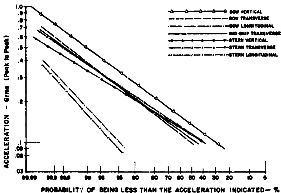
Figure 14.--Wave-induced acceleration versus probability of occurrence (520-ft. cargo ship).
