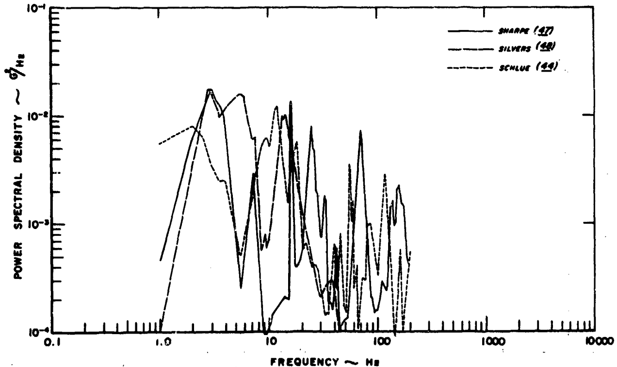
Figure 6.--Truck frequency spectra--summary of PSD data.
