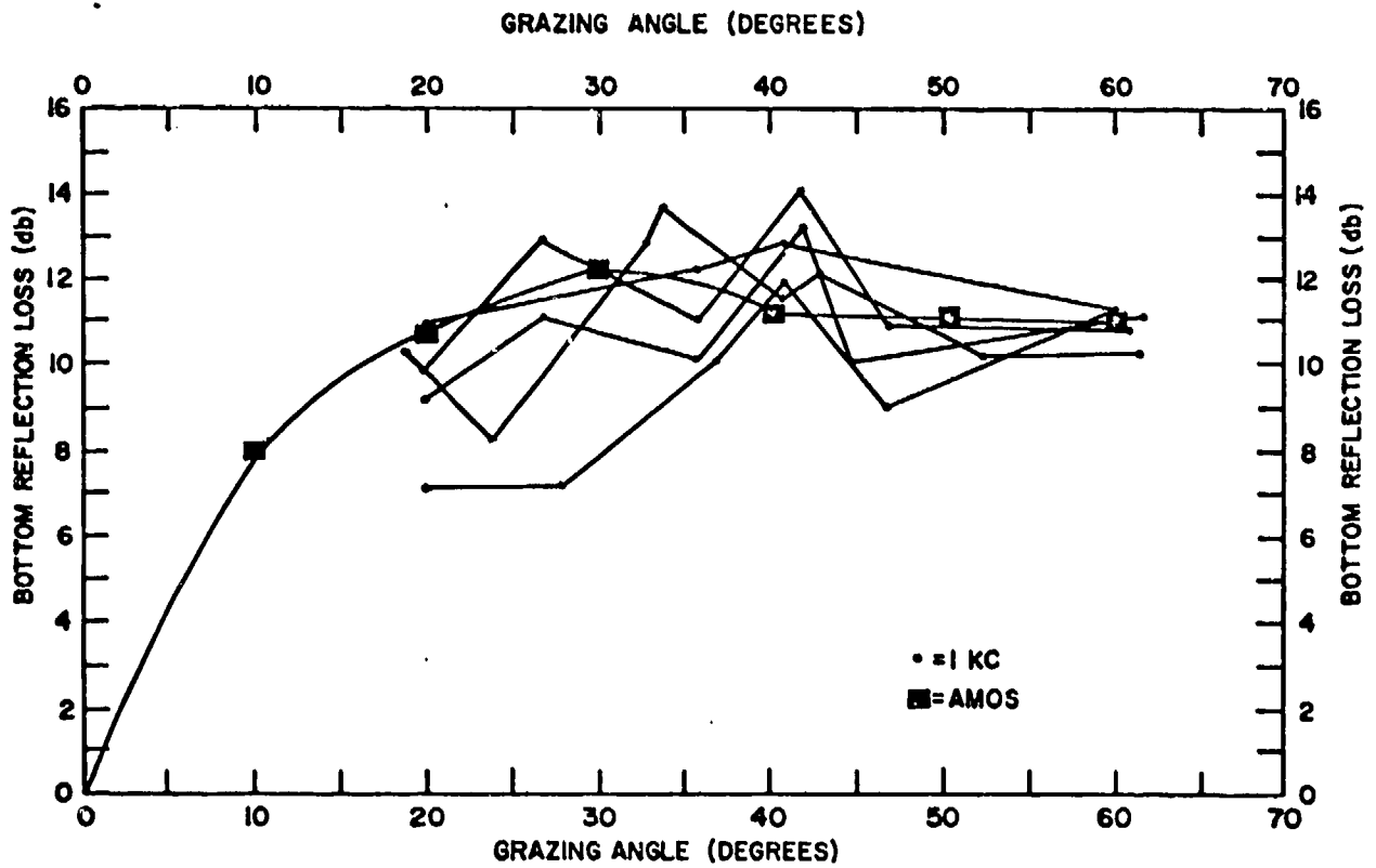
FIGURE 6 COMPOSITE OF TRUE BOTTOM LOSS AND AMOS BOTTOM LOSS
