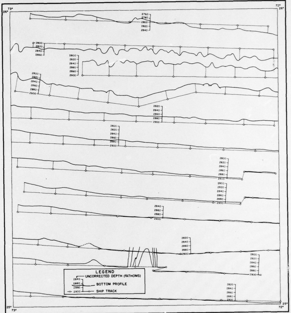
FIGURE II BATHYMETRIC PROFILES
