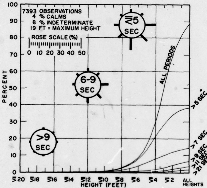
FIGURE 10 WAVES FOR APRIL, MAY, AND JUNE AREA (24°-26°N, 72°-74°W)
