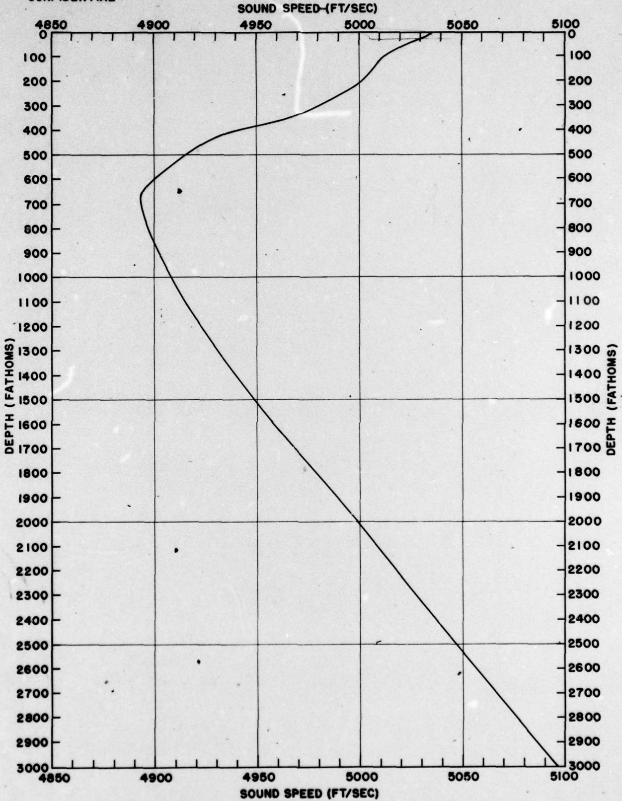
FIGURE I TYPICAL SOUND SPEED PROFILE FOR MAY
