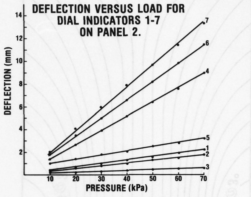
Figure 28. Intrapanel Deflection.
