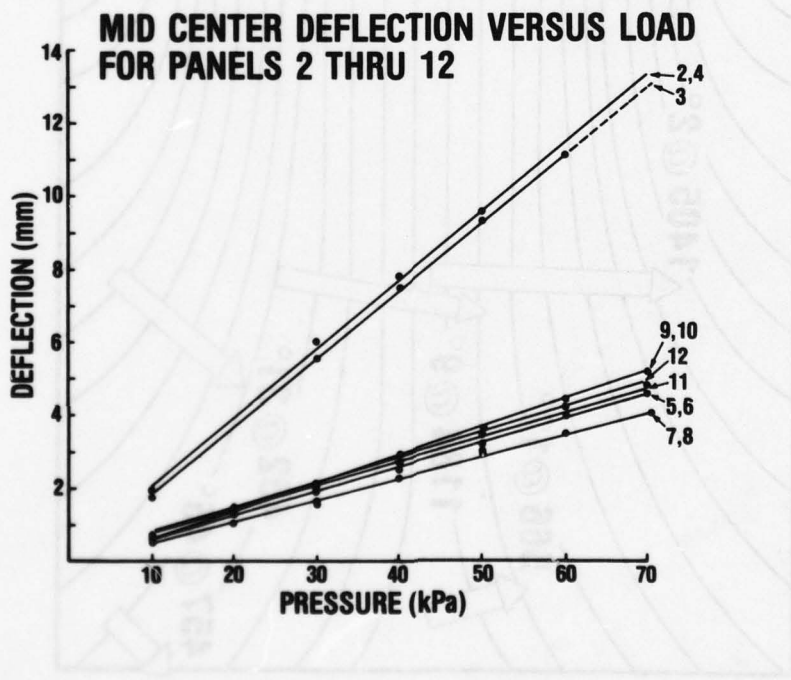
Figure 29. Interpanel Deflection.
