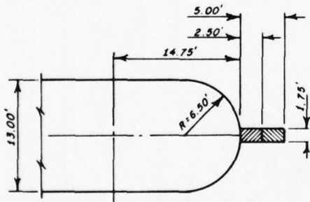
ROUND PIER NOSE
