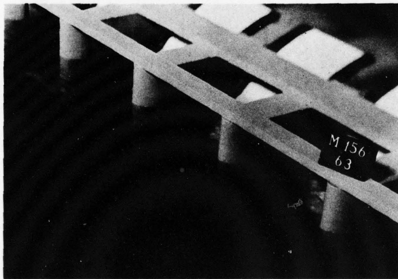
Piers without surge suppressors.
