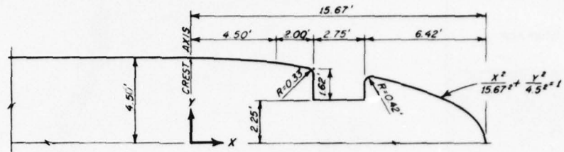
HALF PLAN PIER DETAIL
