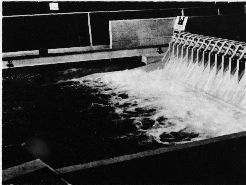
Spillway discharge 440,000 cfs, tailwater elev 797.5.
