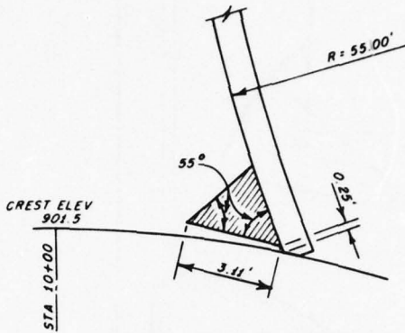
MODIFIED GATE LIP
