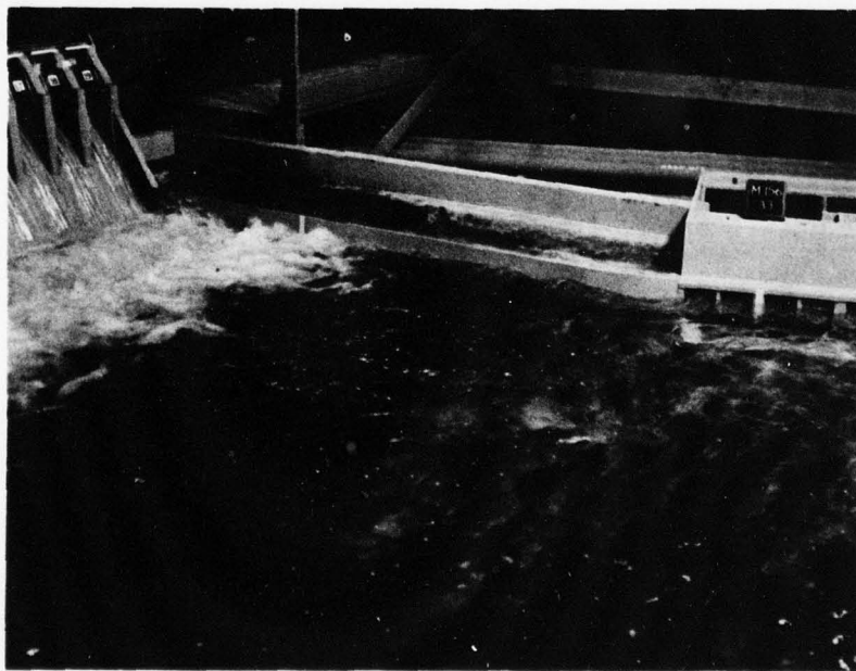
Spillway discharge 242,000 cfs, 27 powerhouse units operating.
