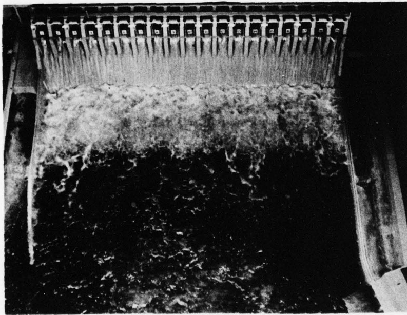
Spillway discharge 440,000 cfs, tailwater elev 797.5.
