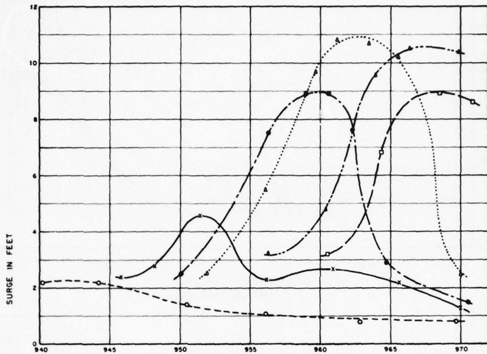
WITHOUT SURGE SUPPRESSORS
