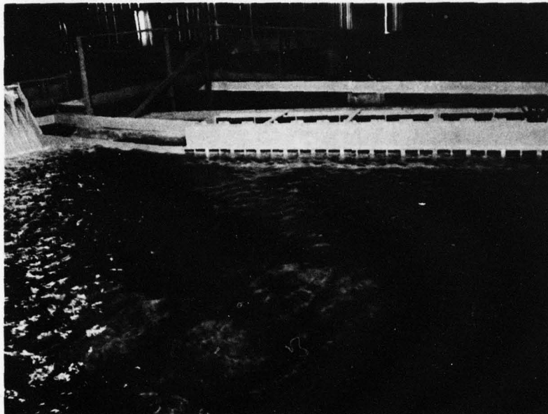
Spillway discharge 440,000 cfs.
