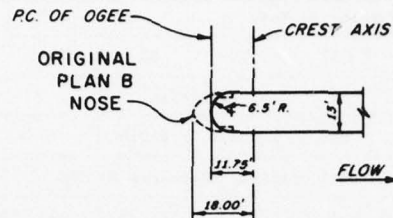
PIER NOSE DETAILS
