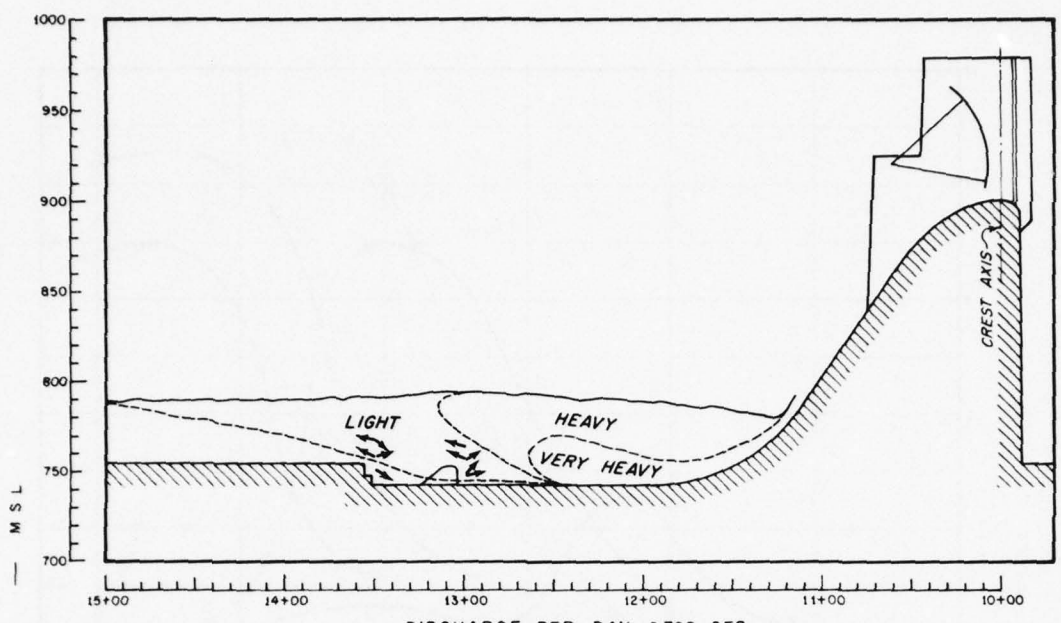
DISCHARGE PER BAY 6 720 CFS TAILWATER ELEV 790.0
