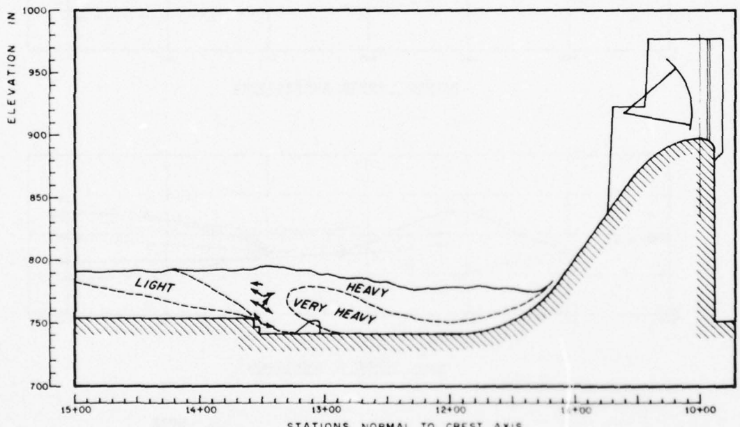
STATIONS NORMAL TO CREST AXIS DISCHARGE PER BAY 9 150 CFS TAILWATER ELEV 792.3
