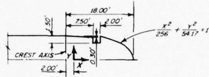
DETAIL FINAL DESIGN PIER
