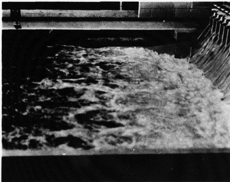
Spillway discharge 750,000 cfs, tailwater elev 809.8.
