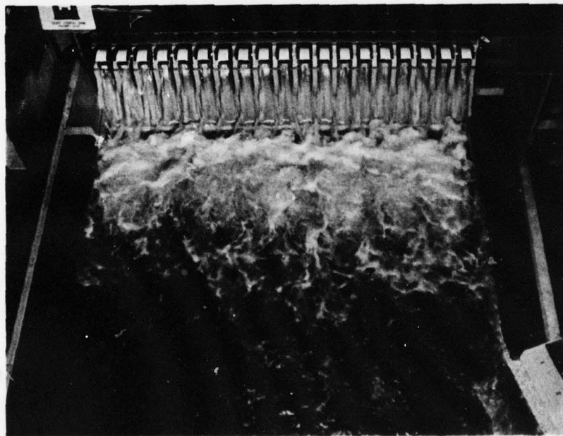
River and spillway discharge 1,200,000 cfs, tailwater elev 825.0.
