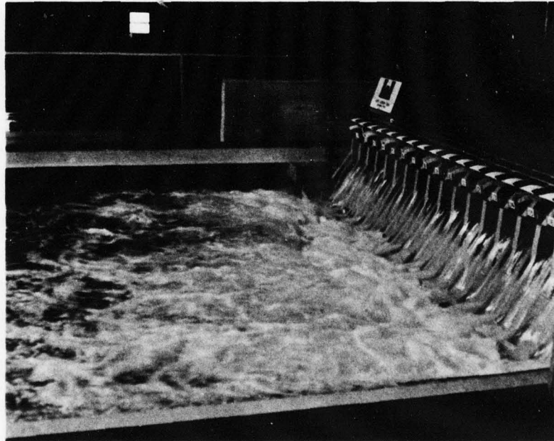
Stilling basin and north training wall.
