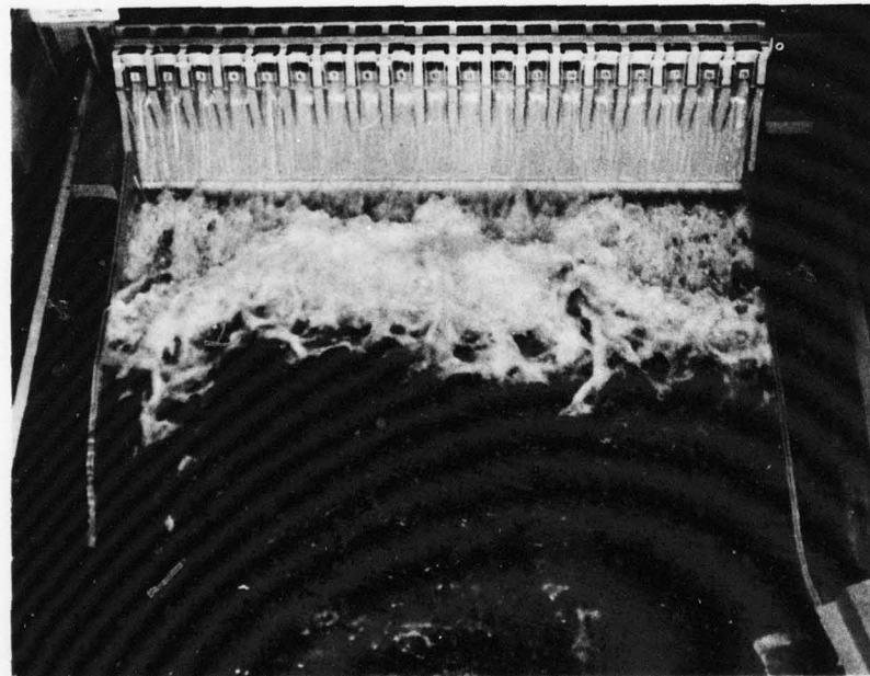
Nonuniform spillway operation (no surging).
