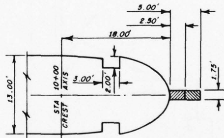
ELLIPTICAL PIER NOSE
