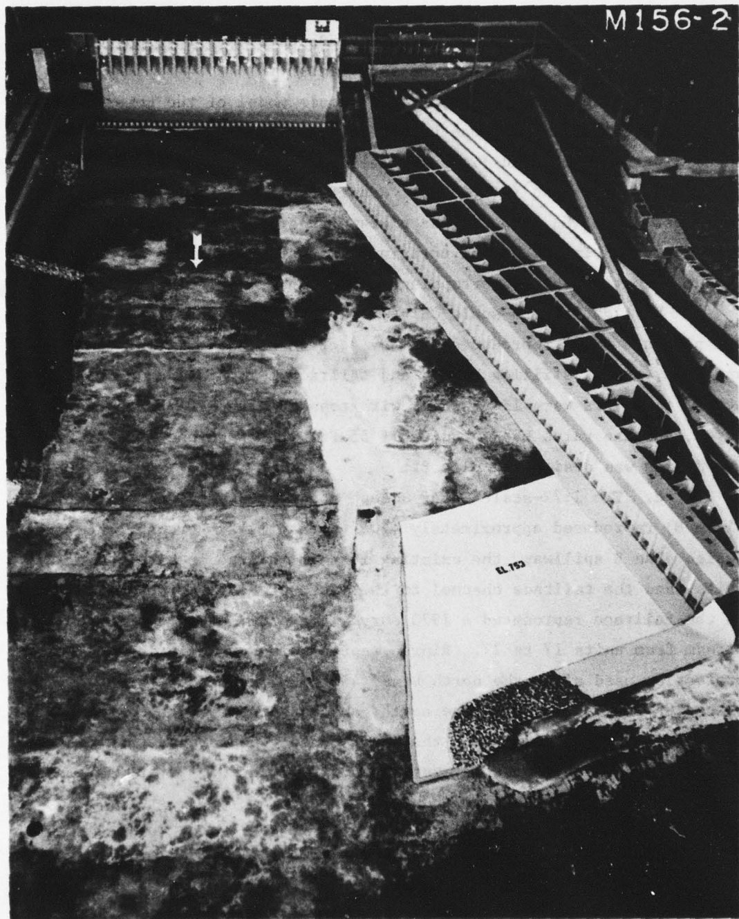
Fig. 2. 1:72-scale comprehensive model
