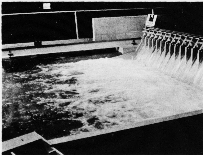
Spillway discharge 750,000 cfs, tailwater elev 809.8.
