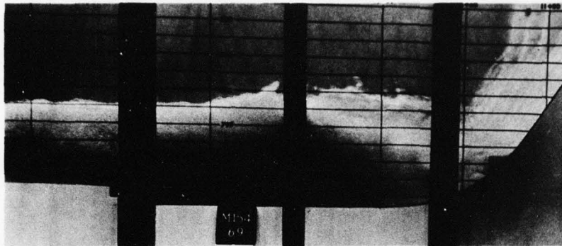
River discharge 440,000 cfs (16,390 cfs per bay), 100-year flood, pool elev 956.0, tailwater elev 798.5, 18 powerhouse units operating.
