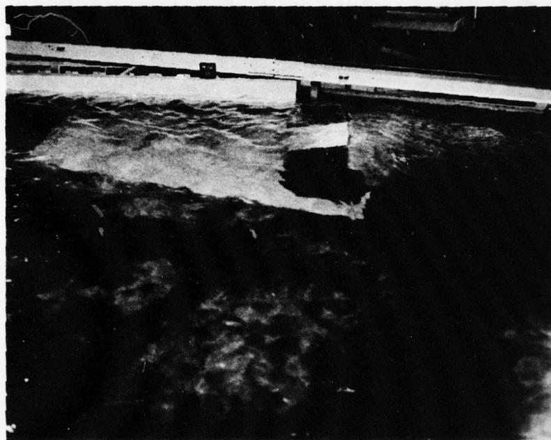
Photograph 22. Flow conditions at downstream end of powerhouse and Foster Creek; river and spillway discharge 1,200,000 cfs, tailwater elev 825.0.
