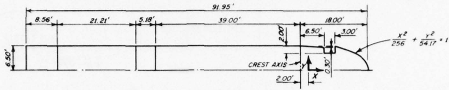
HALF PLAN PLAN B PIER
