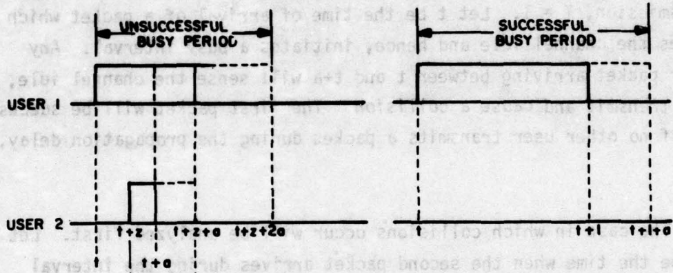
Figure 1 - LWT CSMA CHANNEL BUSY PERIODS
