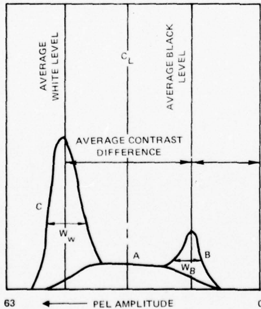
Figure B1. Ideal typewritten image pel brightness histogram.
