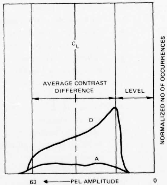
Figure B2. Ideal continuous-tone pel brightness histogram.
