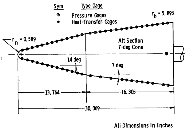
Fig. 3. The 14 to 7-deg Biconic Model
