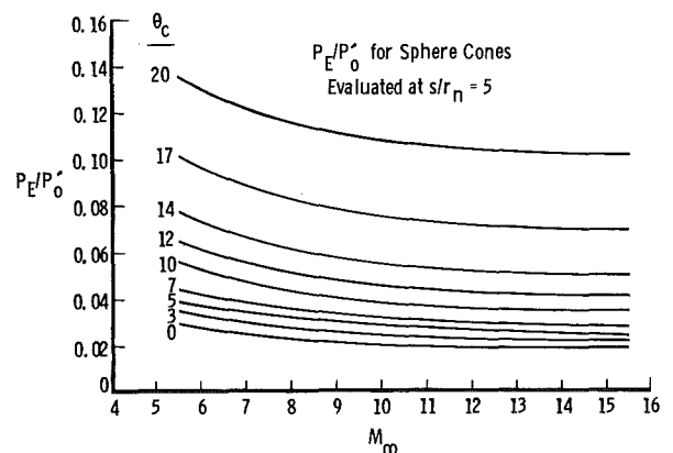
Fig. A-2. Inviscid 3-D Characteristics Pressure Ratio for s/r_n = 5
