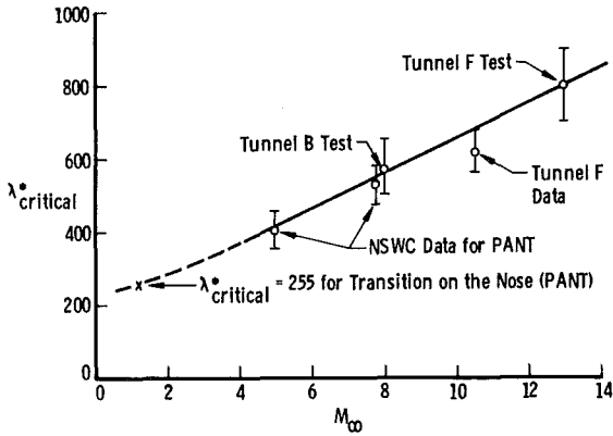
a. Mach Number Effects on \lambda_{critical}^*
