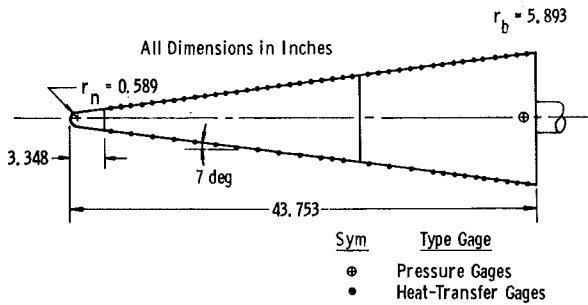
Fig. 2. Large Pressure-Heat-Transfer Model (7-deg Cone)
