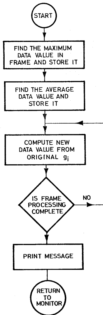
Figure 7(b). Flowchart for implementation of the algorithm
