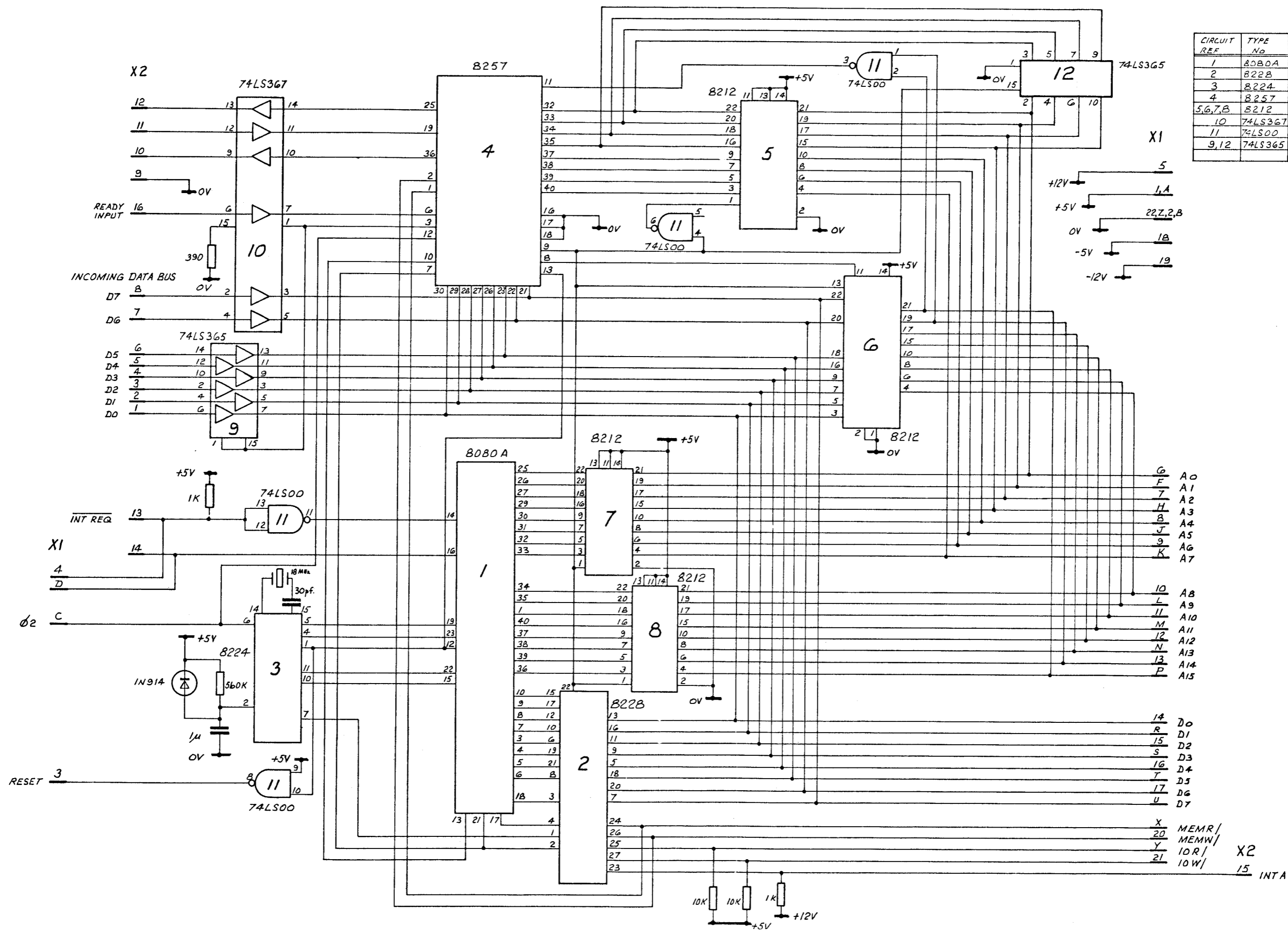
Figure 2. Circuit diagram of the CPU/DMA Controller Board
