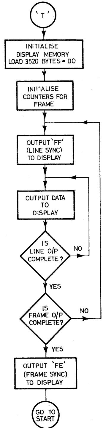
(c) Flowchart to display stored frame via Tektronix monitor
