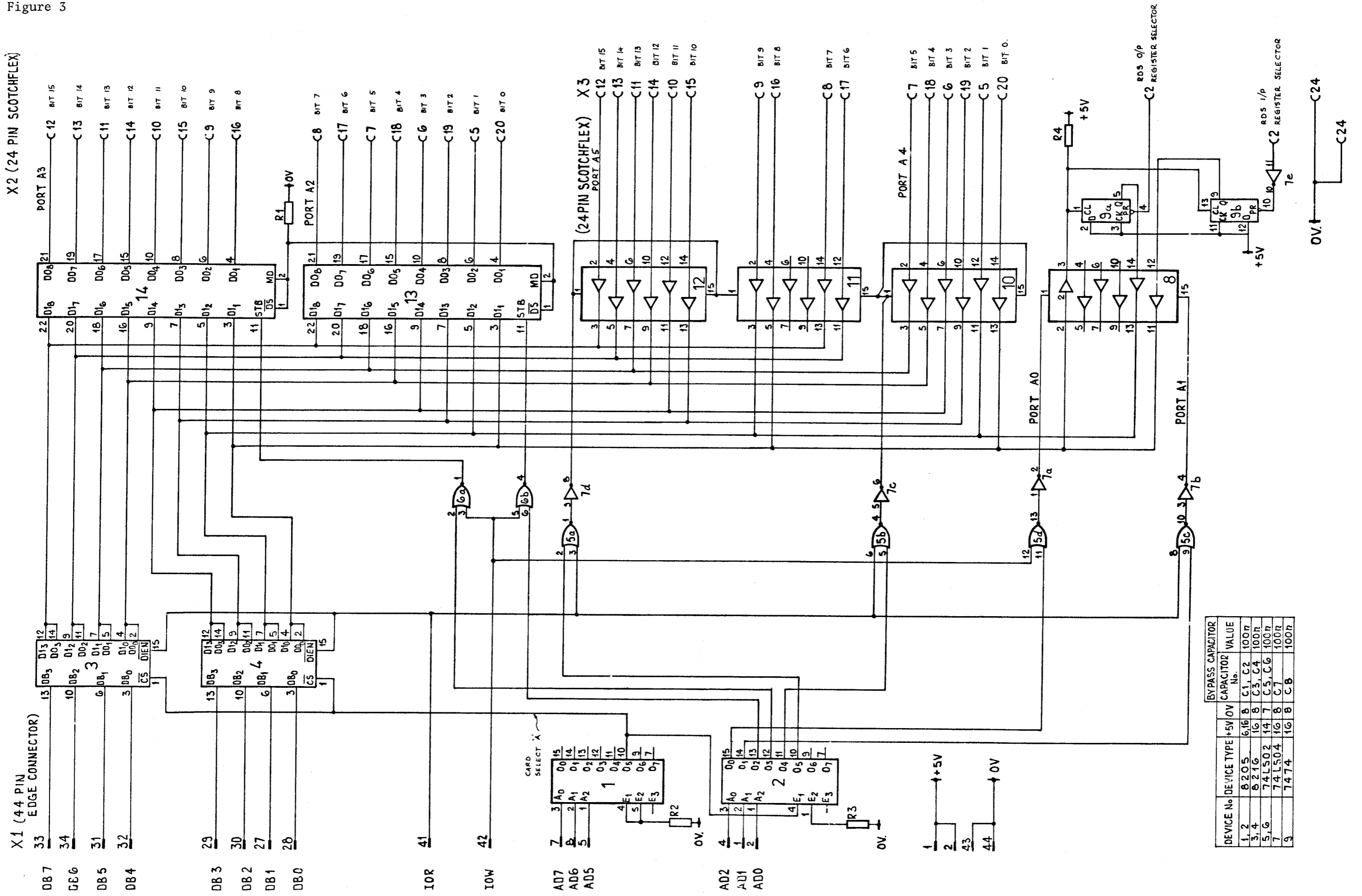
Figure 3. Circuit diagram of the Remote Data Station Interface
