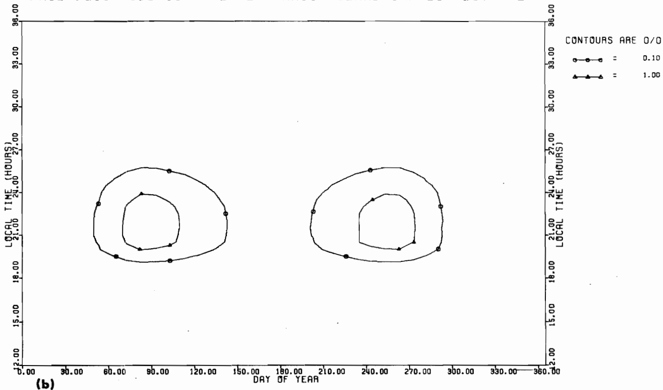
Figure 9. Diurnal and seasonal variations of propagation conditions on the Manus Island circuit
