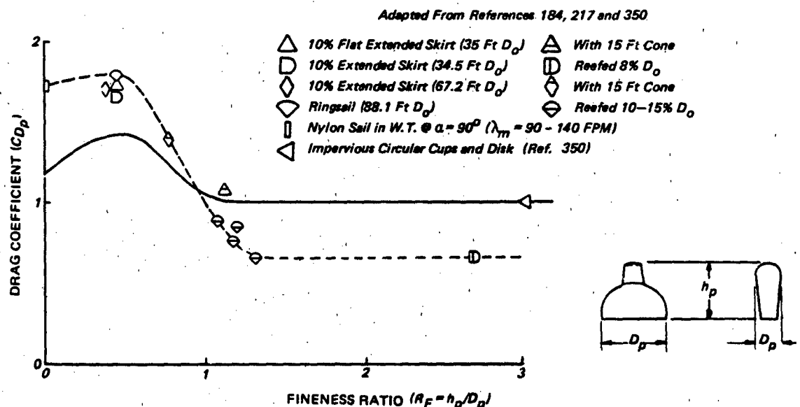
Figure 6.62 Effect of Canopy Fineness Ratio on Drag Coefficient
