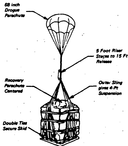
Figure 1.24 High Altitude Airdrop Resupply System (HAARS), First Stage Configuration
