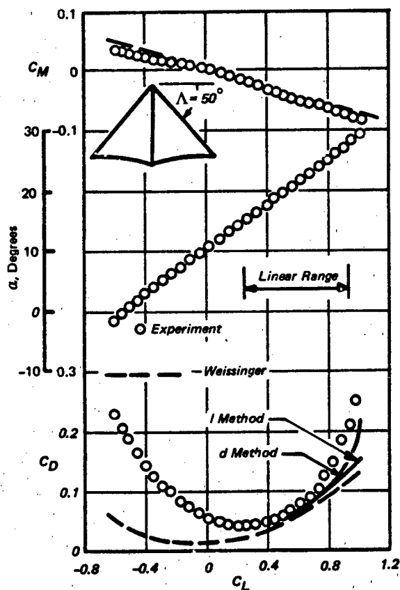
a) Characteristics of a Rigid Wing with A = 3 and 2\beta = 102.9^\circ .
