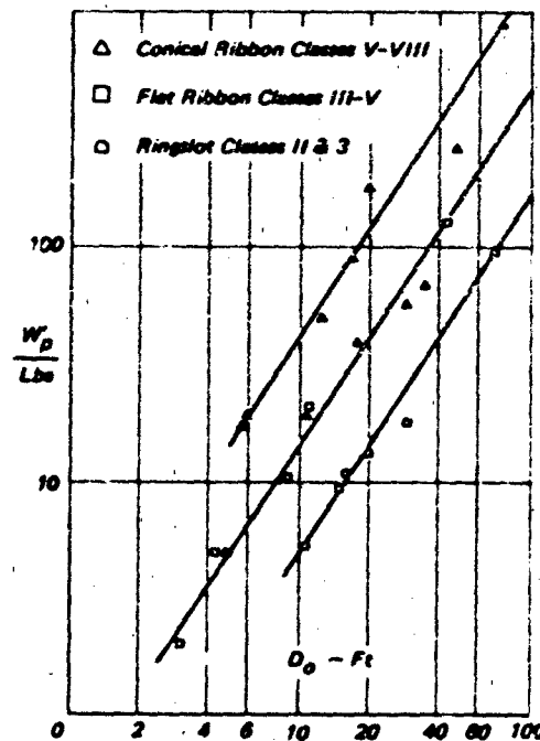
Figure 8.14. Parachute Weight vs D_0 and Construction Class
