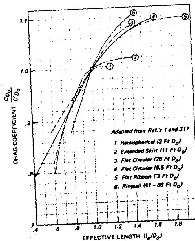
Figure 6.61 Effect of Suspension Line Effective Length on Parachute Drag Coefficient
