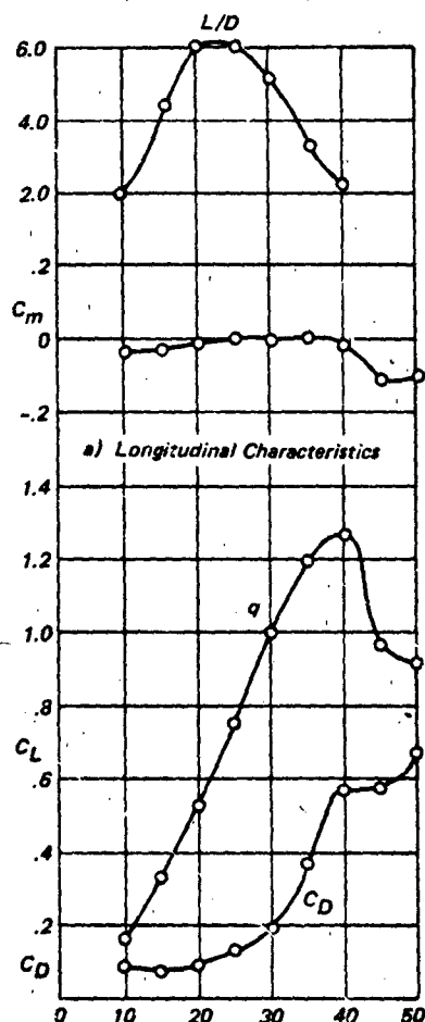
Figure 7.46 Summary of Aerodynamics of Sonic Rigid Model Single Keel Parawing (Ref. 545)
