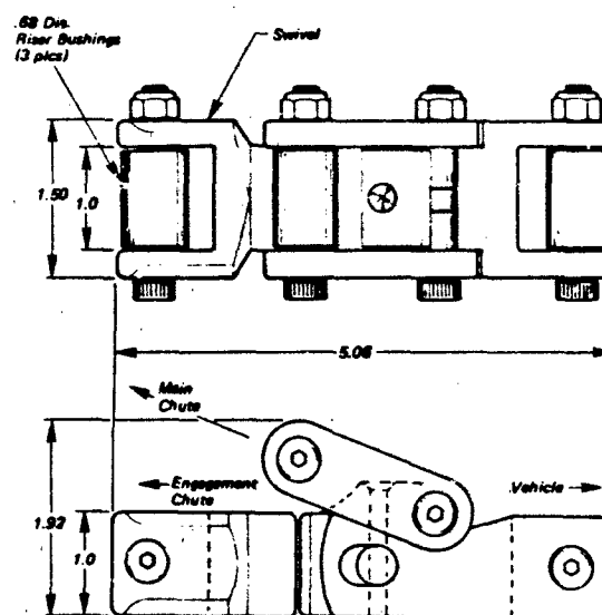
Figure 3.15 Miniature MARS Release
