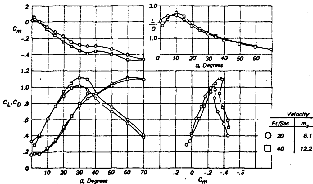
Figure 6.76 Longitudinal Aerodynamic Characteristics of Parafoil Designs II and III
