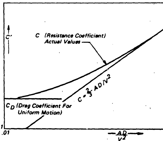
Figure 7.10 Resistance Coefficient vs Dimensionless Acceleration Parameter AD/V^2
