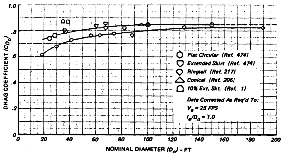
Figure 6.63 Variation of Parachute Drag Coefficient With Scale
