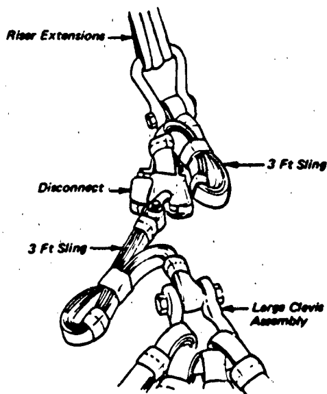
Figure 3.43 Typical Riser Assembly Using Clevis Links
