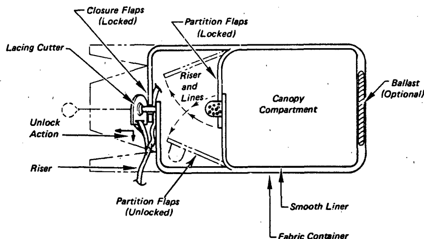
A) Integral Mortar Bag Pack
