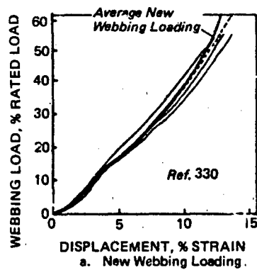
Figure 6.4A Relative Load-Flongation of Nylon Webbing from Twice Repeated Static Tests
