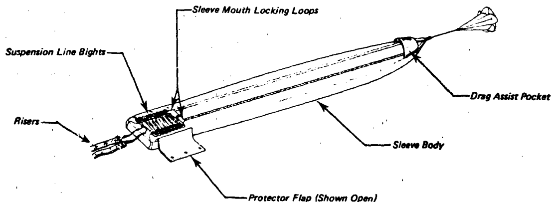
Figure 3.35 Deployment Sleeve
