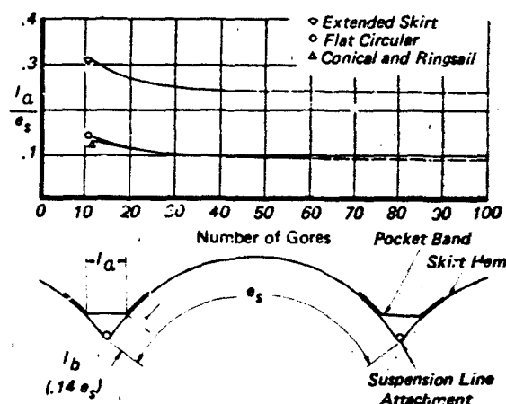
Figure 8.2 Pocket Band Dimensions for Circular Canopies
