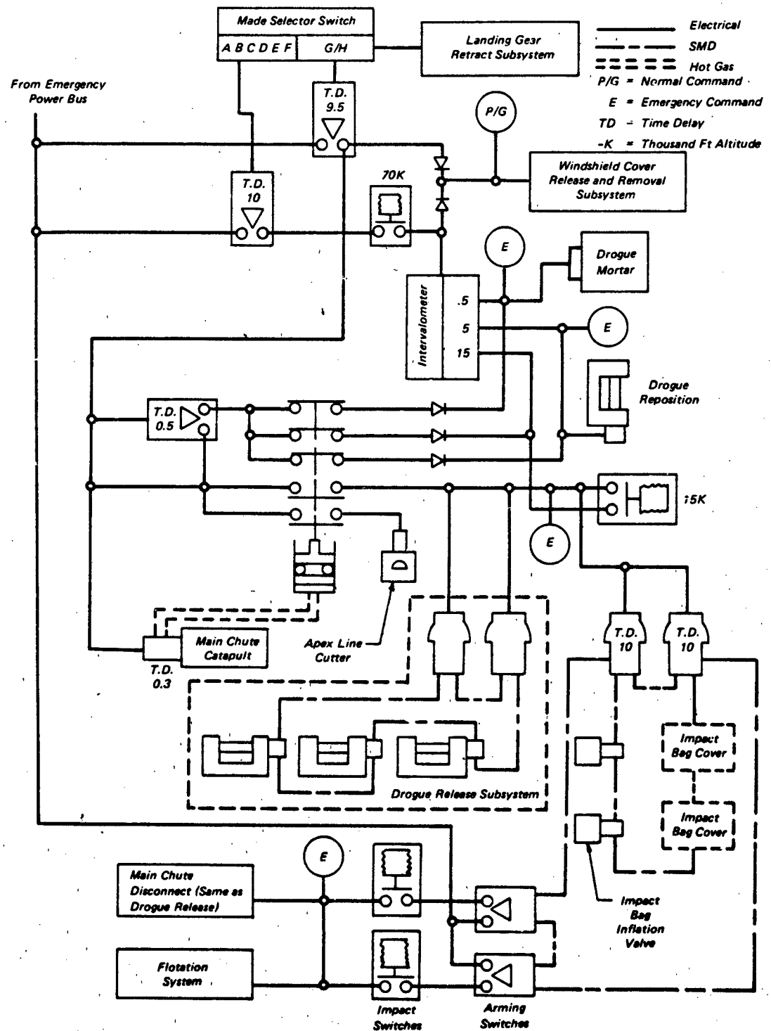
Figure 3.2 Control Subsystem Diagram for Emergency Recovery of Space Capsule
