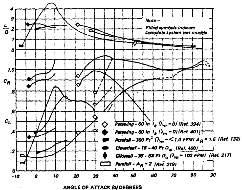
Figure 6.36A Variation of L/D and Aerodynamic Coefficients With Angle of Attack
