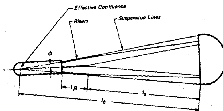
Figure 6.60 Effective Rigging Length With Multiple Riser Attachments
