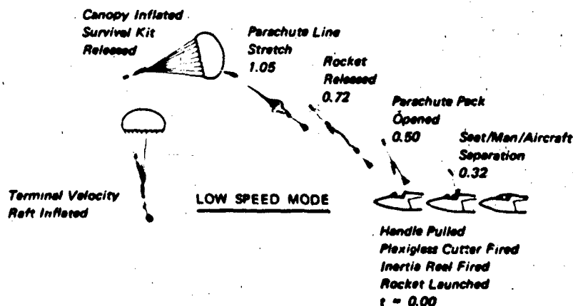
Figure 1.17 Tractor Rocket Escape System Operation
