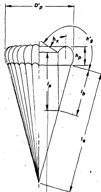
INFLATED PROFILE
