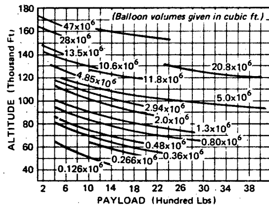
Figure 5.4 Generalized Carrier Balloon Performance Chart
