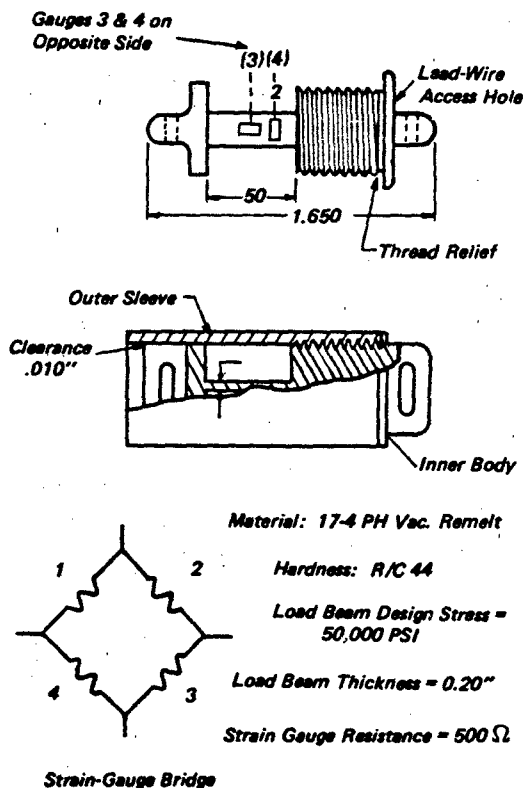
Figure 5.33 Typical Electric Strain-Gauge Force Transducer
