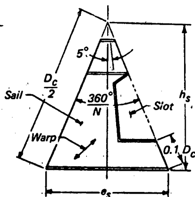
GORE LAYOUT
