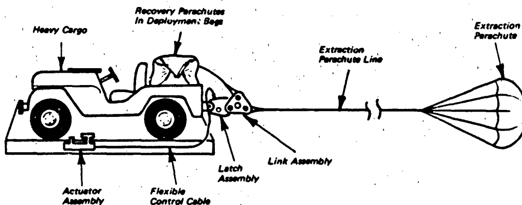
Figure 3.16 Extraction Force Transfer Coupling System (High Capacity)
