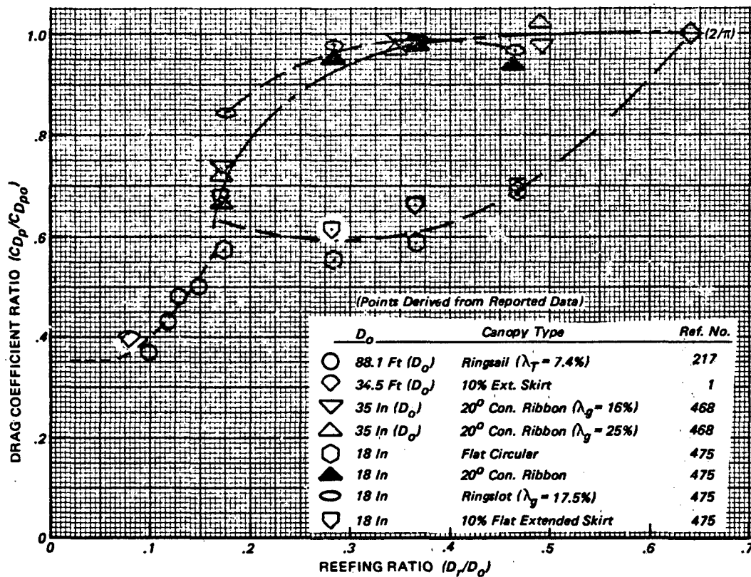
Figure 6.65 Variation of C_{Dp} With Reefing Ratio
