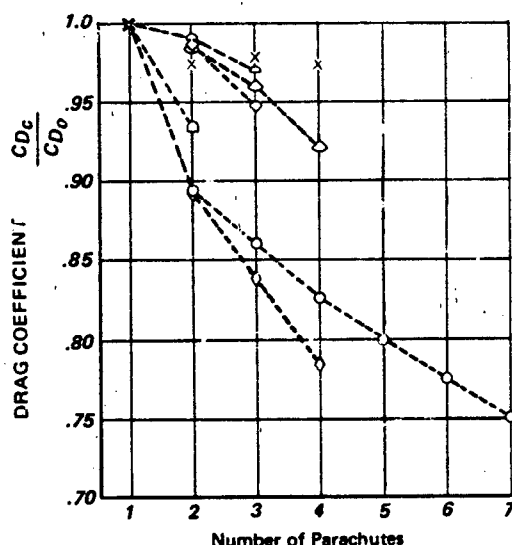
Figure 6.30 Effect of Clustering on Drag Coefficient
