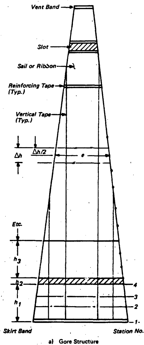
a) Gore Structure
