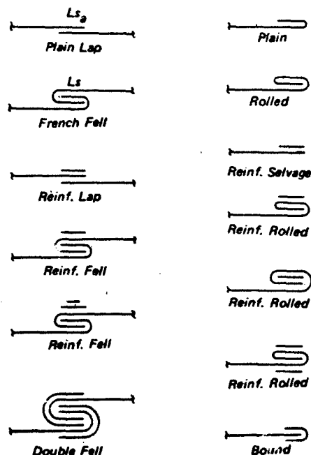
Figure 4.16 Typical Flat Fabric Seams and Hems
