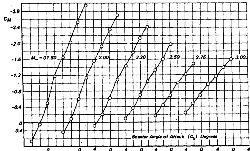
b) Variation of Pitching Moment Coefficient with \alpha_0 at Different Mach Numbers
