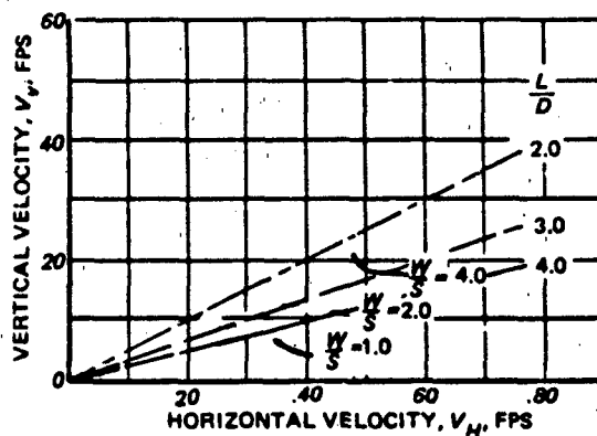
c) Glide Velocities for an Advanced Twin-Keel Parawing Having 15° Canted Keels
