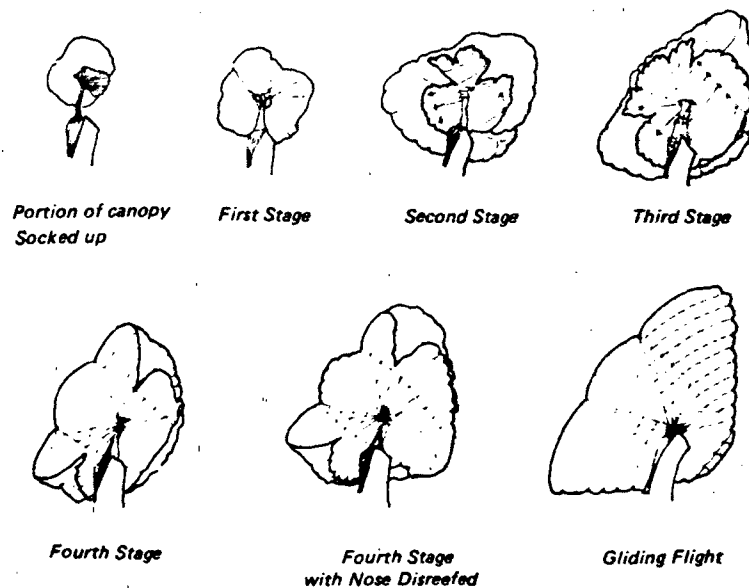
Figure 8.7 Twin-keel Parawing Inflation with Suspension Line Reefing in Four Steps.
