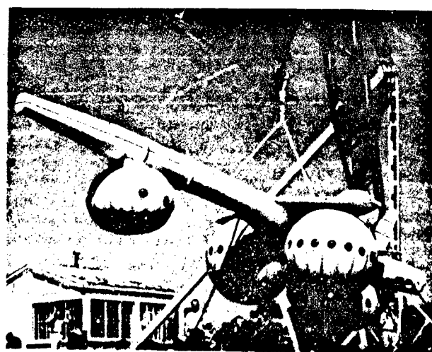
Figure 6.96 Airbag System Vertical Drop Test
