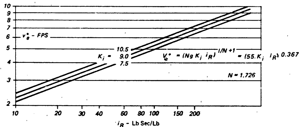
Figure 7.51 Variation of Optimum Design Rate of Descent with Effective Specific Impulse of Landing Retrorocket
