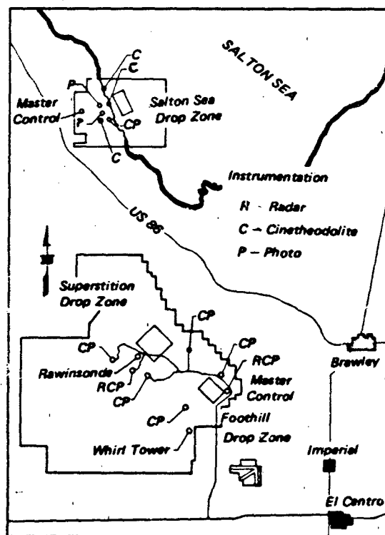
Figure 5.21 National Parachute Test Range, California
