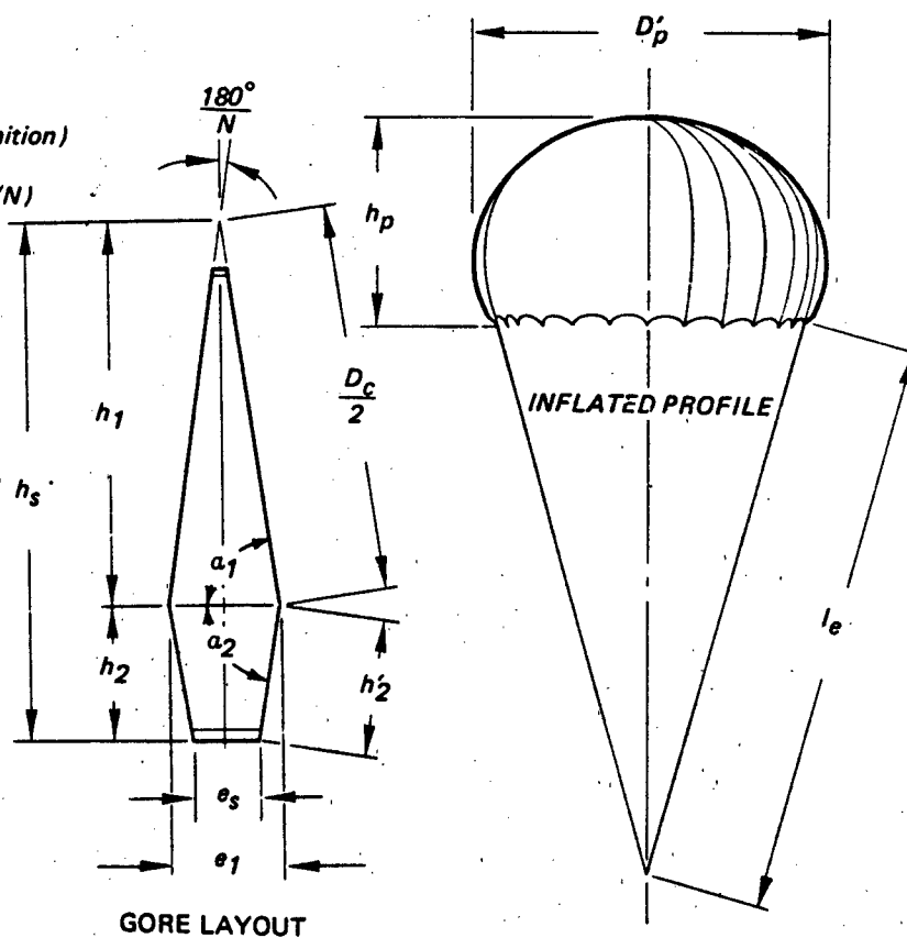
CONSTRUCTION SCHEMATIC
