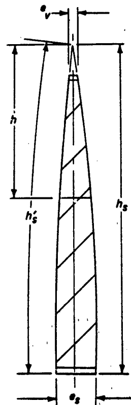
GORE LAYOUT
