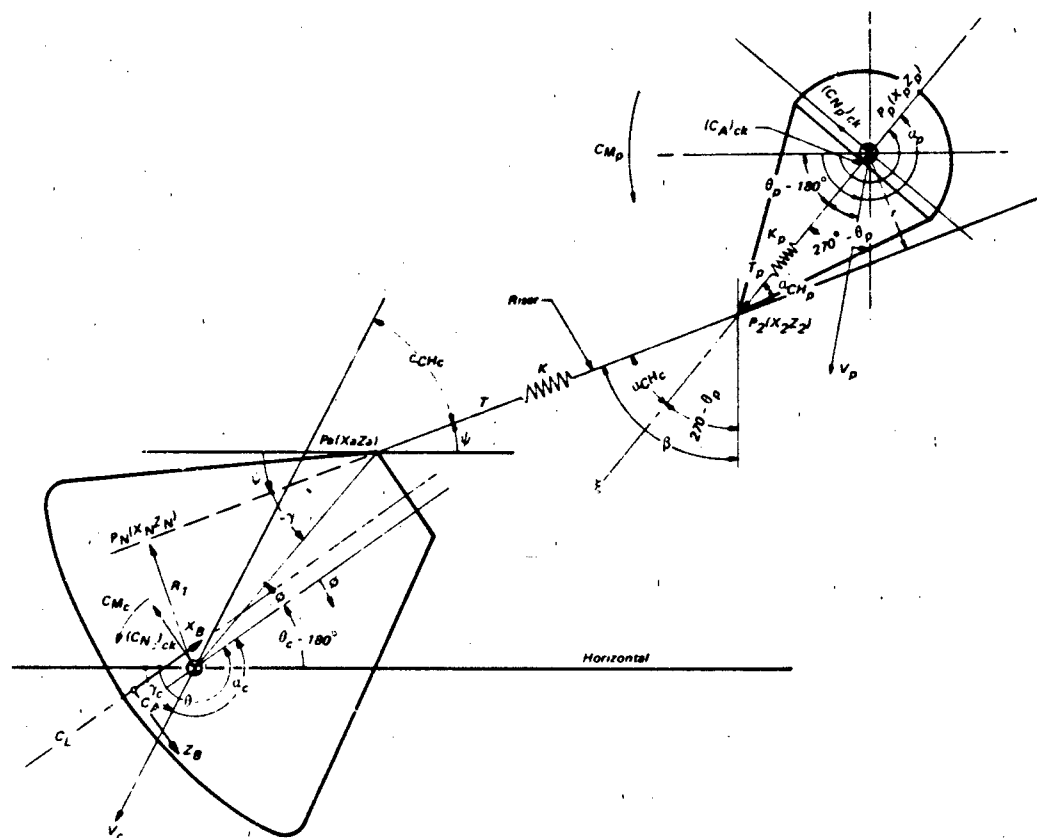
Figure 7.2 Schematic Geometry of Vehicle and Parachute
