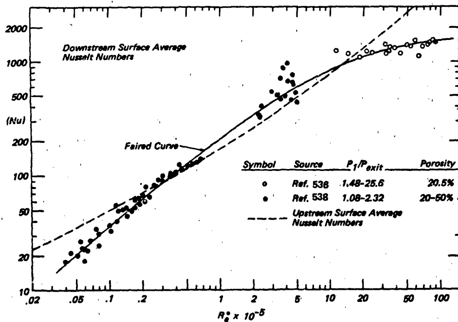
Figure 7.26 Comparison of Upstream and Downstream Experimental Heat Transfer Results
