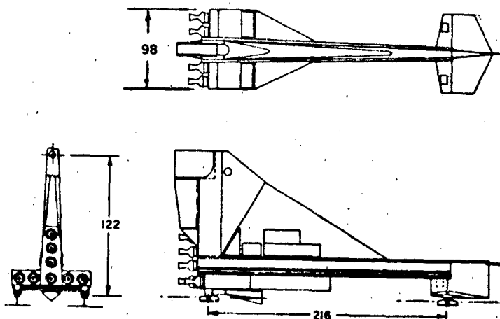
Figure 5.28 The Tomahawk Sled
