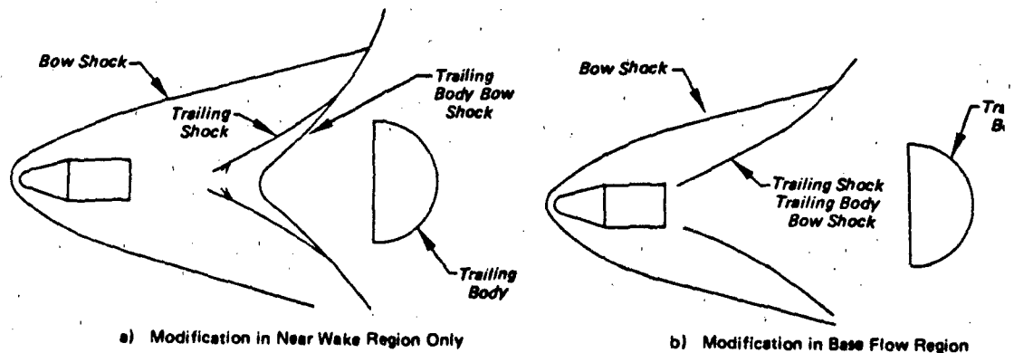
Figure 6.50 Types of Leading Body-Trailing Body Flow Field Interactions
