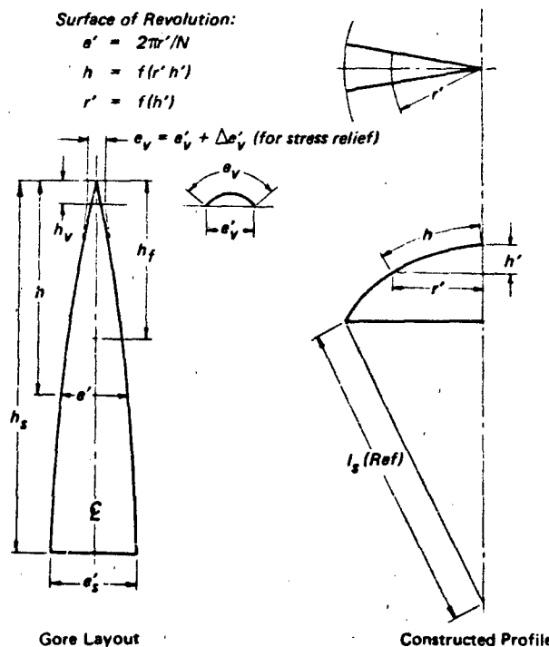
Figure 8.4 The Development of Gore Coordinates for Circular Canopy of General Profile
