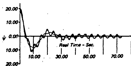
a) Main Parachute - SRB Response to a 20-Deg Pendulum Disturbance (X-SRB, 2-Sec Intervals)
