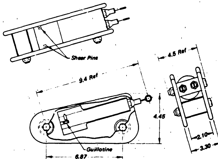
Figure 3.23 Cartridge Actuated In Line Strap Cutter
