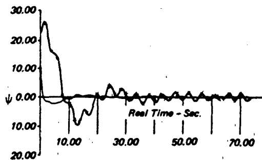
b) Main Parachute - SRB Angle of Attack Response to a 20-Deg Pendulum Disturbance (X-SRB, 2-Sec Intervals)
