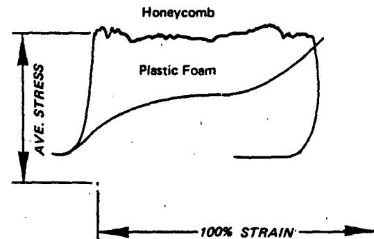
Figure 4.8 Stress-Strain of Crushable Structures
