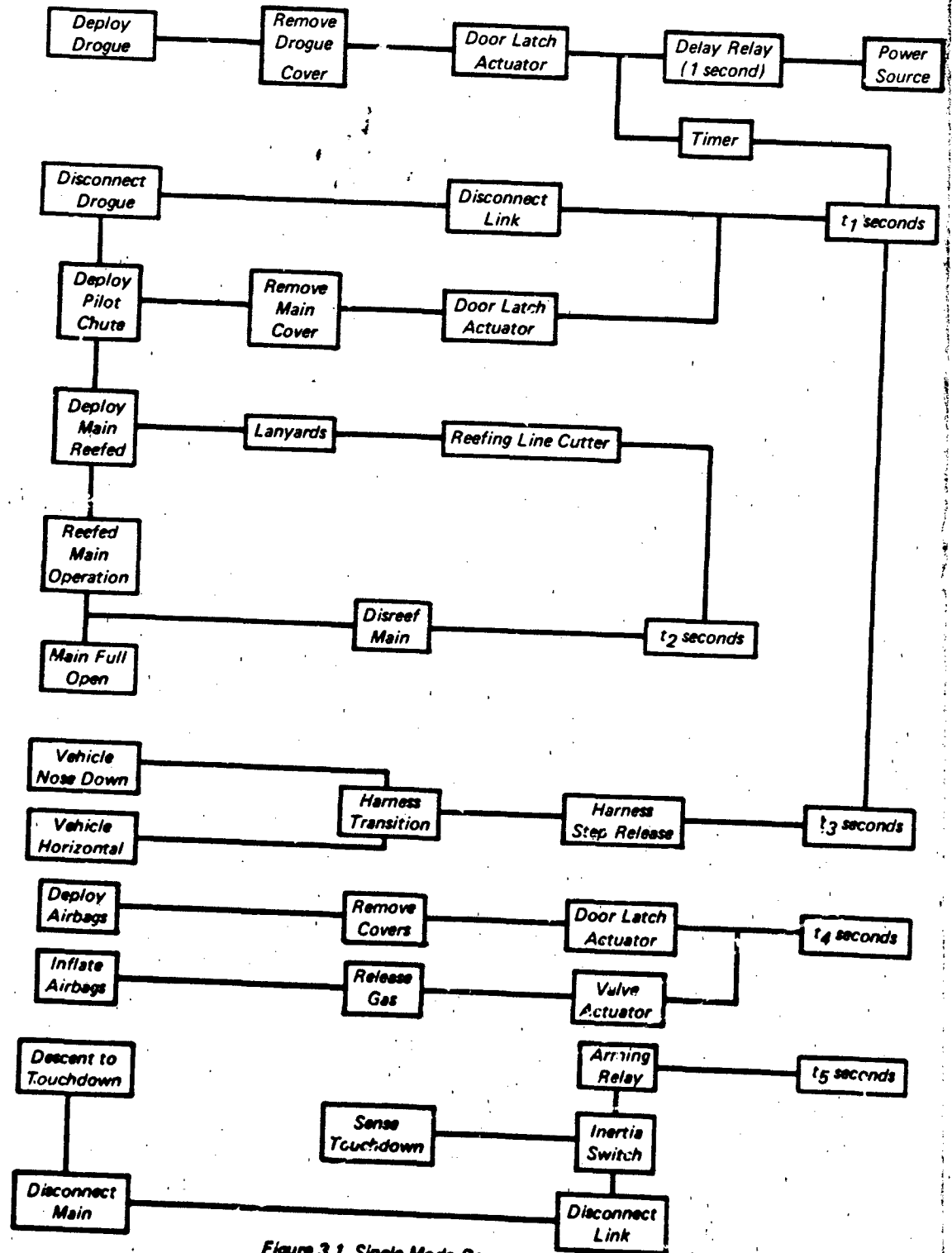
Figure 3.1 Single Mode Recovery Sequence
