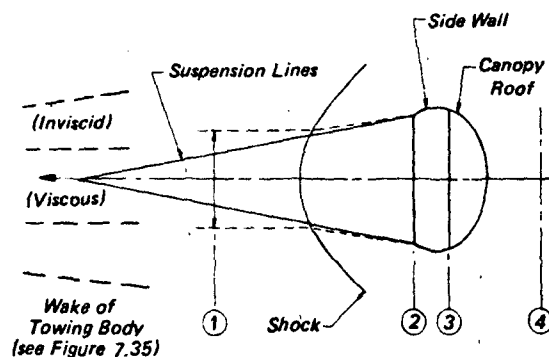
Figure 7.23 Flow Field of Supersonic Drogue for Dynamic Heating Analysis
