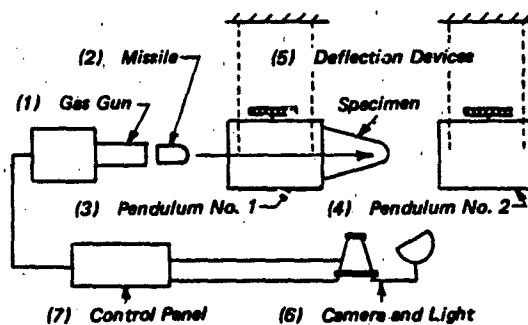
Figure 5.11 Schematic Diagram of Textile Impact-Testing Apparatus (Ref 326)
