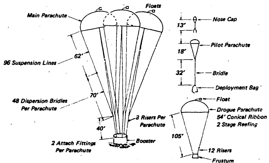
Figure 1.13 Solid Rocket Booster Recovery System
