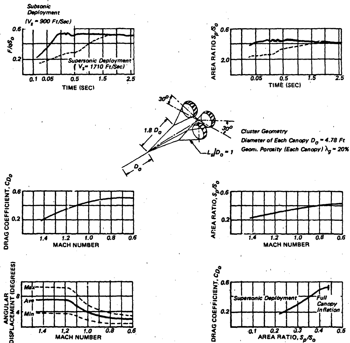
Figure 6.32 Performance Characteristics of Three Flat Circular Ribbon Drogues in Cluster Configuration (Ref. 376)
