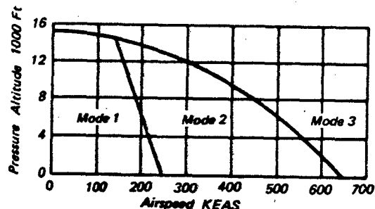
Figure 1.14 ACES II Operation Mode Zones
