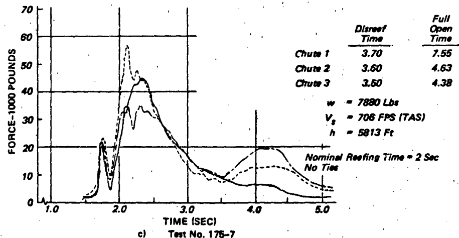
Figure 6.26 Opening Forces of 48 Ft ( D_0 ) Ribbon Parachute in Clusters of Three with Canopies Tied Together at Skirt Tangency Points (Ref. 386)
