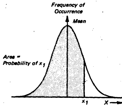
Figure 7.54 The Normal Distribution
