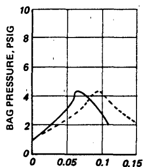
b) Typical Bag Pressure and Vertical Deceleration Transients
