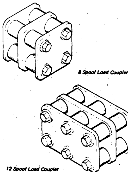
Figure 3.44 Cargo Parachute Load Couplers
