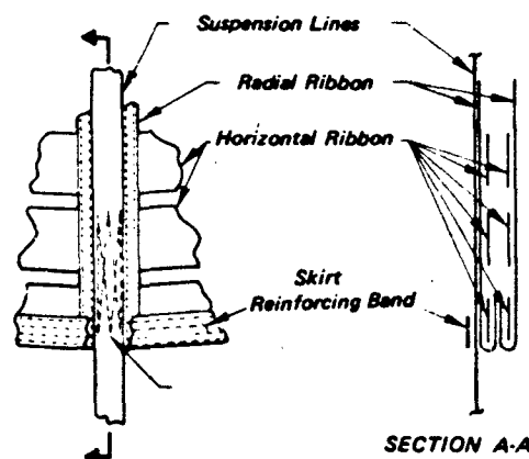
Figure 4.23 Continuous Radial/Suspension Line
