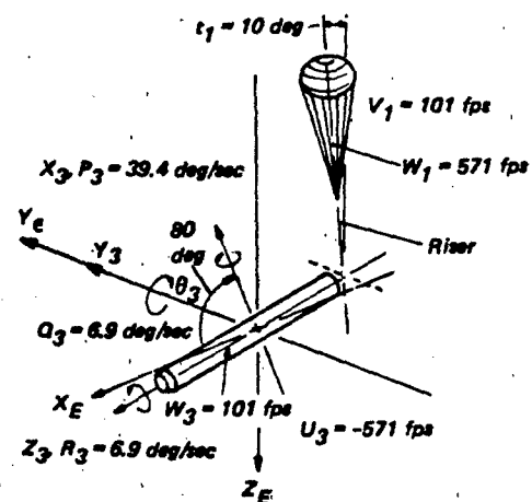
Figure 7.43 Drogue Effect Initial Conditions
