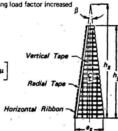
GORE LAYOUT
