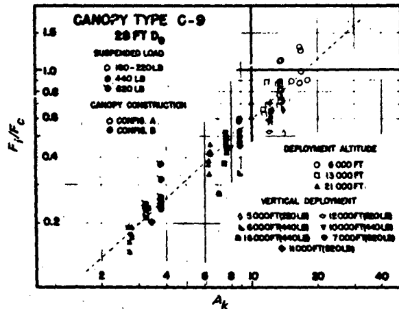
a) Variation of Peak Force Ratio With Parameter A_k
