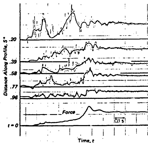
Figure 6.88B Canopy Stress and Total Force Measured on a 32 Gore Ringslot Model Parachute
