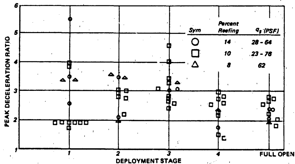
Figure 6.66 Measured Peak g 's vs Opening Stage of 4000 Ft 2 ( S_W ) Twin Keel Parawing
