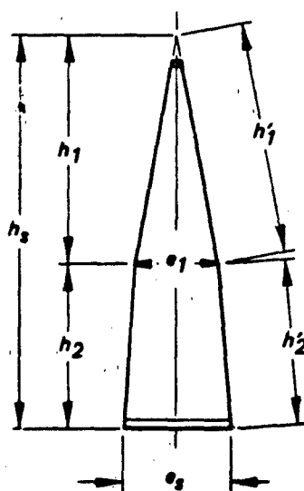
GORE LAYOUT
