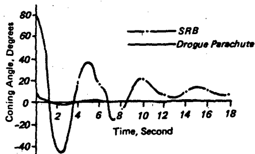
b) SRB Coning Angle as Reduced by the Action of the Drogue Parachute
