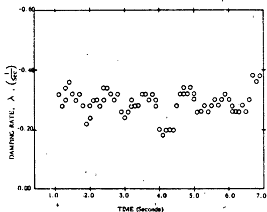
a) Variation of Damping Rate with Time (Test No. 7)
