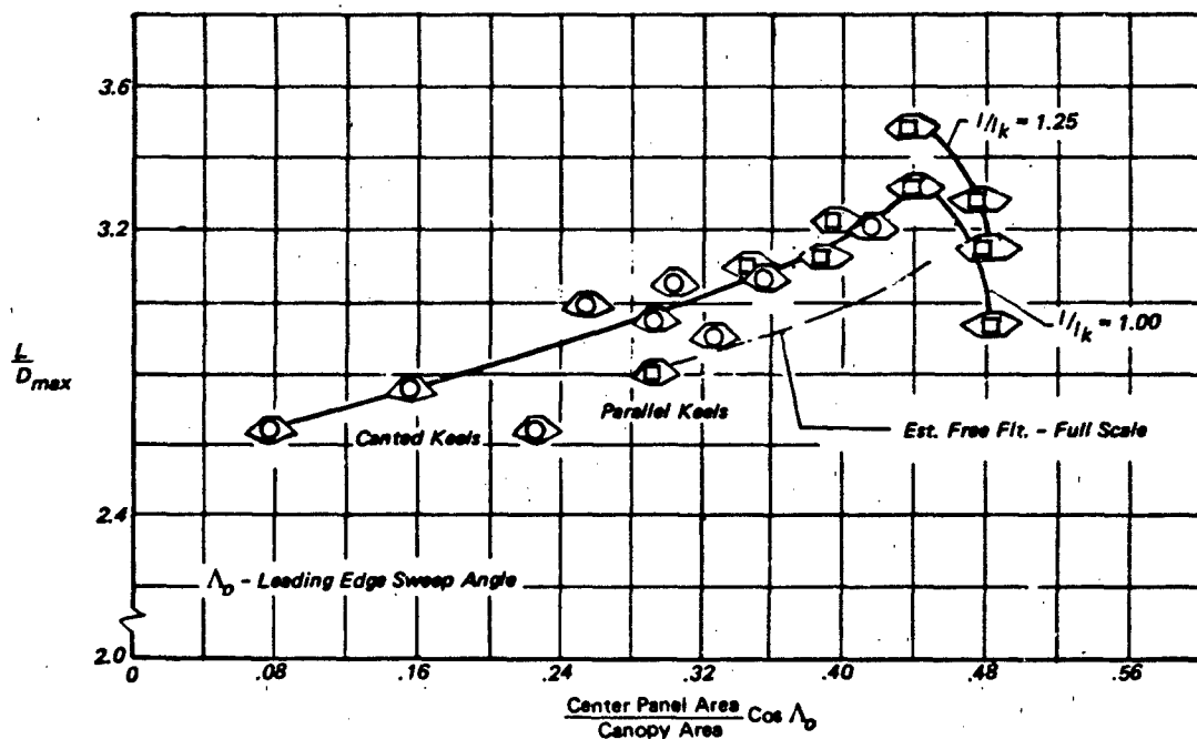
a) Performance Summary of Twin-Keel Parawings Having a Formed Nose
