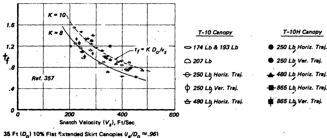
Figure 6.15 Measured Filling Time Vs Snatch Velocity of Solid Cloth Circular Parachute (Non-Reefed)
