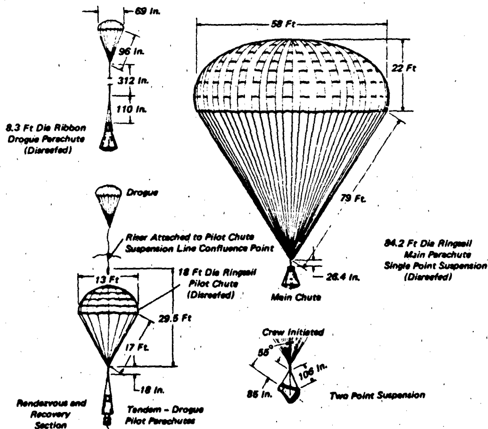
Figure 1.7 Gemini Parachute System
