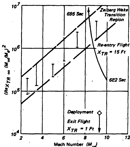
Figure 7.30 Unified Wake Transition Criterion for Ballute Flight Test TB-4 (Ref. 215)
