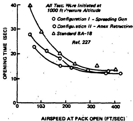
Figure 6.13 Effect of Skirt Spreading Gun and Canopy Apex Retraction on the Opening Time of Personnel Parachutes
