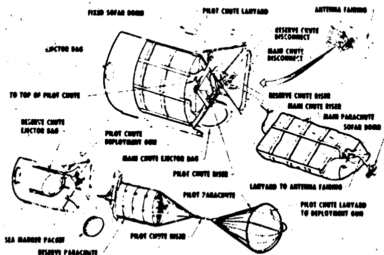
Figure 1.6 Mercury Recovery System Installation
