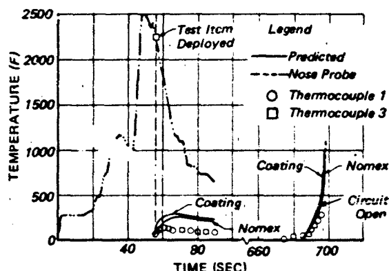
Figure 6.92 Aerodynamic Heating of a Nomex Ballute Flight Test TB-4
