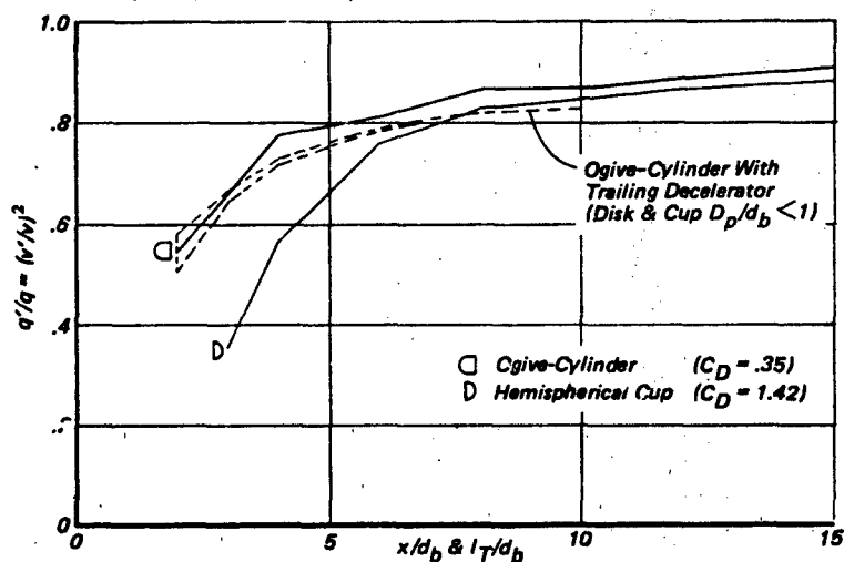
Figure 6.45 Impact Pressure Ratio on Wake Centerline Ogive-Cylinder & Hemispherical Cup (Adapted from Ref. 382)
