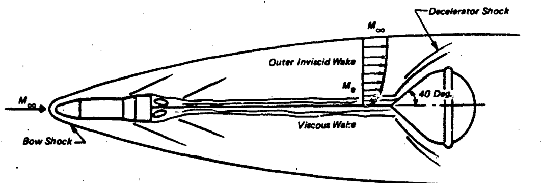
Figure 7.31 Vehicle-Ballute Flow Field Schematic
