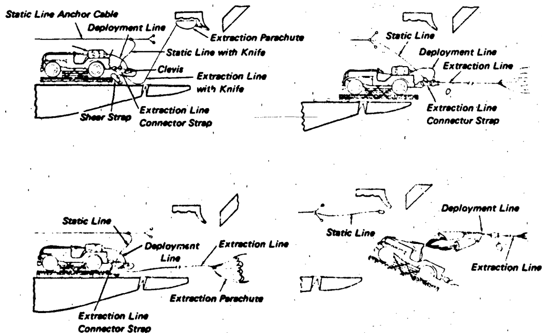
Figure 3.37 Typical Extraction and Force Transfer Sequence
