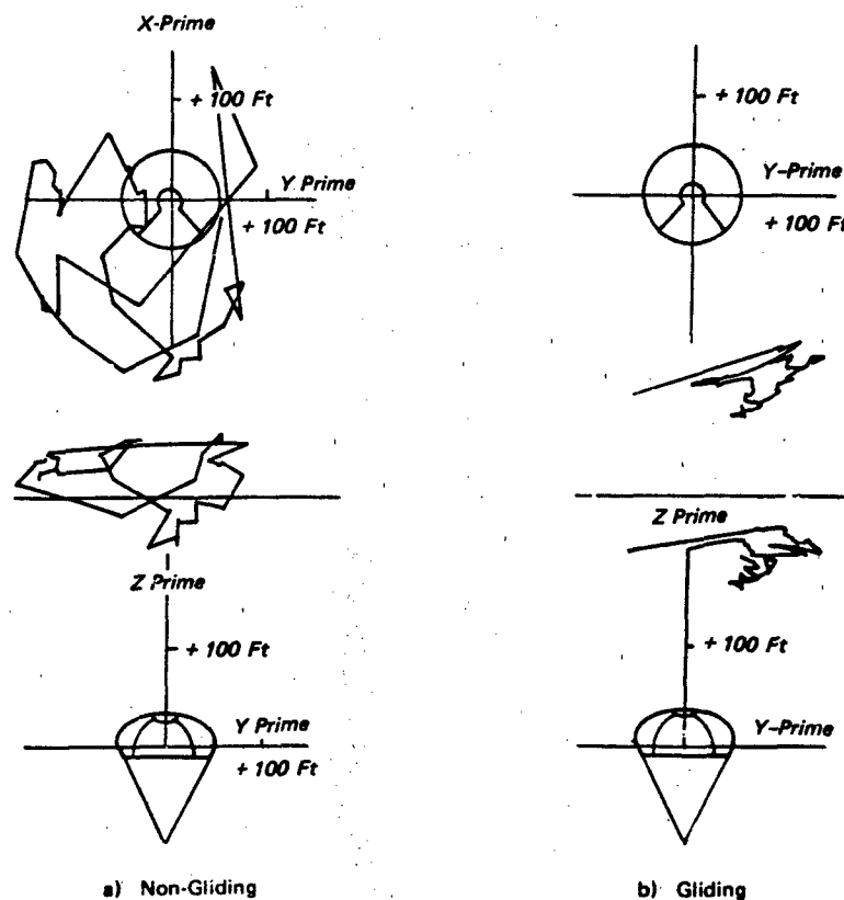
Figure 6.79 Effect of Gliding on Position Stability of MARS-H Engagement Canopy
