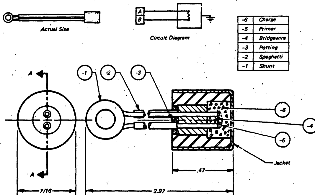
Figure 3.3 Typical Cartridge Configuration
