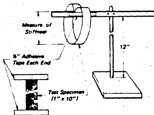
Figure 5.18 The Hanging Loop Method of Measuring the Relative Stiffness of Thin Flexible Materials
