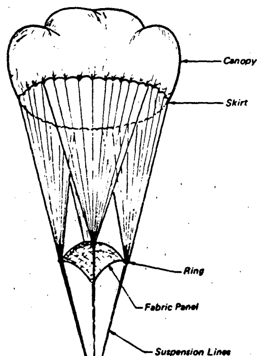
Figure 8.8 Continuous Suspension Line Reefing by Sliding Rings with Drag-Panel
