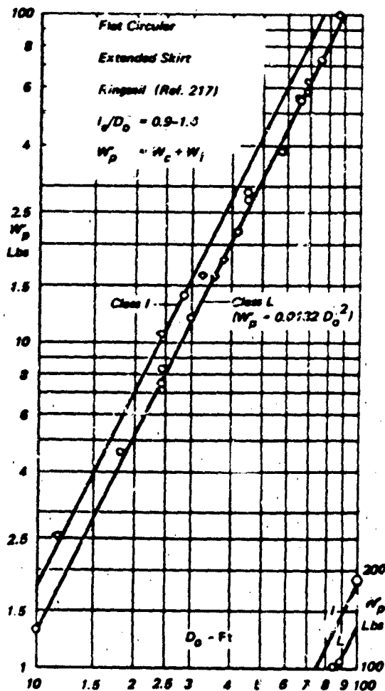
Figure 8.13. Parachute Weight vs D_0 Typical for Classes L and I
