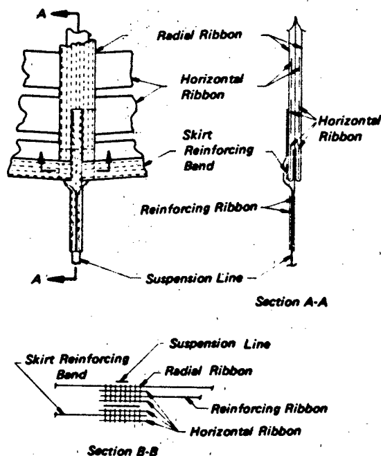
Figure 4.20 Webbing Type Line Attachment
