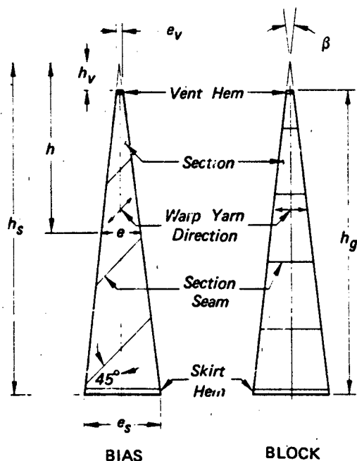
Figure 2.2 Flat Patterns of a Gore
