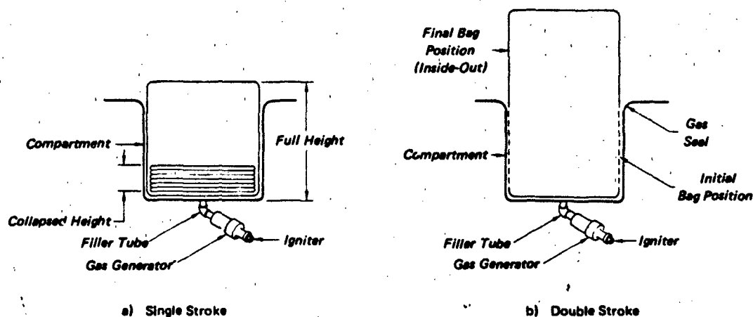
Figure 3.6 Ejector Bags
