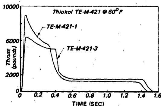
Figure 6.99 Thrust vs Time for TE-M-421-1 and TE-M-421-3 Rockets at 60°F (from Ref. 499)
