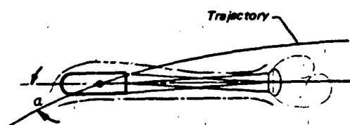
Figure 6.74 Schematic of Bomb Wake Downwash Due to Body-Lift (With Stabilization Para.)
