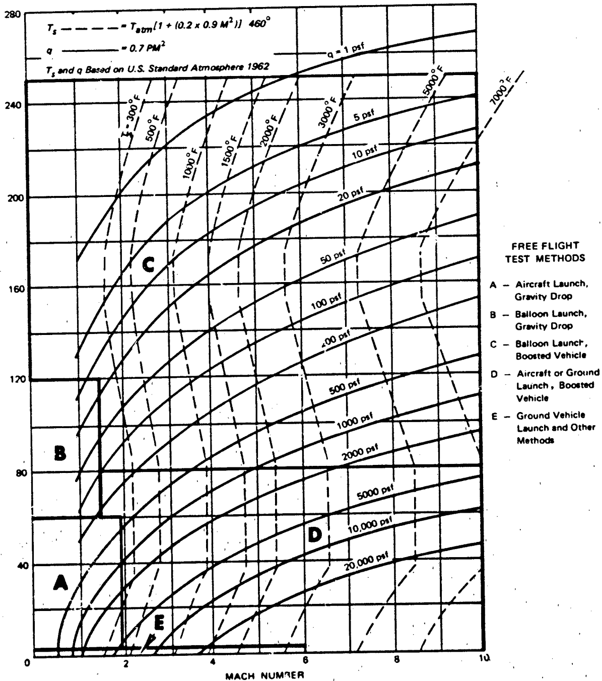
Figure 5.1 Altitude vs Mach Number, Decelerator Performance Regimes
