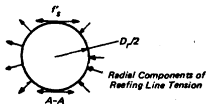
Figure 7.21 Relative Reefing Line Load
