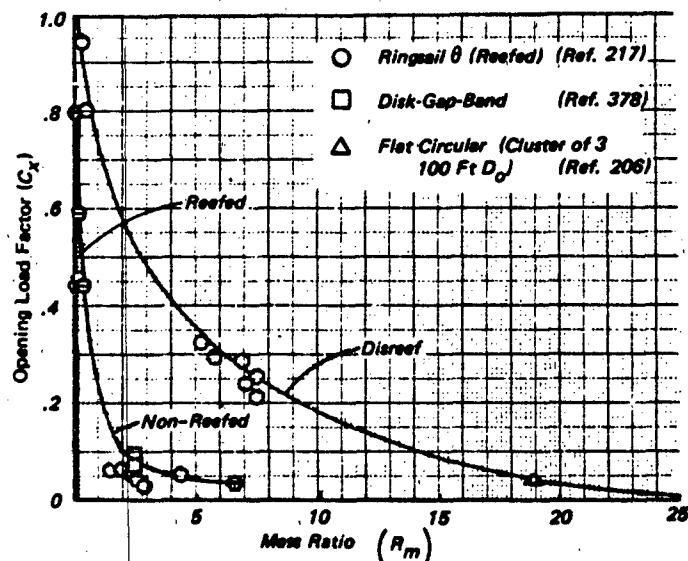
b) Selected Parachute C_x Avg. Disreef to Full and Non-Reefed
