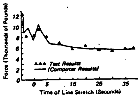
e) Drogue Riser Vs Time. Computer and Test Results
