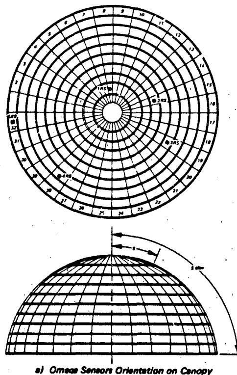
a) Omega Sensors Orientation on Canopy Figure 6.89 Measured Opening Forces and Canopy Stress of Model Ringslot Canopy
