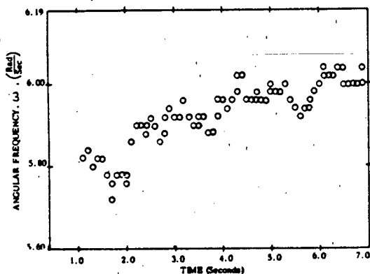
c) Variation of Angular Frequency with Time (Test No. 7)
