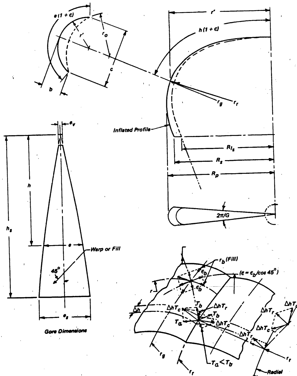
Figure 7.15 Stress-Strain Relationships in Circular Canopy of General Profile and Bias Construction
