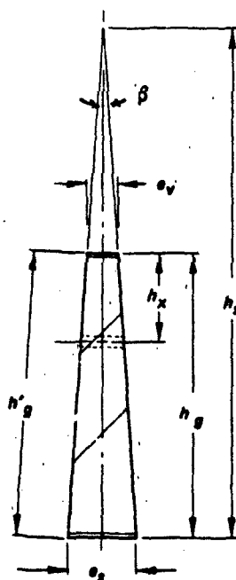
GORE LAYOUT
