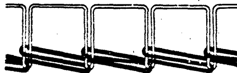
Figure 4.13 Stitch Type 401
