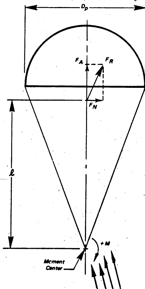
Figure 6.71 The System of Axes Used for Static Stability Considerations
