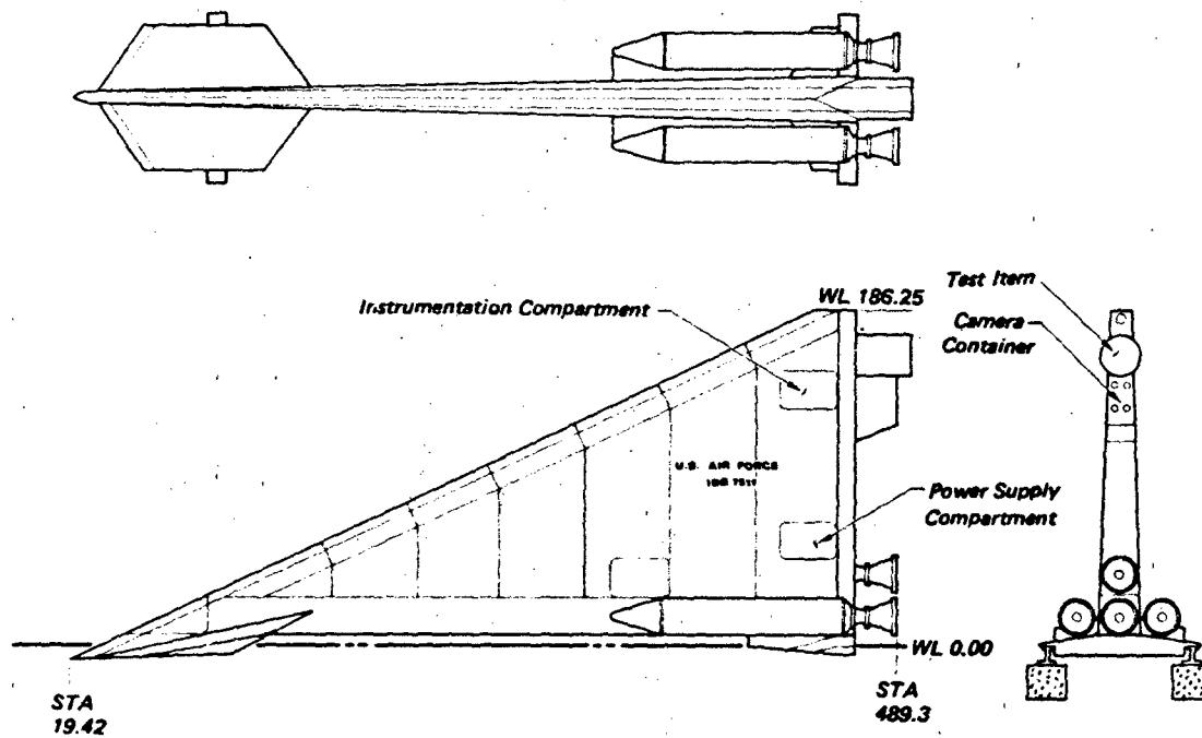
Figure 5.29 The Bushwhacker Sled
