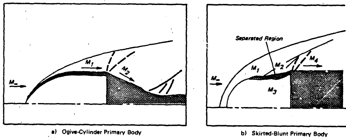
Figure 6.49 Sketch of Flow Patterns Around Primary Bodies Alone at Supersonic Speeds
