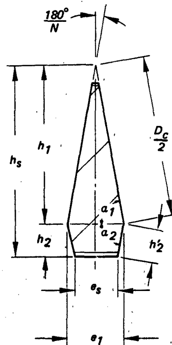
GORE LAYOUT
