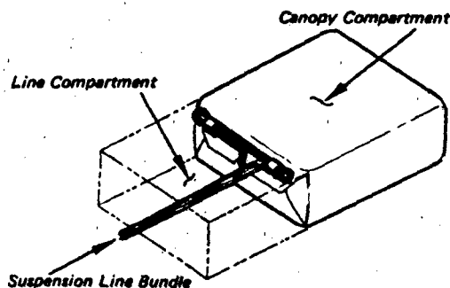
Figure 3.32 Line-Bight Locks Inside a Deployment Bag
