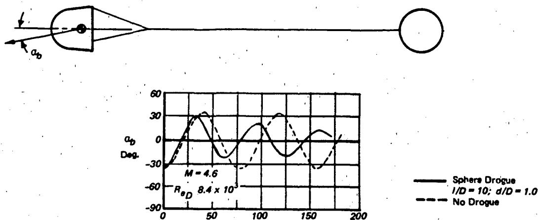
Figure 6.81 Effect of Sphere Drogue on Amplitude Decay of Entry-Body Angle of Attack (Ref. 440)
