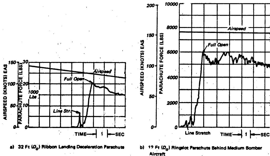
Figure 6.23 Typical Opening Forces of Aircraft Deceleration Parachutes (Ref. 382)
