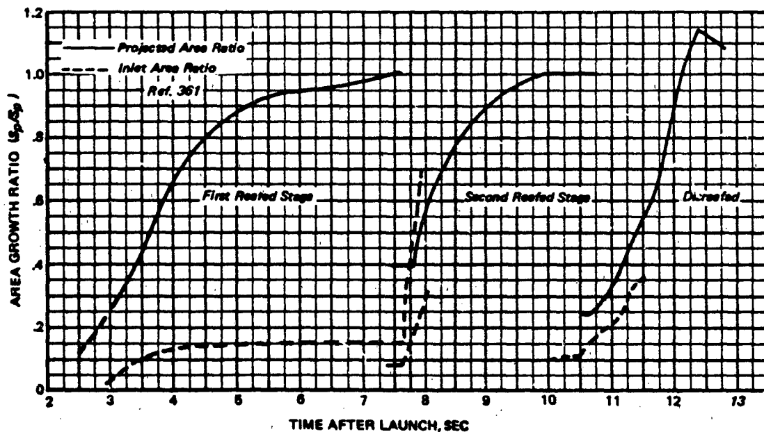
Figure 6.11 Measured Area Growth During Inflation of 85.6 Ft ( D_0 ) Modified Rinsall Parachute With Two Reefed Stages ( S_p' = Projected Area at End of Stage)
