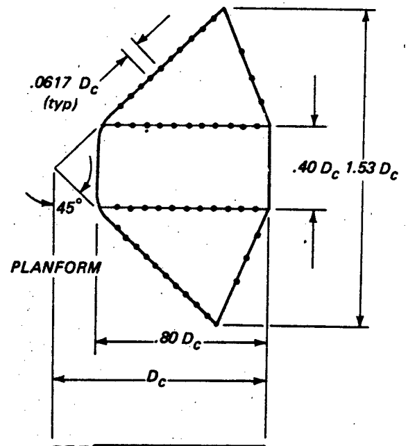
CONSTRUCTION SCHEMATIC
