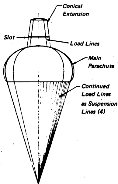
Figure 1.36 Extended Skirt Parachute With Conical Extension
