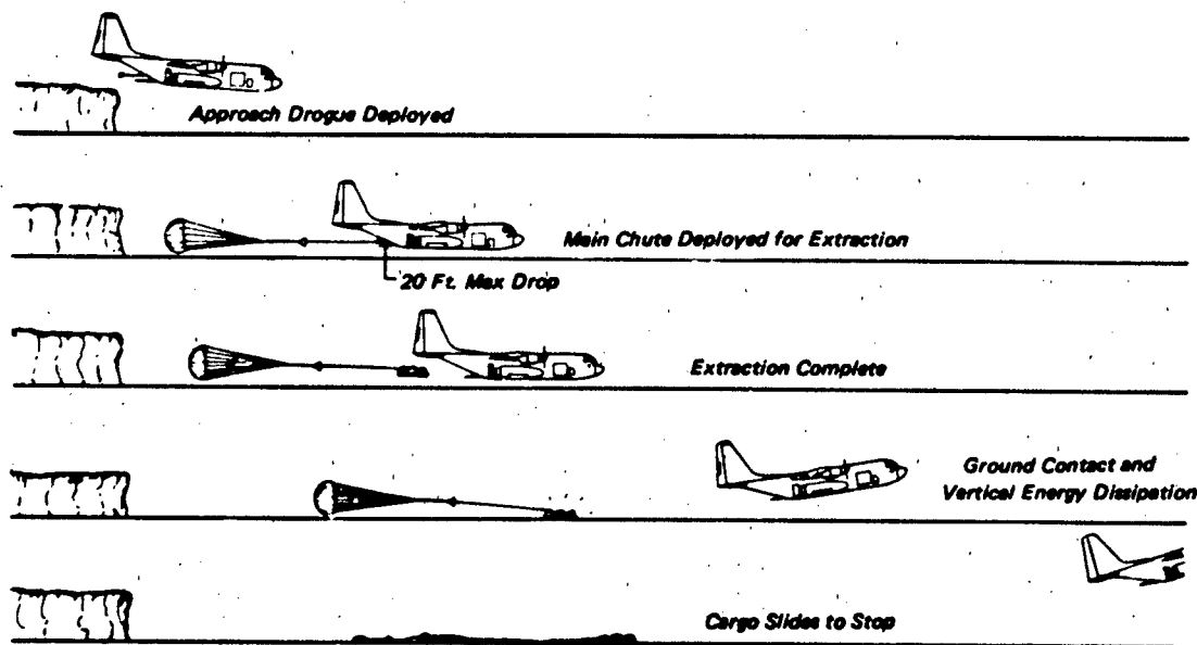
Figure 1.23 "LAPES" Airdrop System
