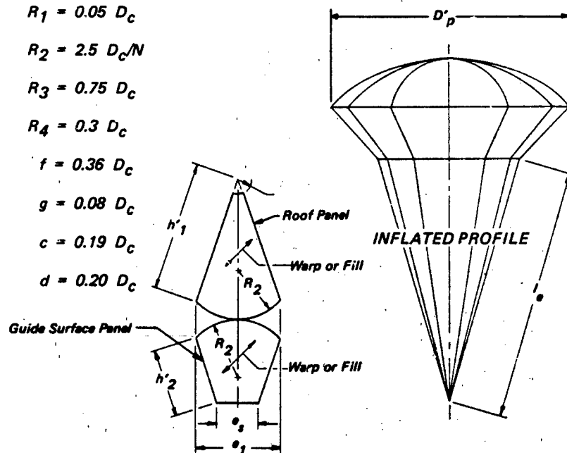
GORE LAYOUT
