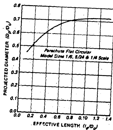
Figure 6.59 Variation of Canopy Projected Diameter With Effective Length of Suspension Lines in Small Models (Ref. 382)
