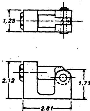
Figure 3.25 Single Initiator Parachute Release
