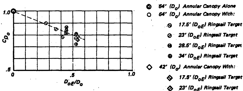
Figure 6.46 Drag Coefficient of Experimental Tandem Canopy Systems (Ref. 184)
