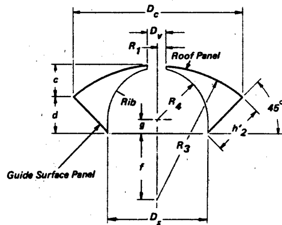
CONSTRUCTION SCHEMATIC
