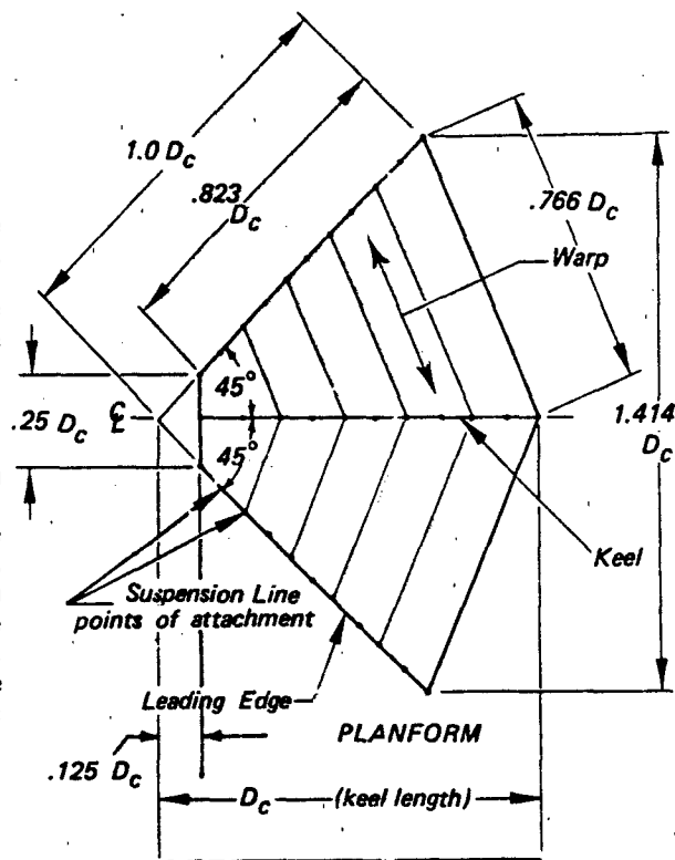
CONSTRUCTION SCHEMATIC
