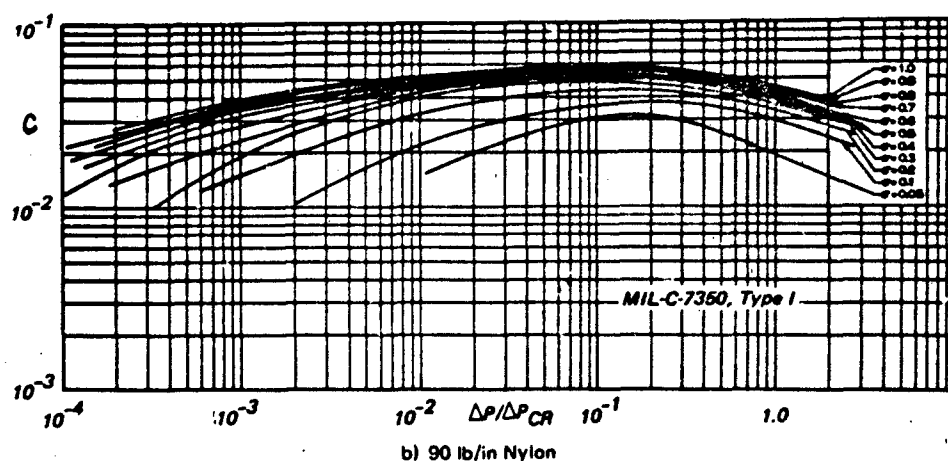
Figure 6.57 Effective Porosity versus Pressure Ratio for Various Nylon Cloth Materials
