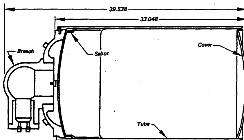
a) Mortar Assembly (Uses eroding orifice)
