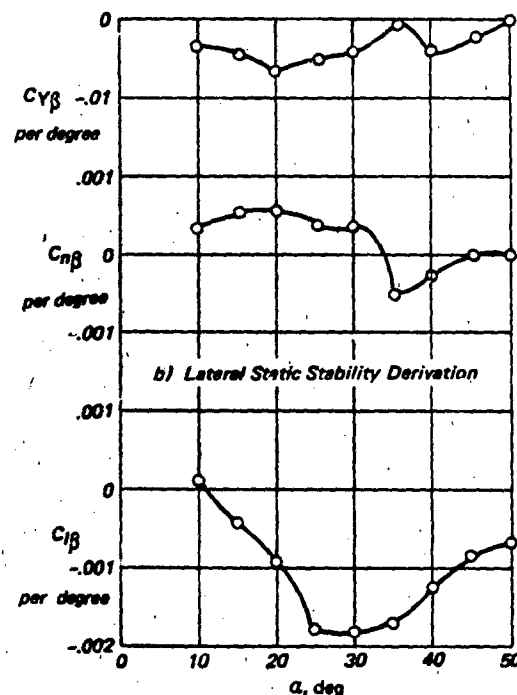
Figure 7.46 Summary of Aerodynamics of Sonic Rigid Model Single Keel Parawing (Ref. 545)
