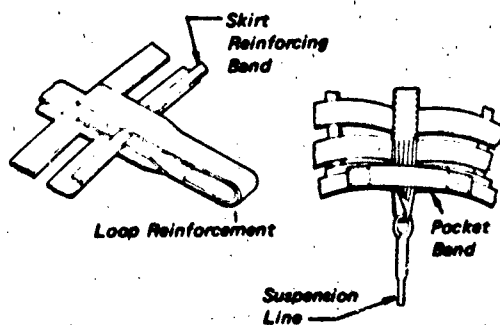
Figure 4.21 Suspension Line Connection to Skirt Loop Attachment
