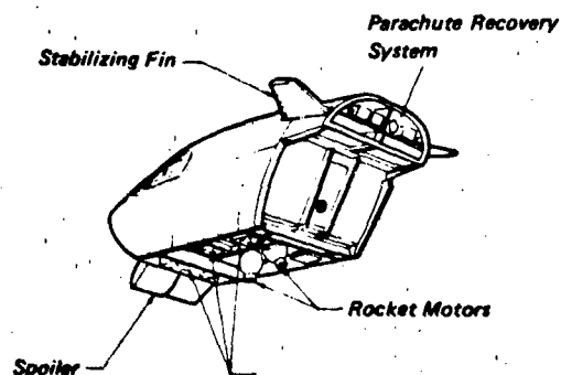
Figure 1.21 Aircraft Crew Module
