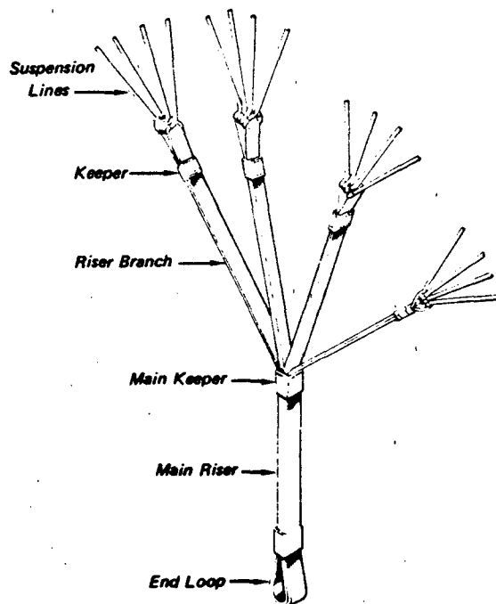
Figure 3.36 Typical Riser with Branches
