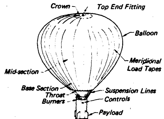
Figure 2.14 Paravulcoon System
