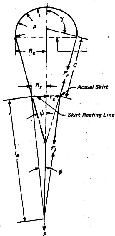
c) Inflated Profile - Reefed
