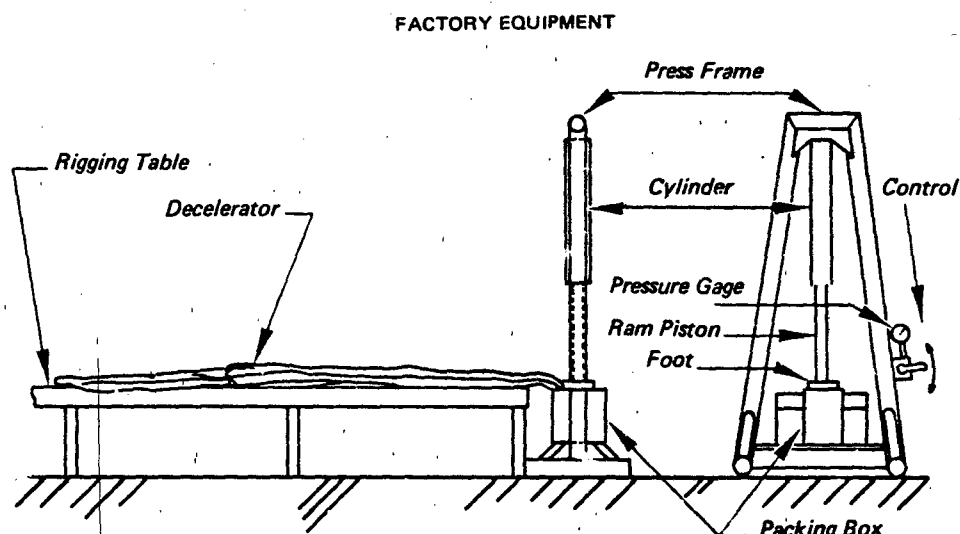
Figure 4.34 Schematic of General Utility Decelerator Packing Press Facility
