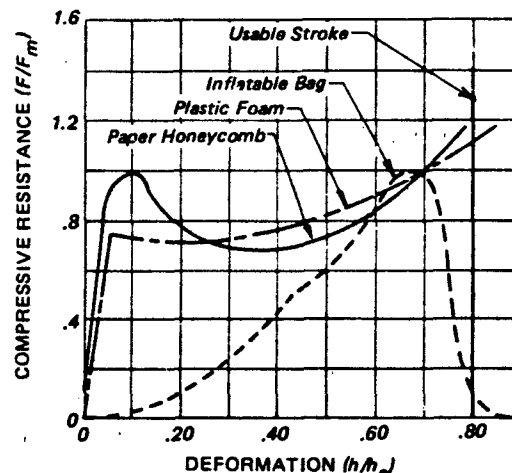
Figure 6.94 Variation of Compressive Resistance With Deformation of Energy Absorber (Ref. 382)
