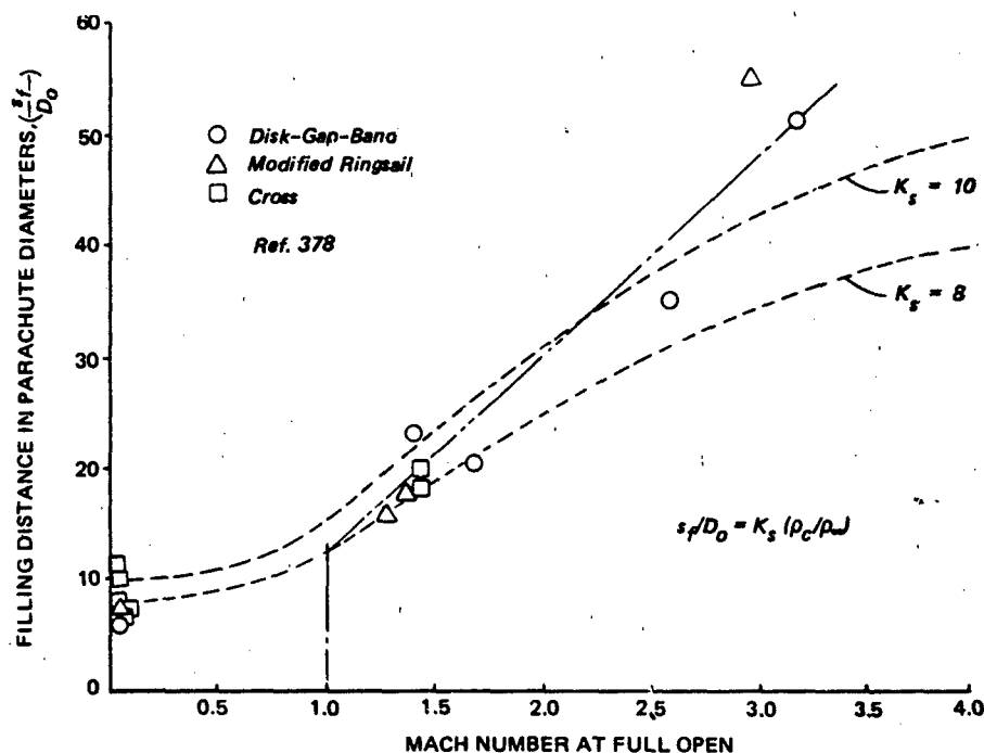
Figure 6.16 Effect of Compressibility on Filling Distance of Non-Reefed Parachutes
