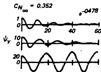
a) Computer Solutions for 1°, 10° and 20° Pitch Displacements of the Stable System
