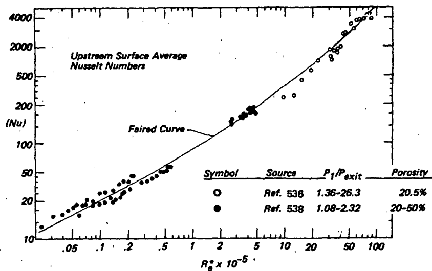
Figure 7.25 Experimental Heat Transfer Results (Upstream) for Parachute Ribbon Grids
