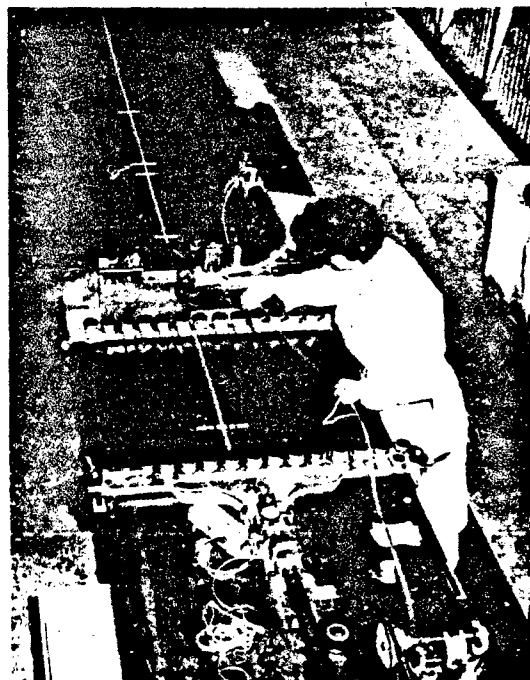
Figure 4.30 Suspension Line Tensioning and Marking Apparatus
