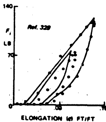
b) Measured Vs Computed Load-Elongation for Ten Impact Loading Cycles
