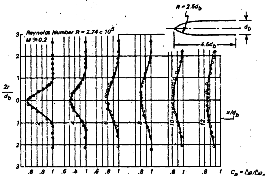
b) Pressure Distribution in the Wake of a Body of Revolution ( C_D = 0.35 ) (Ref. 423)
