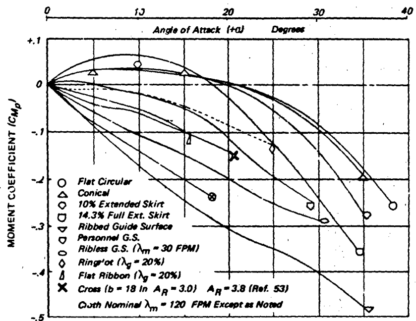
Figure 6.72 Measured Moment Coefficients vs Angle of Attack for Small Cloth Canopies in Wind Tunnel
