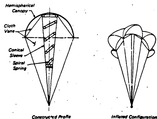
Figure 3.30 Vane Type Pilot Chute
