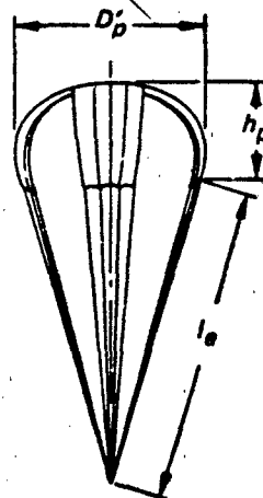
INFLATED PROFILE
