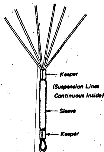
Figure 4.27 Integral Line Riser
