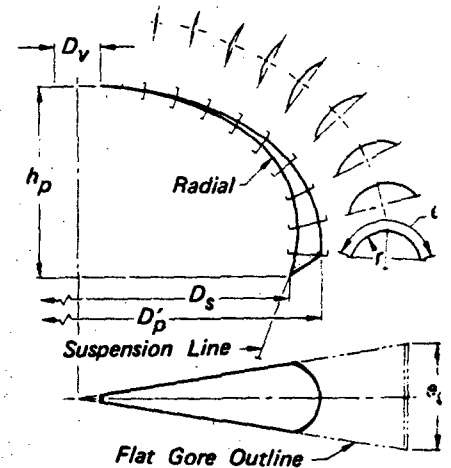
Figure 2.5 Shape of an Inflated Gore
