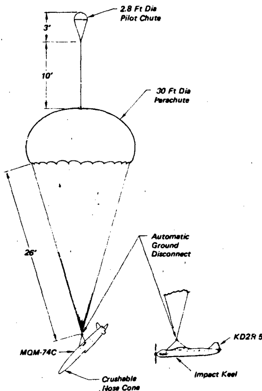
Figure 1.1 Recovery Configurations for MQM-74C and KD2R-5
