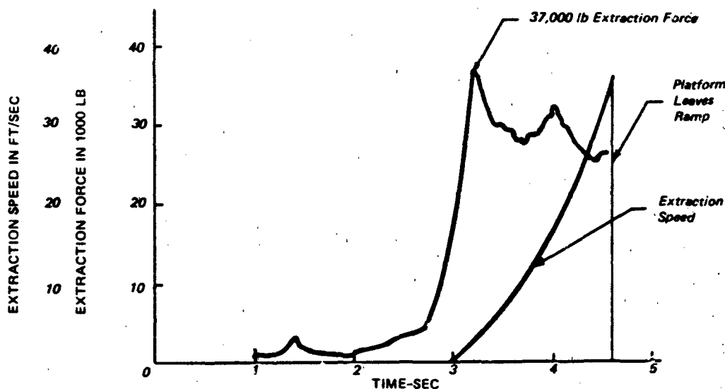
Figure 1.25 Parachute Extraction Force and Extraction Speed vs Time For a 35 Ft Parachute Extracting a 50,000 Lb Load
