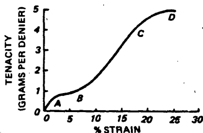
Figure 4.1 Stress vs Strain of a Polymeric Fiber
