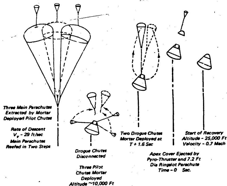
Figure 1.10 Apollo Recovery System Deployment For Normal Landing
