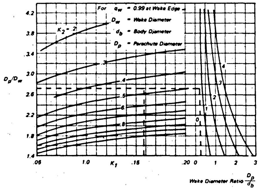
Figure 7.35 Diameter of Wake
