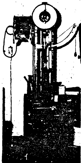
Figure 5.10. Representative Textile Testing Machine for Fabrics and Light Cordage
