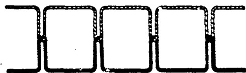
Figure 4.9 Stitch Type 301
