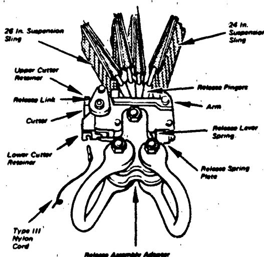
Figure 3.19 Multiple Release Assembly with Adapter, Slings, and Cutter Installed
