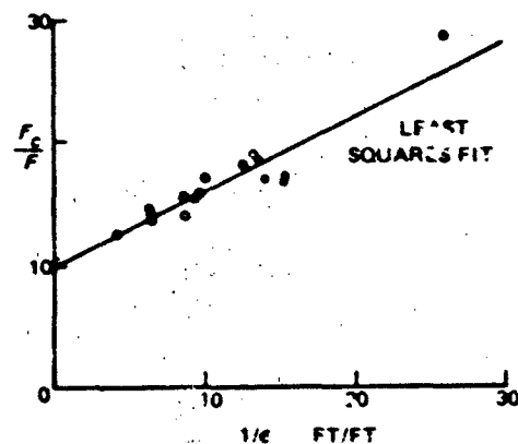
Figure 6.4C Ratio of Impact Peak Load to Static Load Versus Inverse Elongation ( 1/\epsilon )
