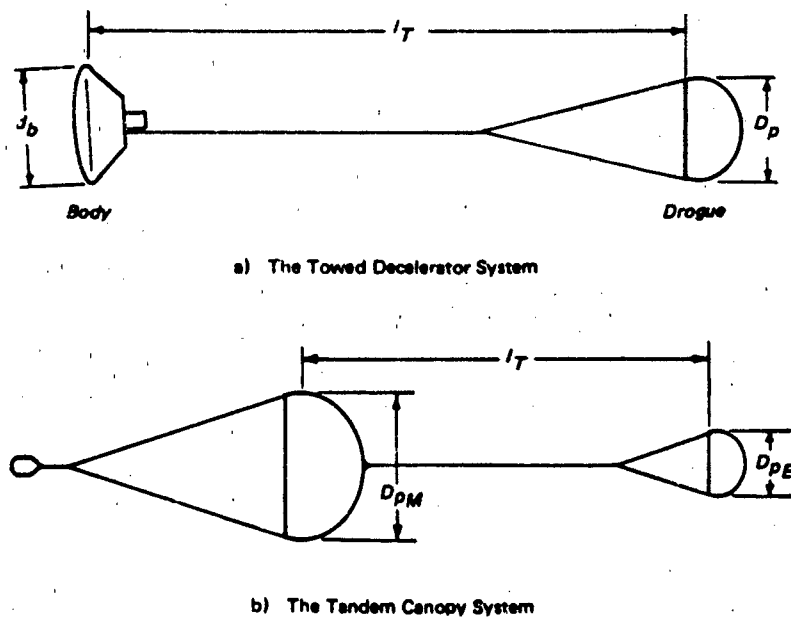
Figure 6.39 Decelerator Systems Subject to Strong Wake Effects
