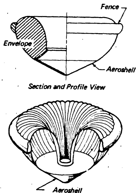
Figure 2.12 Attached Inflatable Decelerators
