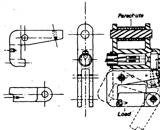
Figure 3.24 Parachute Canopy Release Assembly, Latch Type
