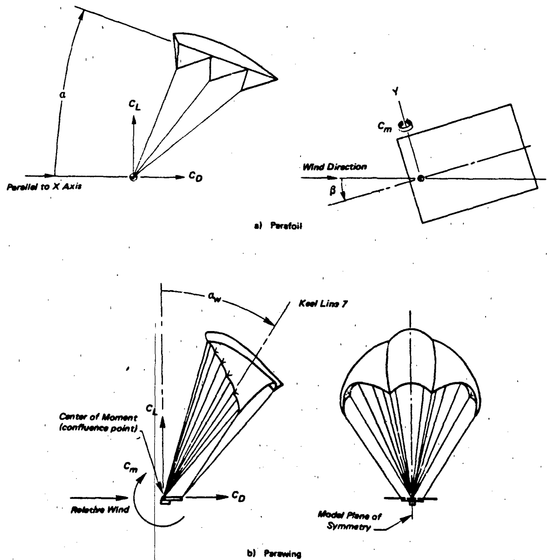
Figure 6.78 System of Axis and the Positive Direction of the Forces, Moments and Angles Used in the Presentation of the Data
