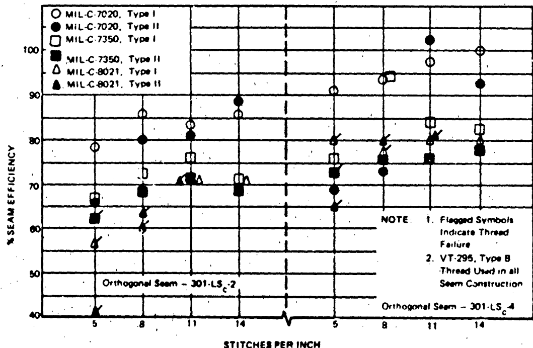
Figure 4.14 Dependence of Seam Efficiency on Stitches per Inch
