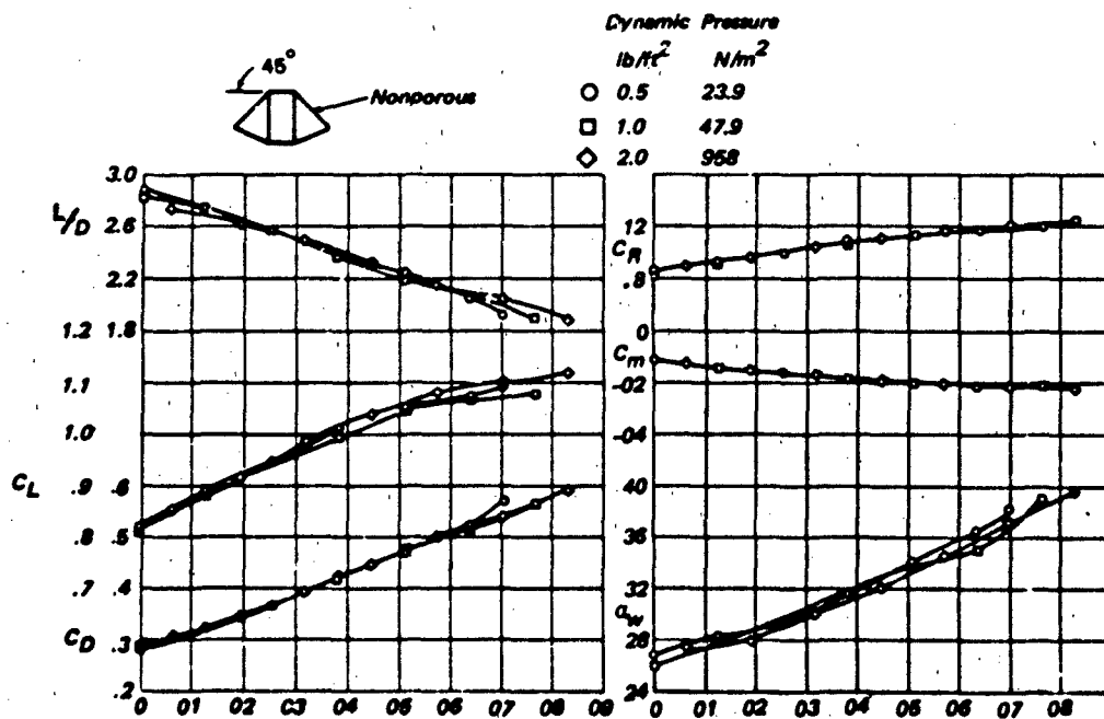
Figure 6.77 Effects of an Increase in Dynamic Pressure on Longitudinal Aerodynamic Characteristics of a Twin-Keel All Flexible Parawing
