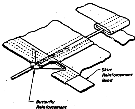
Figure 4.19 Cord Line Attachment with Butterfly
