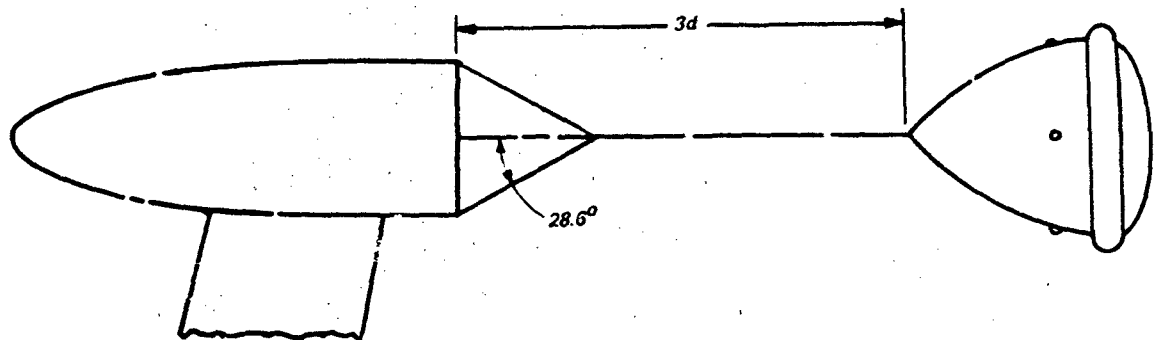
a) Model Booster With Ballute Drogue in Wind Tunnel
