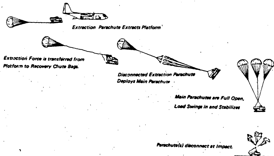
Figure 1.22 Standard Airdrop Method
