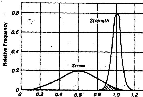
Figure 7.55 Exaggerated Stress-Strength Distribution
