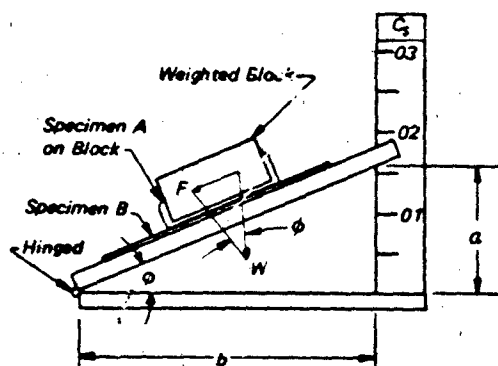
Figure 5.17 Inclined-Plane Apparatus for Measuring Coefficient of Sliding Friction
