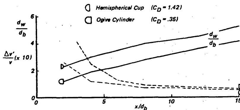
Figure 6.44 Wake Width & Center-Line Velocity Increment vs Distance From Body of Revolution (Adapted from Ref. 382)
