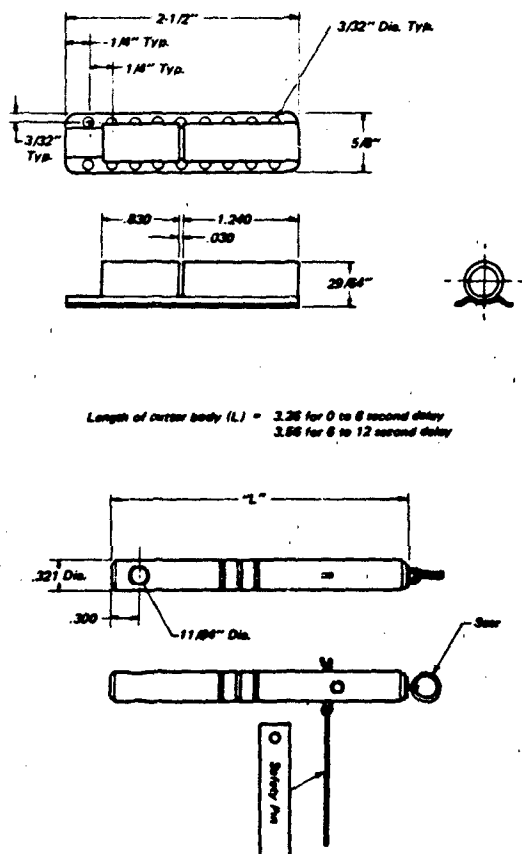
Figure 3.12 Reeling Line Cutter and Mounting Bracket
