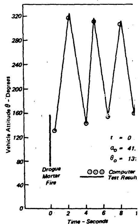
a) \theta Vs Time, Computer and Drop Test Results (Single Drogue)
