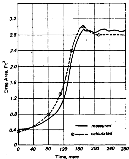
Figure 6.86 Calculated and Measured Drag Area
