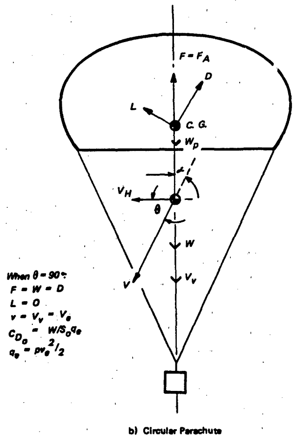
Figure 6.33 Generalized Decelerator System in Stable Equilibrium Descent Through Homogeneous Air Mass ( \rho = \text{const.}; F_y = 0, M = 0 )
