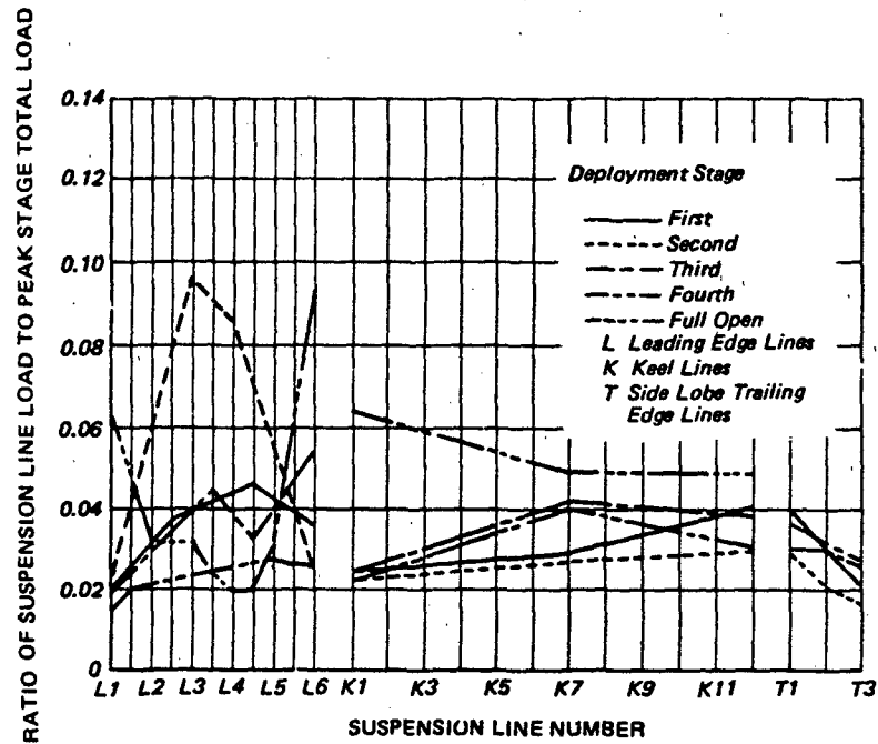
Figure 6.32 Distribution of Suspension Line Loads for Each Opening Stage of Reefed 4000 Ft 2 (SW) Twin Keel Parawing (Reference 398)
