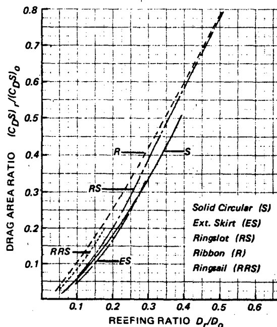
Figure 6.64 Drag Area Ratio vs. Reefing Ratio for Solid Circular, Extended Skirt, Ringslot, Ringsail and Ribbon Parachutes (from Ref. 393)
