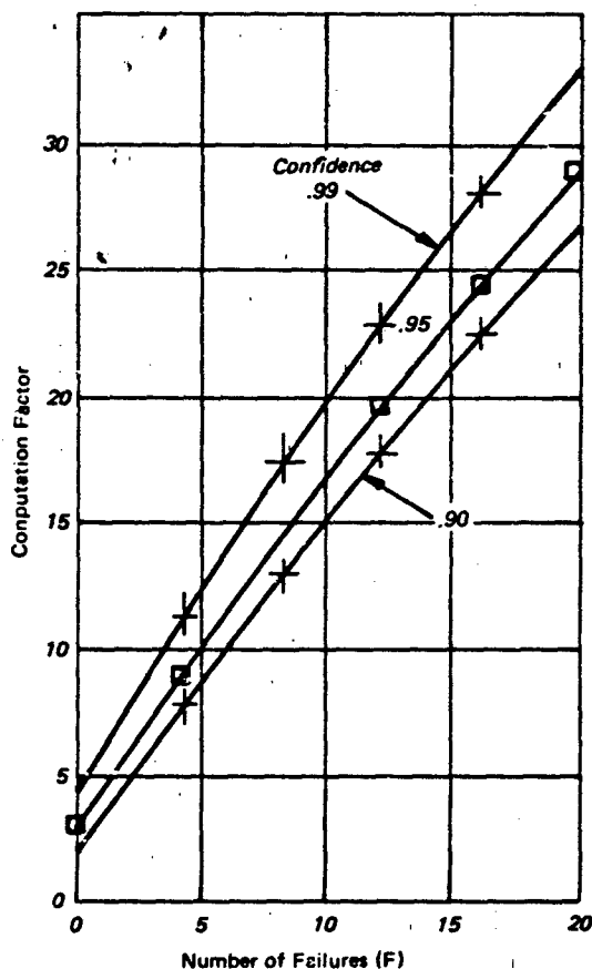
Figure 7.52 Reliability From a Series of Trials
