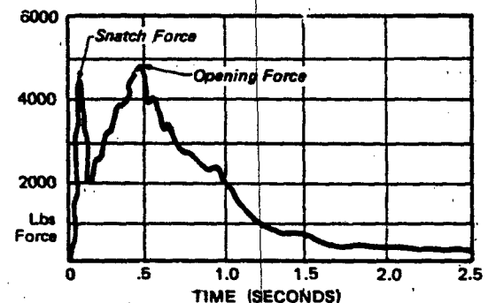
Figure 6.2 Snatch and Opening Forces of a 28 Ft D_0 Solid Flat Circular Parachute
