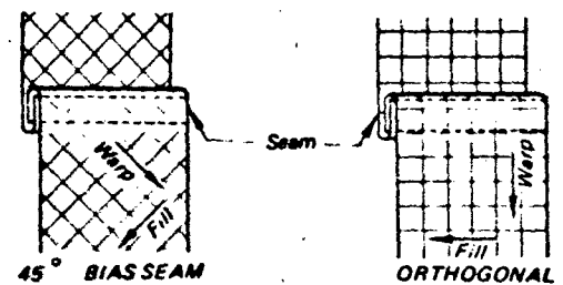
Figure 4.15 Fabric Orientation
