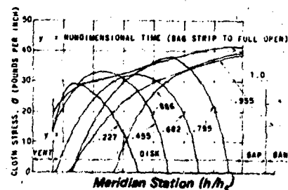
e) Design Limit Cloth Stress Distribution at Various Stages of Inflation
