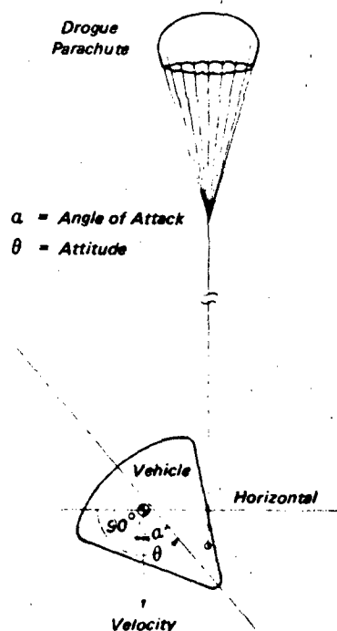
Figure 7.3 Vehicle Orientation at Drogue Parachute Line Stretch
