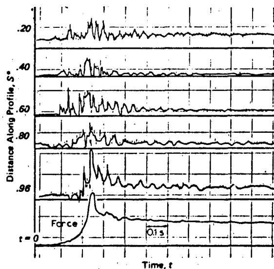
Figure 6.88A Canopy Stress and Total Force Measured on a 28 Gore Solid Flat Circular Model Parachute
