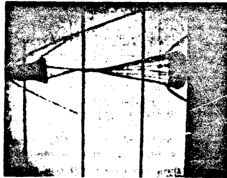
Figure 6.47 Schlieren Photograph of the Flow Fields About a Hyperflo Type Parachute at M 4.0 (Free flight test in Wind Tunnel)
