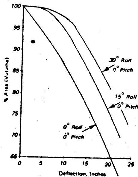
d) Impact Bag Cross-Sectional (Volume) Variation For Different Roll Angles and Deflection (Stroke) Conditions.
