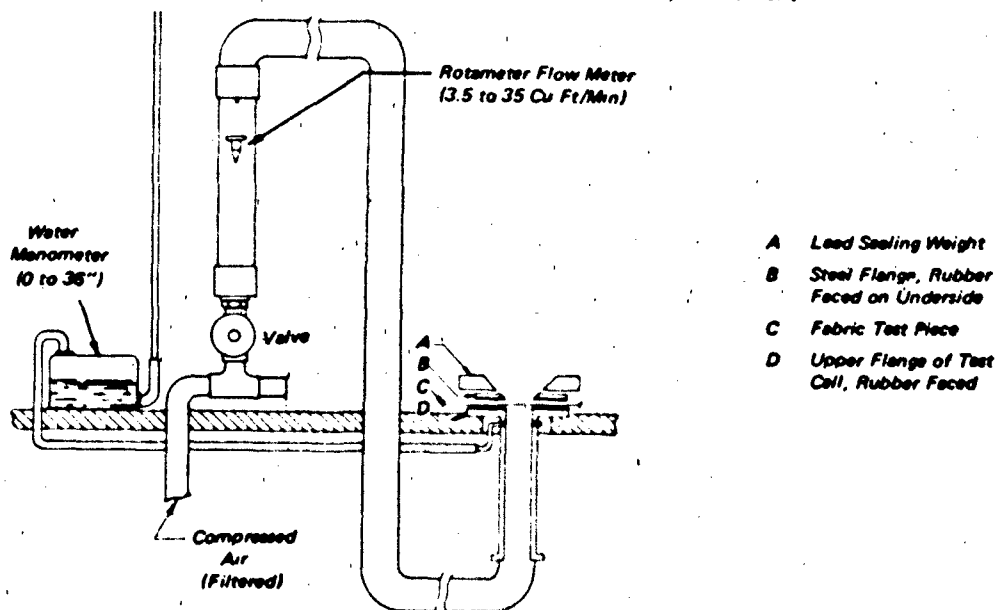
Figure 5.16 Air Permeability Apparatus
