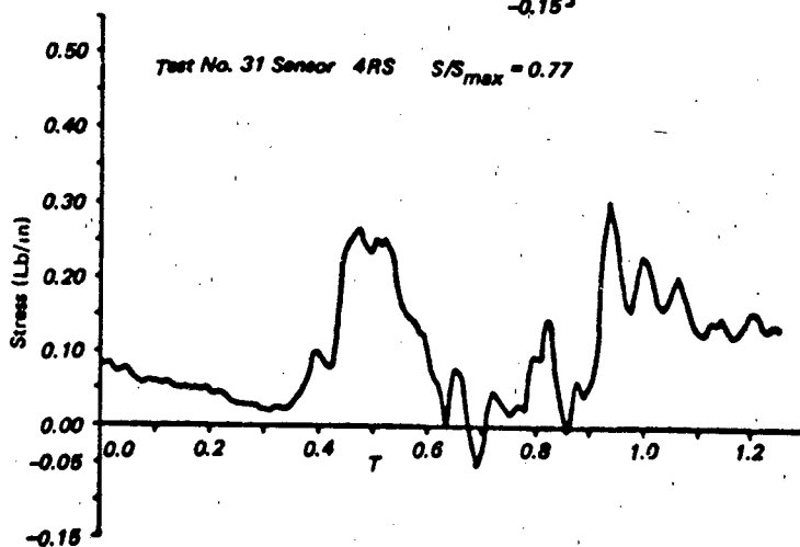
Figure 6.89 Measured Opening Forces and Canopy Stress of Model Ringslot Canopy (Continued)
