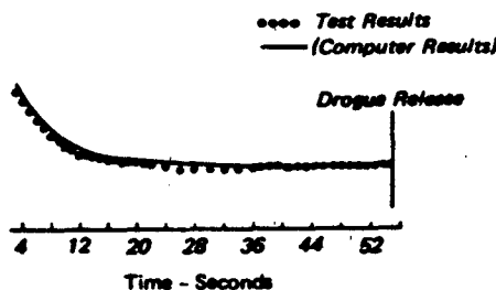
d) Vehicle Dynamic Pressure Vs Time. Computer and Test Results. (Twin Drogue)
