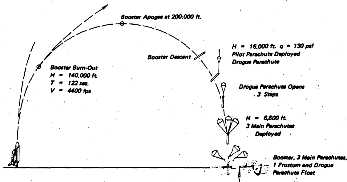
Figure 1.12 Solid Rocket Booster Recovery Sequence
