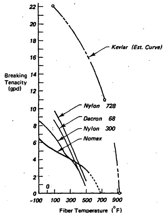
Figure 8.9 Temperature Strength Loss of High Tenacity Synthetic Textile Fibers
