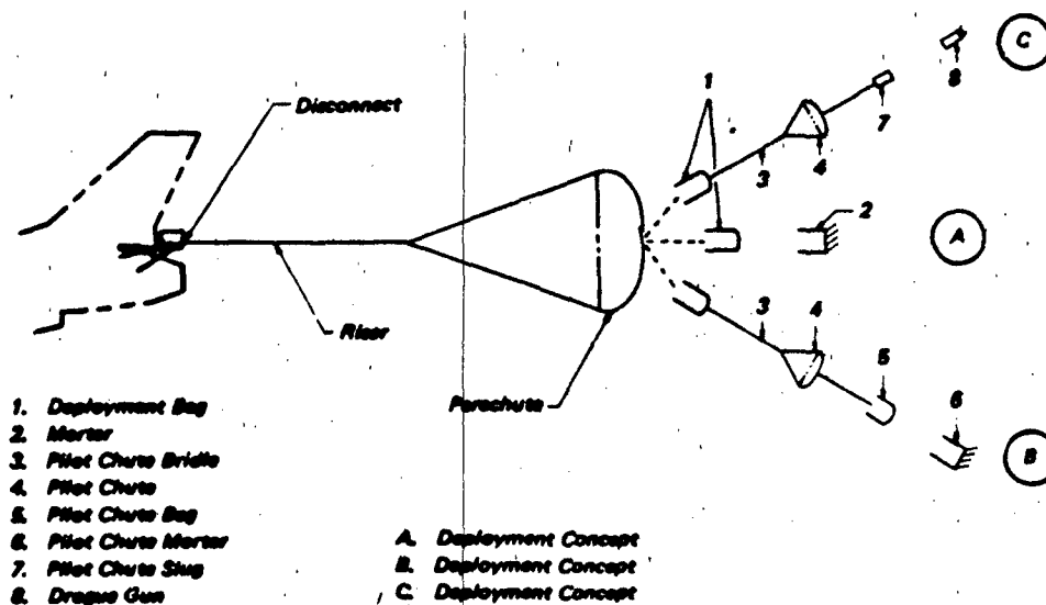
Figure 1.31 Spin Recovery Parachute and Deployment Sequence
