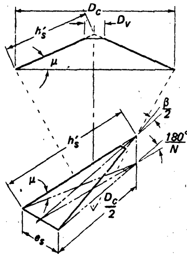
Figure 2.4 Construction Schematic of Conical Canopy
