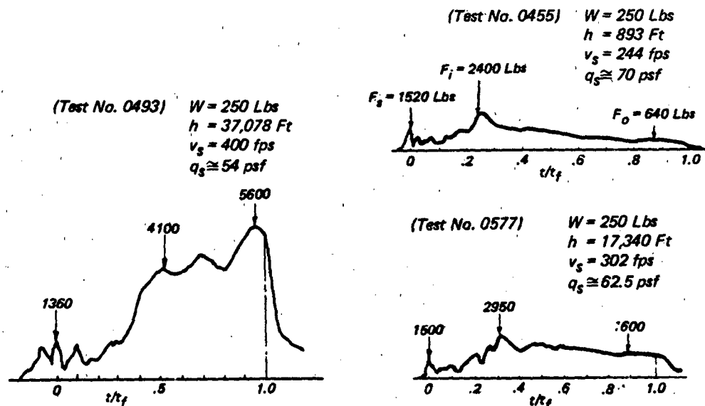
Figure 6.21 Measured Force vs Normalized Time During Inflation of T-10H (High Strength) 35 Ft ( D_o ) 10% Extended Skirt Parachute Deployed Lines - First Horizontally from Cylindrical Vehicle (Ref. 357)
