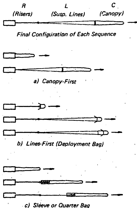
Figure 6.1 Schematic of Different Deployment Sequences
