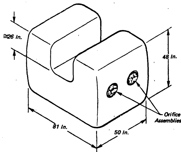
Figure 6.97 Maximum Inflated Dimensions Impact Bag (Ref. 496)
