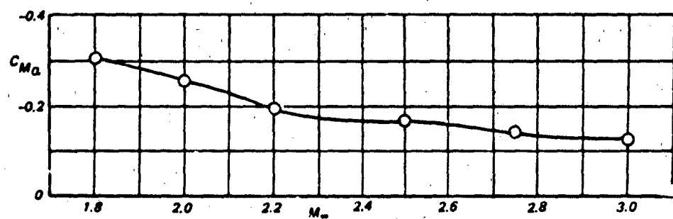
c) Variation of the Rate of Change of Pitching Moment Coefficient with Mach Number at \alpha = 0
