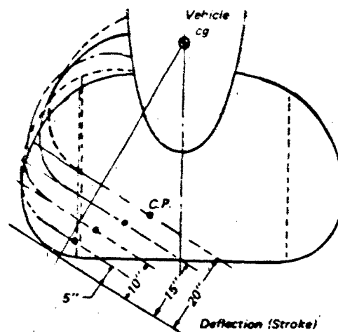
b) Footprint Analysis of Impact Bag For 30° Roll, 0° Pitch Condition. MQM-34D
