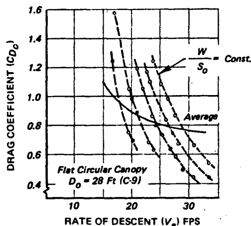
a) Variation of Drag Coefficient Data for Different Constant Unit Loads vs Rate of Descent (From Ref 382)
