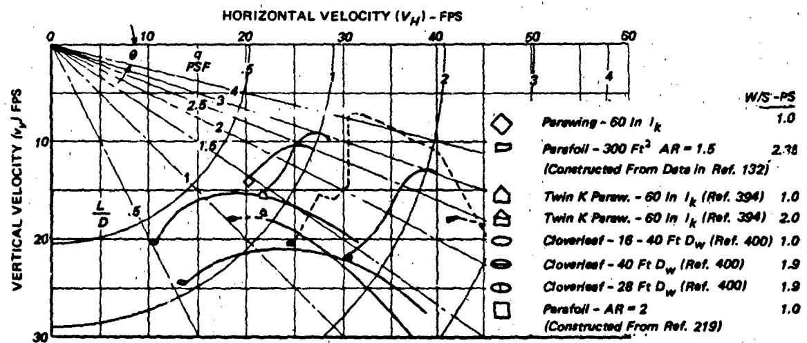
Figure 6.36B Effect of Wing Loading ( W/S_W ) on Components of Glide Over Controllable Range of L/D Modulation
