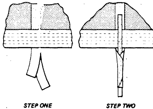
Figure 4.22 Tapered Radial/Suspension Line Joint
