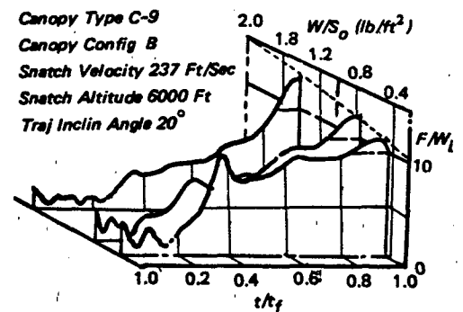
d) EFFECT OF CANOPY LOADING PARAMETER, W/S_o
