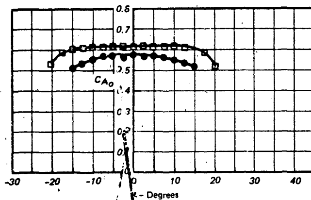
A) Ringslot (50 Inch Prototype) and Ribbon (100 Inch Prototype), \lambda_g = 20\%
