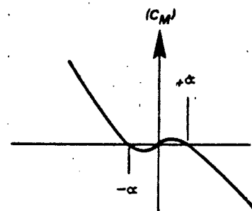
b) Variation of Parachute Moment Coefficient with Canopy Angle of Attack
