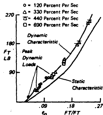
a) Derived Dynamic Load-Elongation Characteristic
