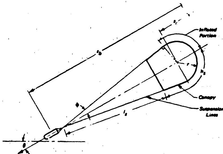
Figure 7.12. Canopy Geometry and Trajectory Coordinates
