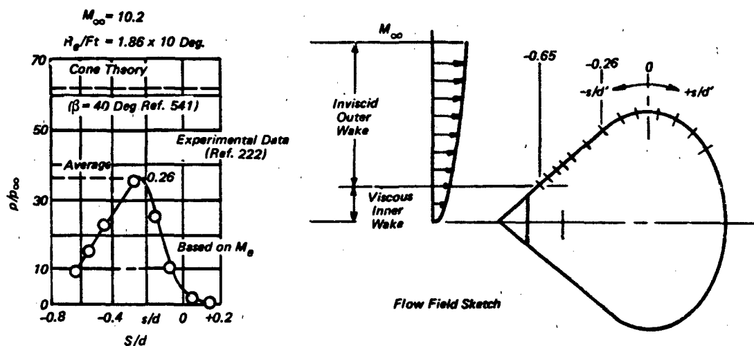
Figure 7.32 Pressure Distribution Over Ballute (Test TB - 4)
