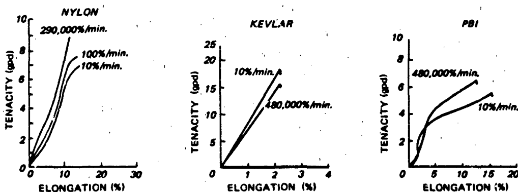
Figure 4.3 Tenacity - Elongation: Effect of Loading Rate
