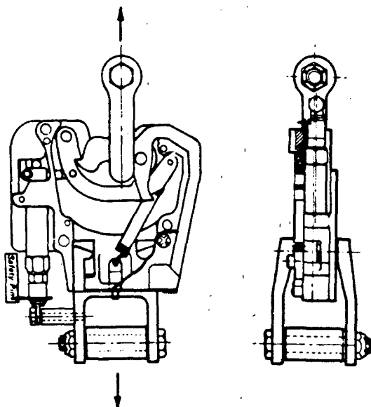
Figure 3.18 Cargo Parachute Release, 5000 Pound Capacity
