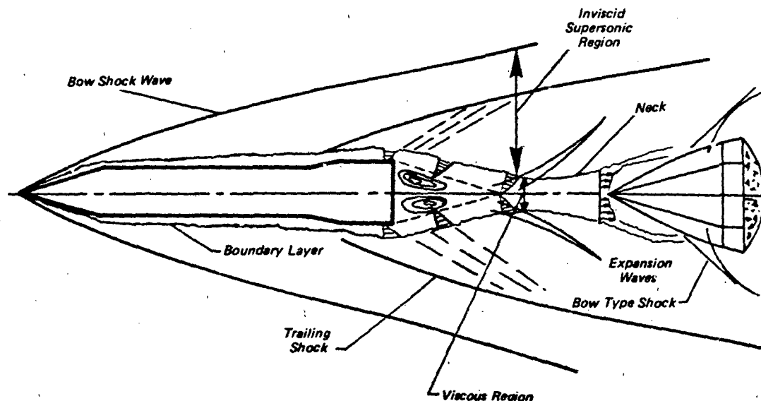
Figure 6.90 Typical Body - Drogue Supersonic Flow Field
