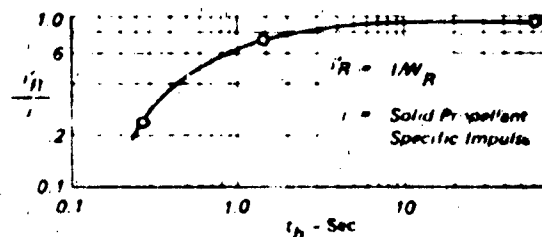
Figure 8.12 Rocket Specific Impulse Ratio vs Burn Time (Ref. 574)
