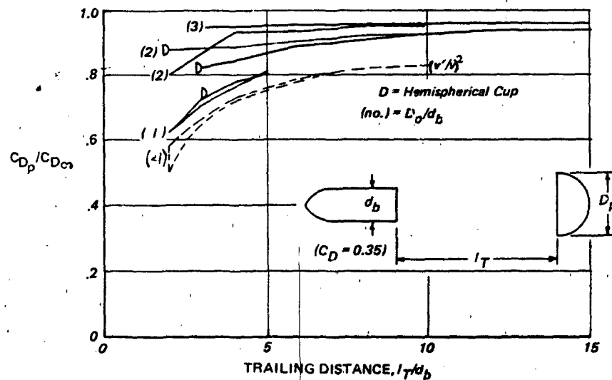
Figure 6.43 Wake Drag Coefficient for Small Circular Models (Disk & Hemispherical Cup) (Adapted from Ref. 382)
