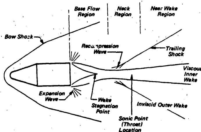
Figure 6.48 Schematic of Unmodified Supersonic Wake Details and Nomenclature for Body of Revolution
