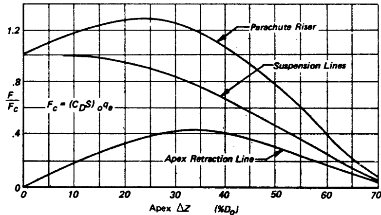
b) Forces in Parachute Suspension Members vs Apex Retraction Distance, \Delta Z , During Equilibrium Descent
