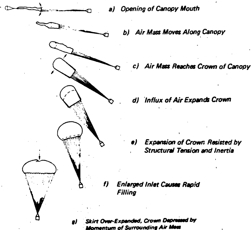
Figure 6.9A Stages in Parachute Inflation
