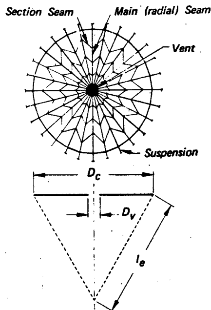
Figure 2.3 Planform and Construction Schematic for a Flat Circular Parachute
