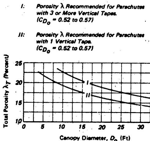
Figure 8.6 Recommended Total Porosity of Ringslot Canopy Designs
