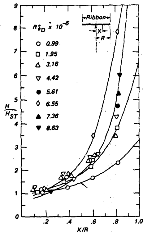
Figure 7.27 Distribution of Heat Transfer Coefficients on Upstream Side of Ribbon Grid (Ref. 536)
