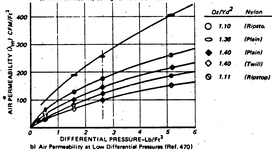
Figure 6.56 Typical Variation of Mechanical and Effective Porosities of Nylon Parachute Cloth With Differential Pressure
