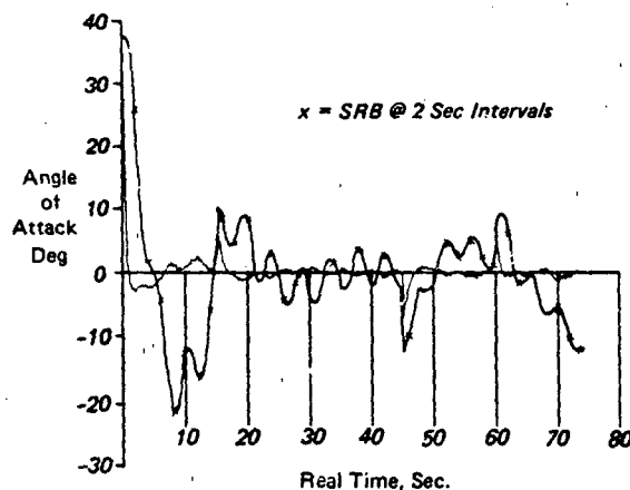
c) System Angle of Attack Response to Non-Steady Air Mass Figure 7.45 Continued
