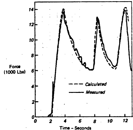
Figure 7.9 Mass Time Method; Calculated vs Measured Opening Loads
