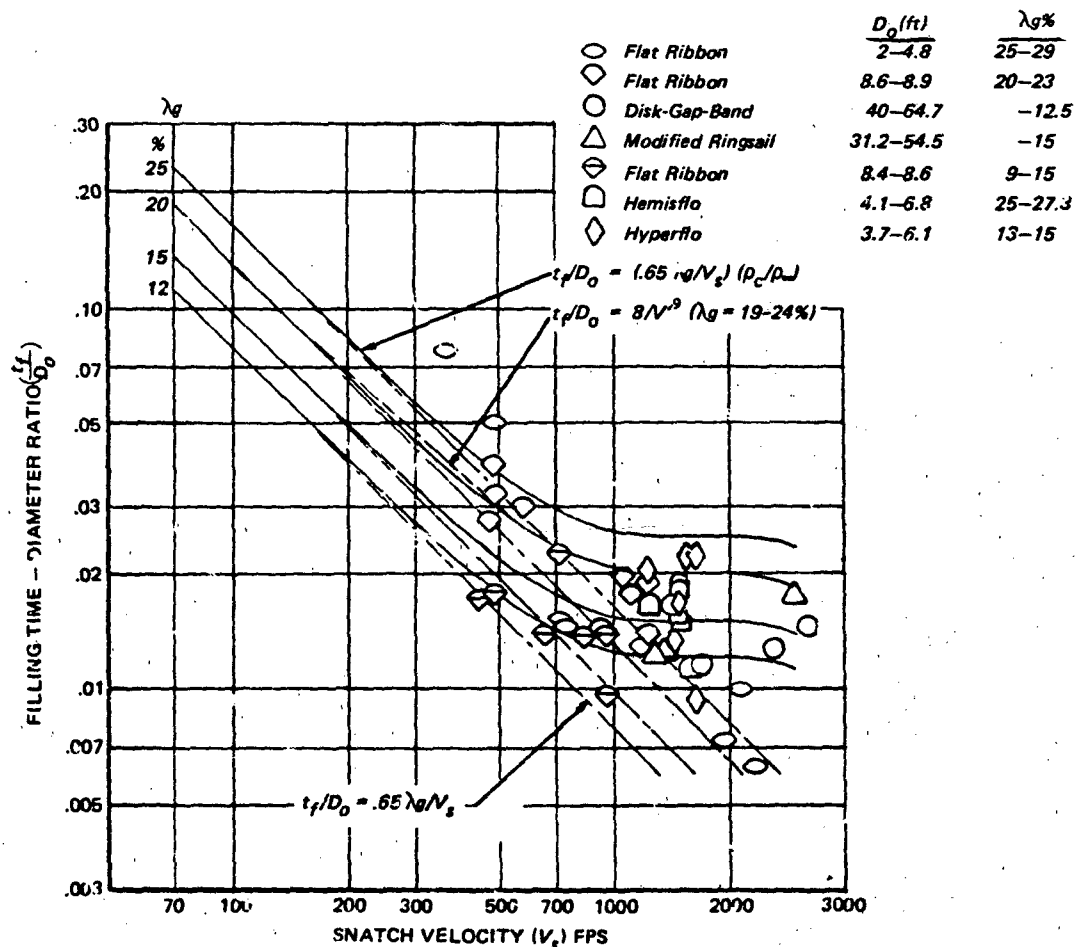
Figure 6.17 Apparent Variation of Filling Time With Velocity for Slotted Canopies (Infinite Mass Condition)
