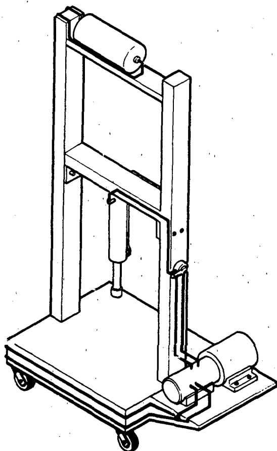
Figure 4.33 Hydraulic Packing Press
