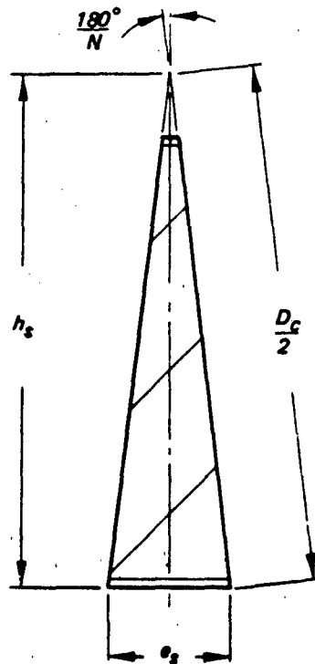
GORE LAYOUT
