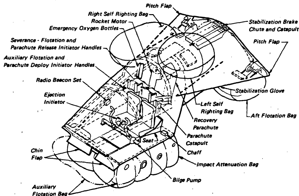
Figure 1.19 F111 Crew Module Configuration
