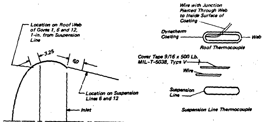
a) Location of Thermocouples
