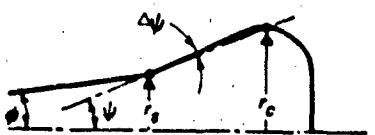
Figure 7.14 Details of Spring Mass-Momentum Model of Inflating Polysymmetric Parachute
