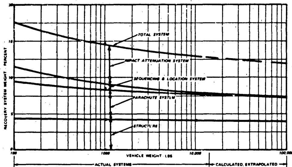
Figure 8.15 Recovery System Weight Breakdown
