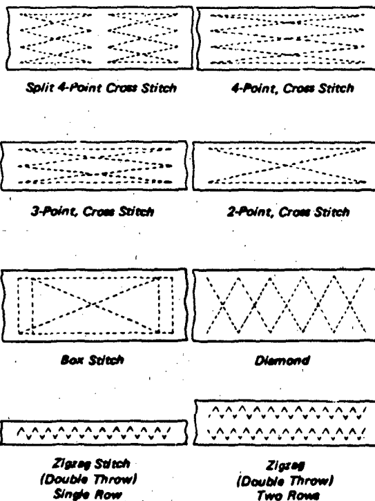
Figure 4.18 Example of Stitch Patterns
