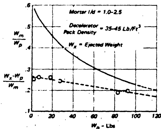
b) Variation of Mortar Weight Ratios with W_p
