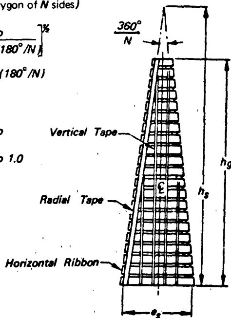
GORE LAYOUT
