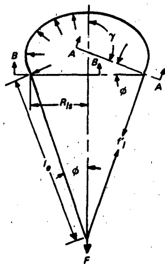
b) Inflated Profile Full Open After Disreefing
