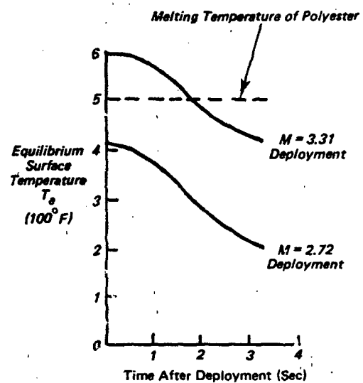
Figure 7.29 Calculated Temperatures in Crown of 40 Ft D_o Disk-Gap-Band Parachute (Ref. 486)
