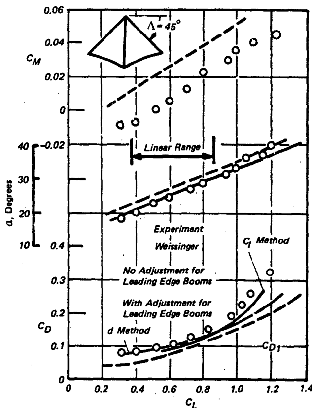
b) Characteristics of a Flexible NASA Planform Parawing with A = 2.83 and 2\theta = 130.5^\circ .
