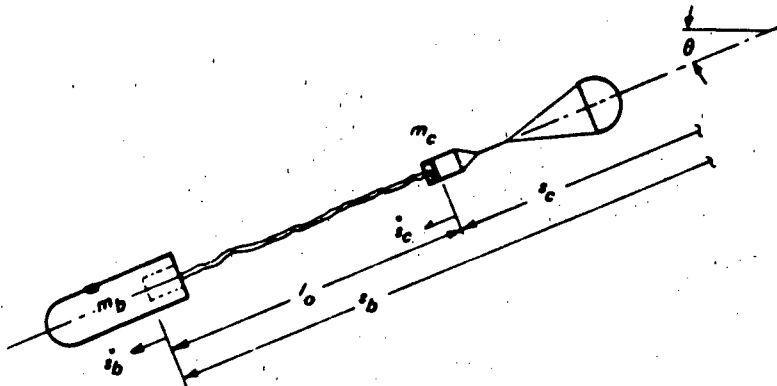
Figure 7.8 System Configuration During Deployment
