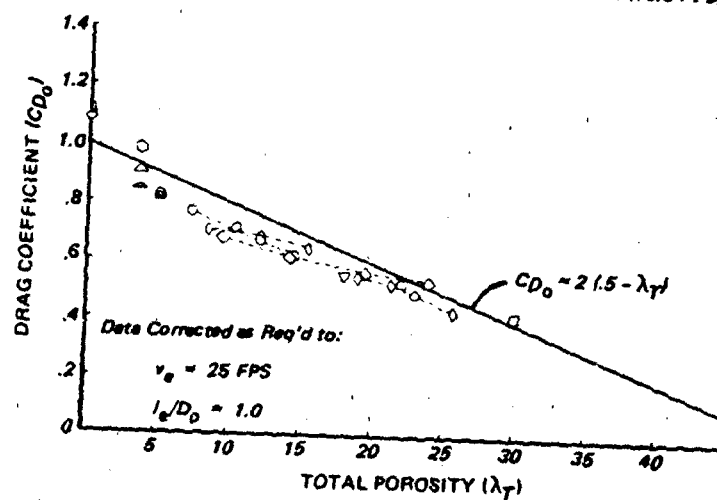
Figure 6.58 Effect of Canopy Porosity on Parachute Drag Coefficient
