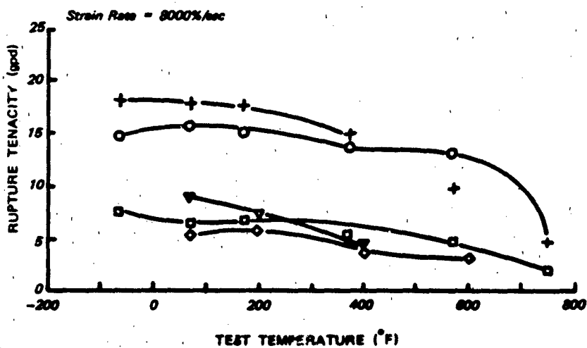
Figure 4.4 Rupture Tenacity as a Function of Tenile Test Temperature (stress values based upon denier measured at 70°F) (Ref. 579)
