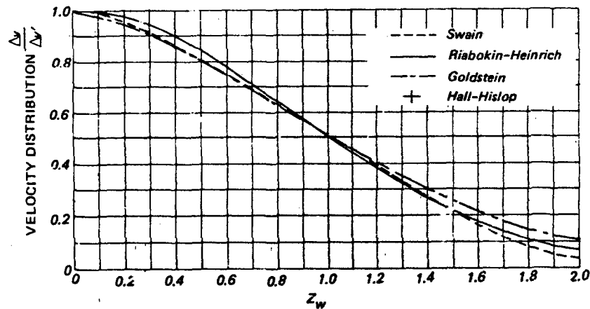
Figure 6.42 Velocity Distribution in Accordance With Analytical and Experimental Studies
