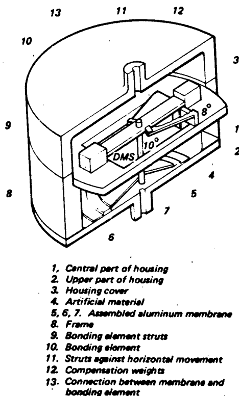
Figure 5.31. Differential Pressure Transducer with Compensation for Linear Acceleration
