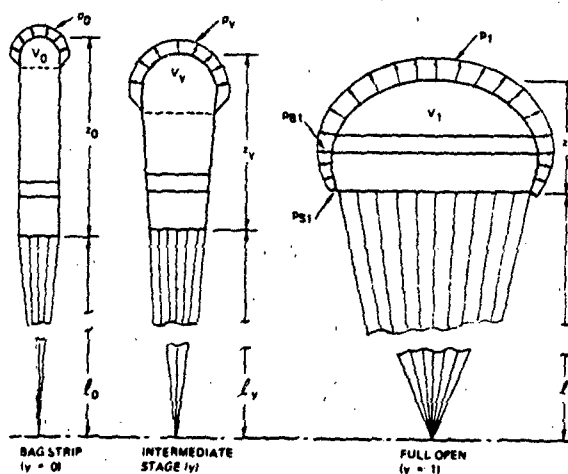
d) Inflation Stage Sequence
