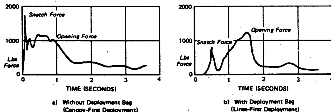
Figure 6.7 Effect of Deployment Bag on Relative Magnitude of Snatch Force During Deployment of a 28 Ft D_0 Solid Flat Circular Parachute
