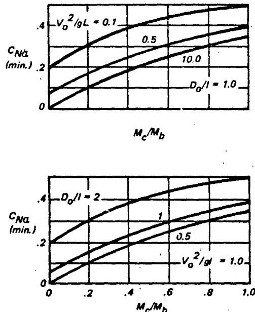
Figure 7.42 Effect of Froude Number and Slenderness Ratio on Stability C_{A_0} = 0.7 Zero Porosity
