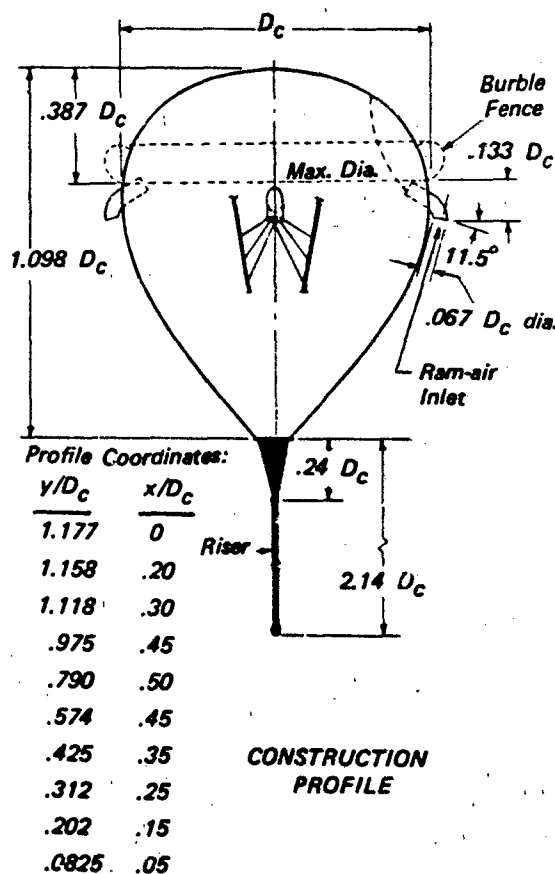
Figure 2.11 Ballute Geometry
