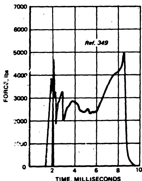
Figure 6.8 Force Record for Pilot Chute Bridle Test
