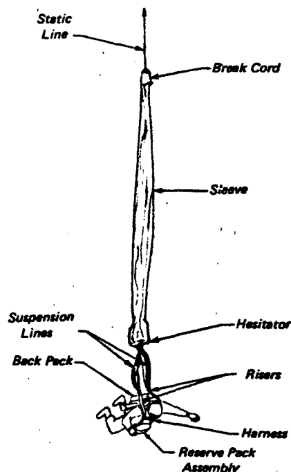
Figure 3.26 Components of Typical Decelerator Subsystems
