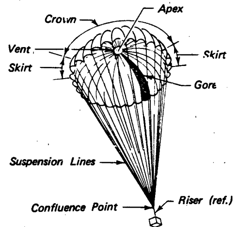
Figure 2.1 Parts of a Parachute
