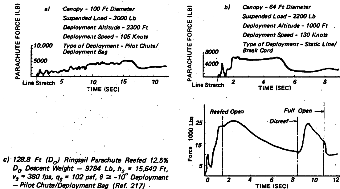
Figure 6.22 Airdrop and Recovery Parachutes - Typical Opening Force vs Time
