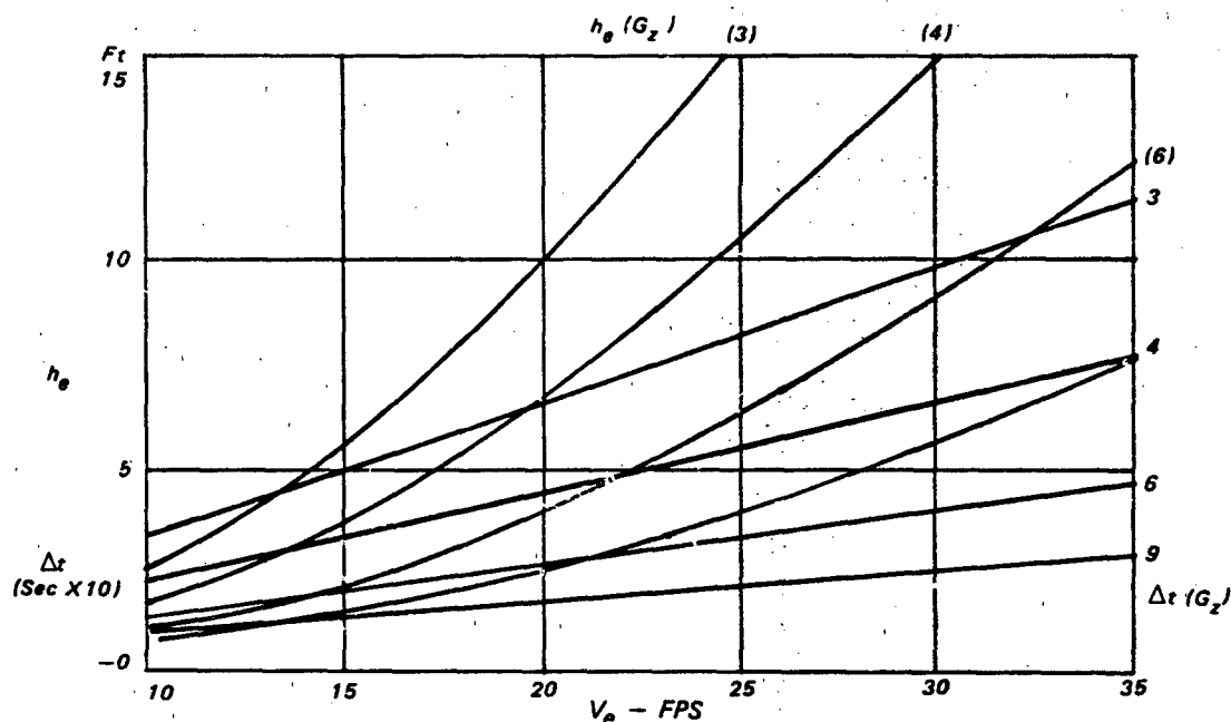
Figure 7.49 General Characteristics of Impact Attenuation System Vs Vehicle Vertical V_0 and Load Factor
