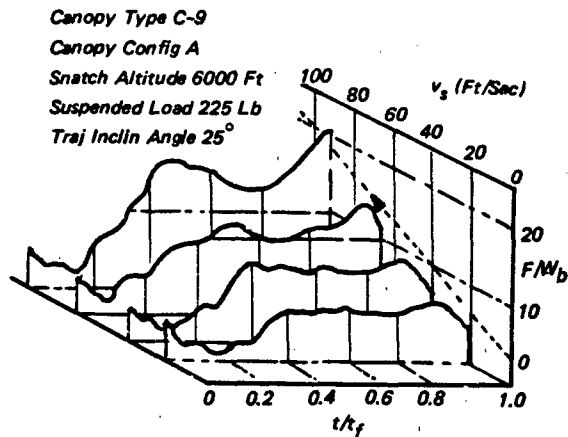
a) EFFECT OF VELOCITY AT SNATCH, v_s
