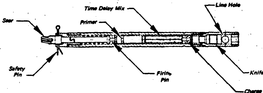
Figure 3.11 Reefing Line Cutter
