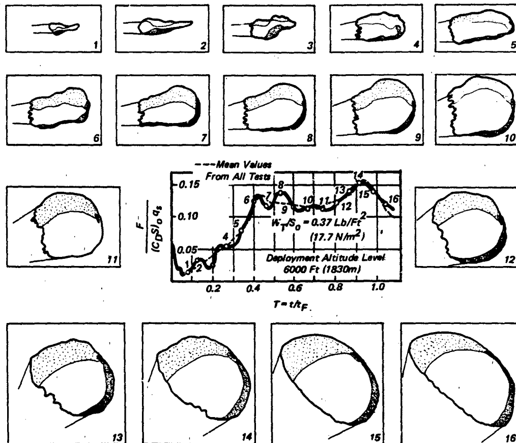
Figure 6.24 Comparison Between Inflating Canopy Shape and Generated Force.
