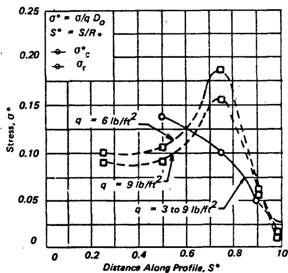
Figure 6.87 Measured Circumferential and Radial Stresses
