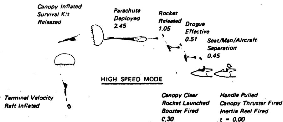
Figure 1.17 Tractor Rocket Escape System Operation (Continued)
