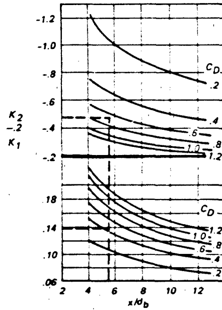
Figure 7.34 Wake Coefficients vs (x/d_b)
