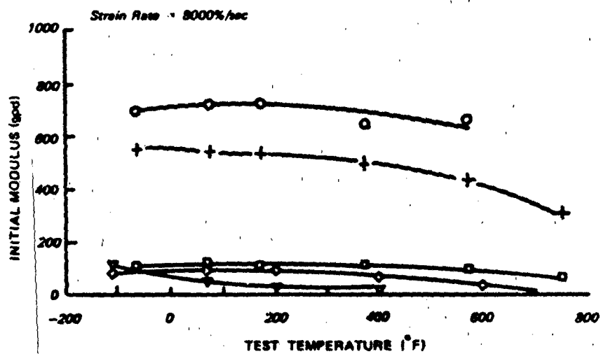
Figure 4.5 Initial Modulus of Yarns as a Function of Tensile Test Temperature (based upon at-temperature yarn dimensions) (Ref. 578)
