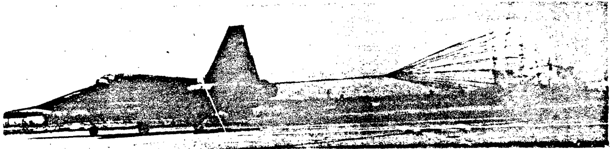
Figure 5.7 F-5 Aircraft Testing of 15-Foot Ringslot Deceleration Parachute
