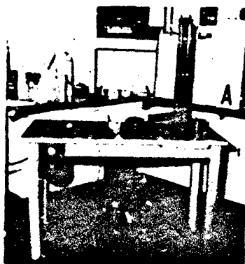
Figure 5.15 The Frazer Air Permeability Instrument
