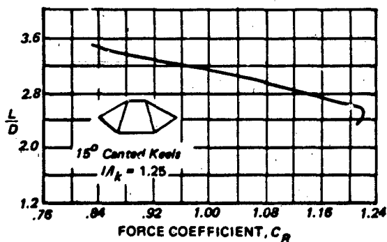
b) Performance Characteristics of an Advanced Twin-Keel Parawing
