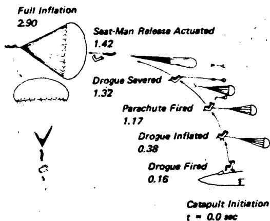
Figure 1.16 Aces II, Mode 2 Operation
