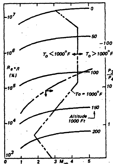
Figure 7.24 Sonic Reynolds No. and P_3/P_4 vs. Mach No. (Ref. 534)
