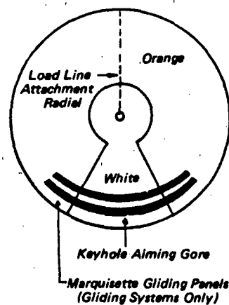
c) Top View of MARS Main Canopy
