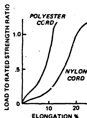
Figure 4.6 Load vs Elongation of Cords
