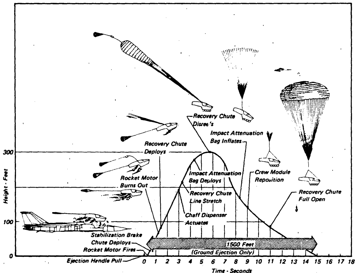
Figure 1.20 F-111 Crew Module Low Speed Ejection Sequence
