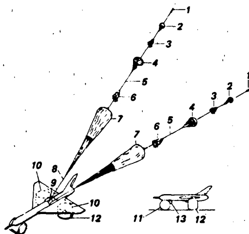
Figure 1.2 USD-5 Recovery System
