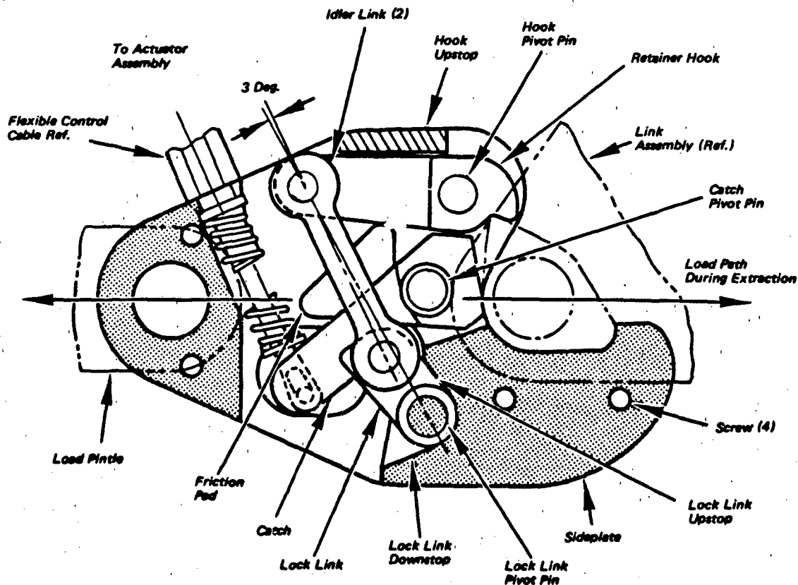
Figure 3.17 Latch Assembly
