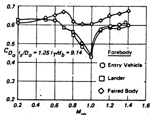
Figure 6.54 Effect of Forebody Shape on C_{D_0}
