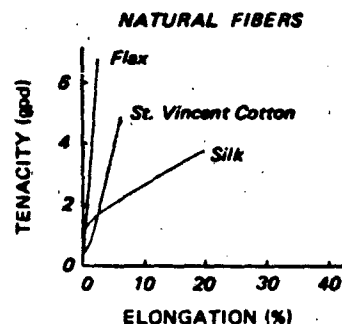
Figure 4.2 Tenacity vs Elongation Of Textile Fibers
