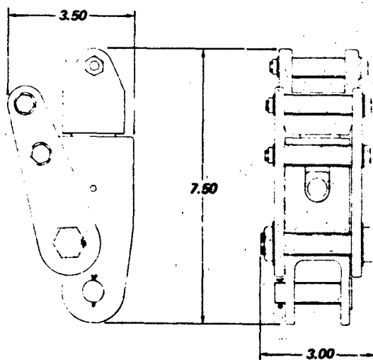
Figure 3.14 MARS Release
