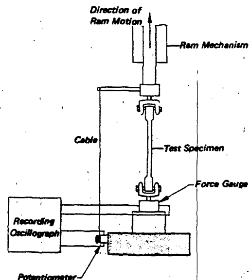
Figure 5.13 Suspension Line Impact Loading Apparatus for Strain Rates of 50% to 200%/Sec. (Ref. 331)
