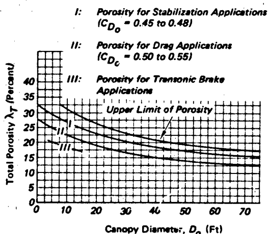
Figure 8.5 Total Porosity vs. Canopy Diameter for Flat Circular Ribbon Canopies
