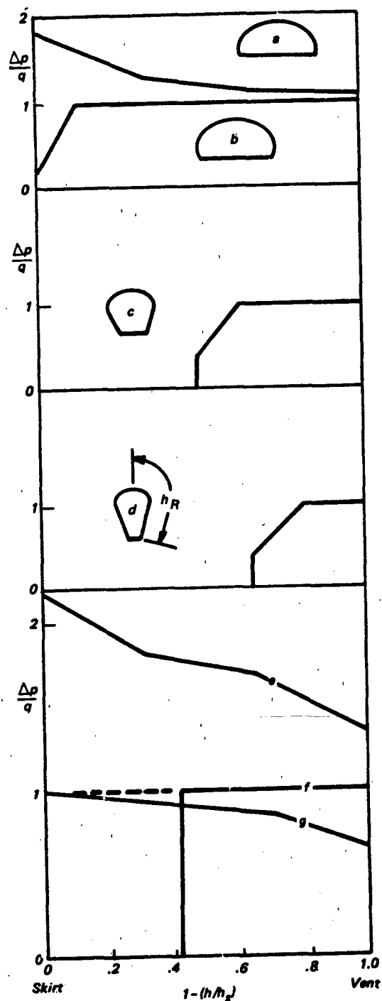
Figure 7.18 Pressure Distribution in Inflating Parachutes (Ref. 221)
