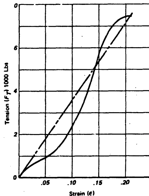
Figure 7.6 Average Static Load - Strain Characteristic of 1" Nylon Webbing
