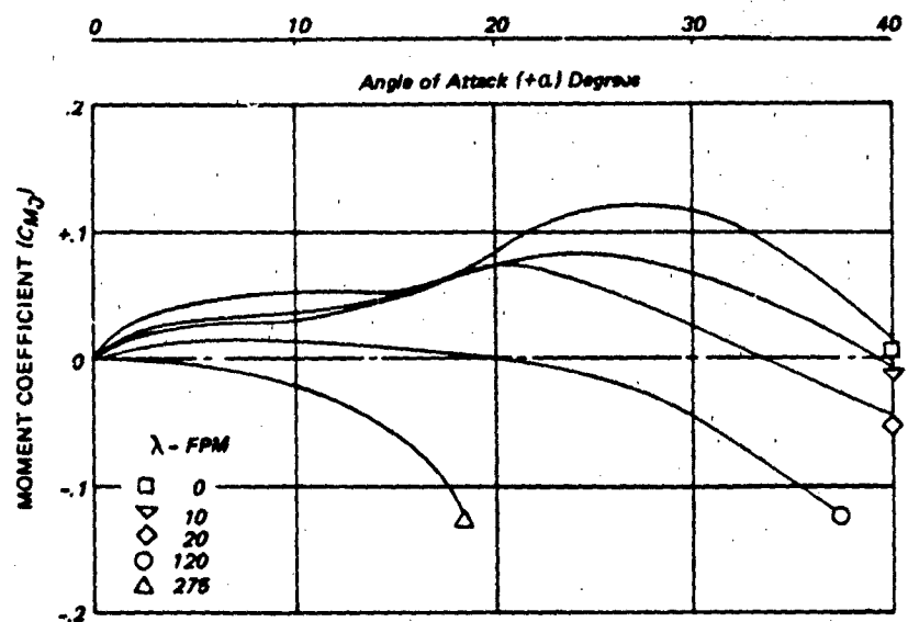
Figure 6.73 Effect of Air Permeability on C_{Mp} vs α of Small Solid Flat Circular Canopies in Wind Tunnel
