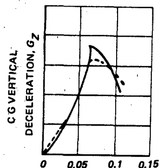
b) Typical Bag Pressure and Vertical Deceleration Transients
