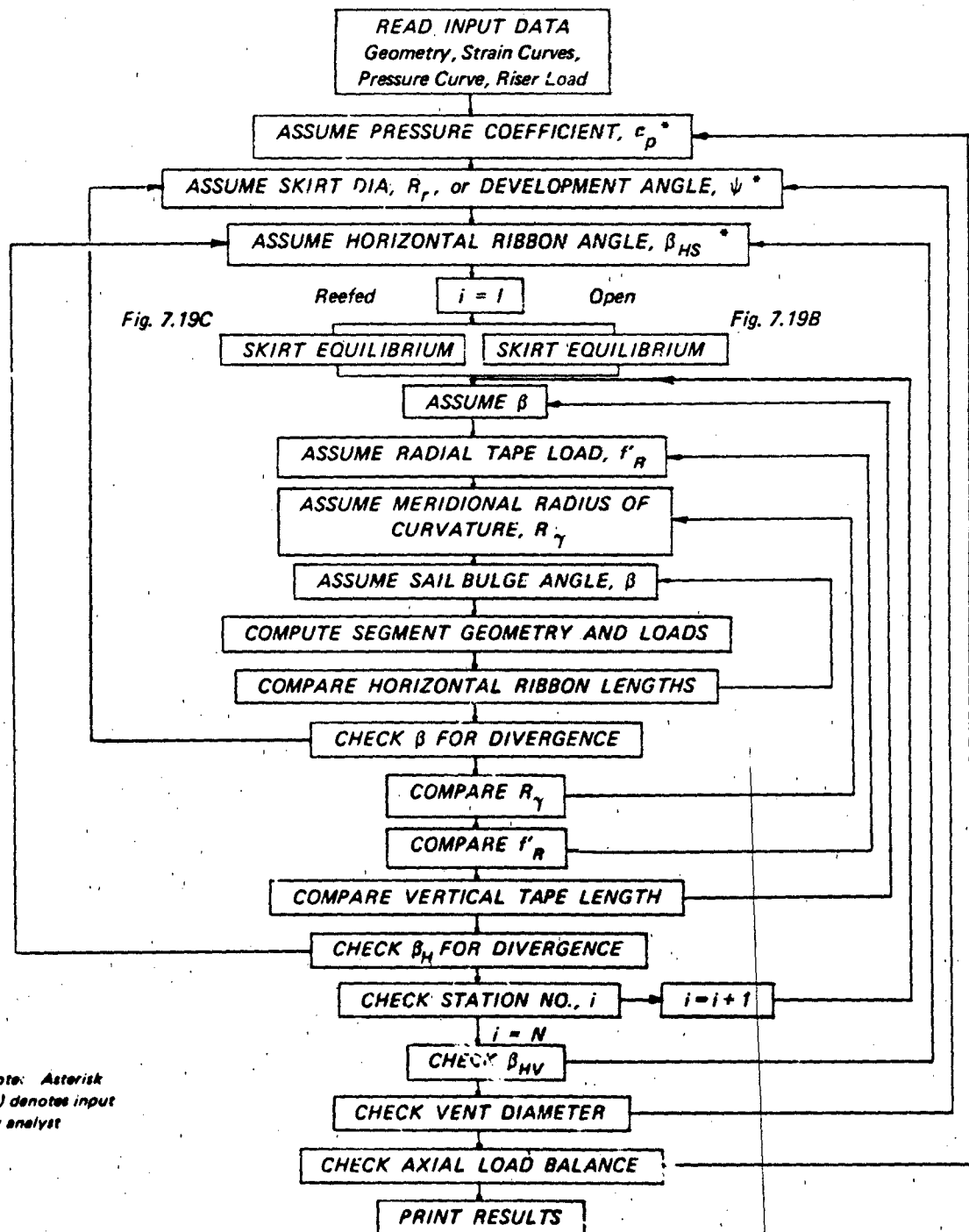
Figure 7.20 Flow Diagram for Program CANO 1
