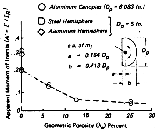
Figure 7.11 Measured Apparent Moment of Inertia of Rigid Canopy Models vs \lambda_g
