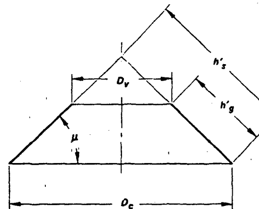
CONSTRUCTION SCHEMATIC
