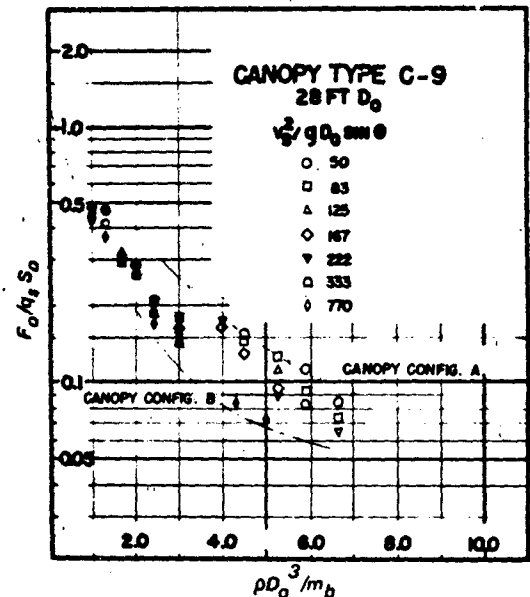
b) Effect of Froude Number on Opening Force Parameter vs Mass Ratio
