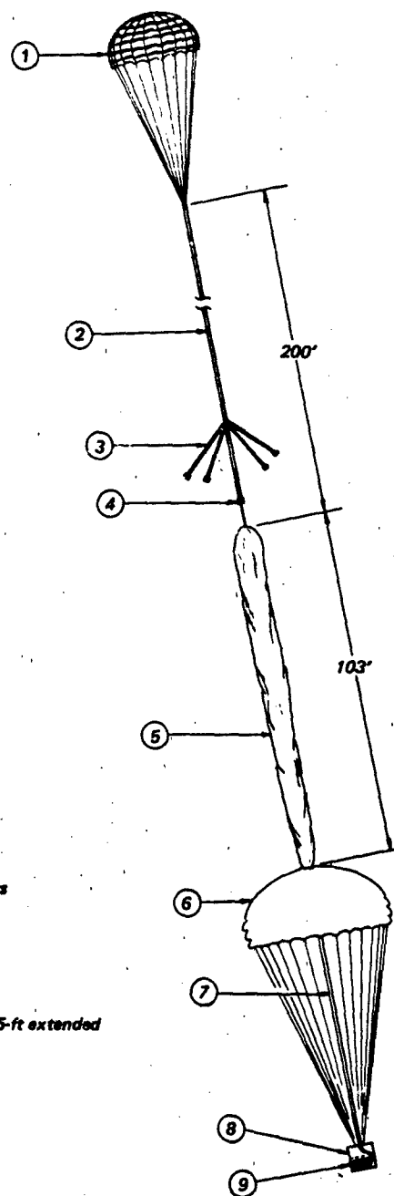
Figure 1.41 Schematic Of Parachute Balloon Train Of Air-Launch Communications Relay Balloon.
