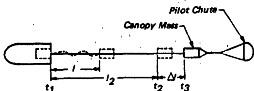
Figure 6.3 System Geometry During Deployment to End of Line-Stretch
