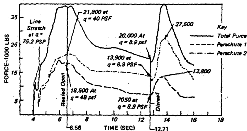
Figure 6.27 Opening Force-Time History for Cluster of Two 12.8 Ft D_0 Ringsails Reefed 13% D_0 for 8 Seconds Deployed at 299 FPS (TAS) at 10,246 Feet Altitude (Weight = 17,720 Pounds) (Ref. 217)
