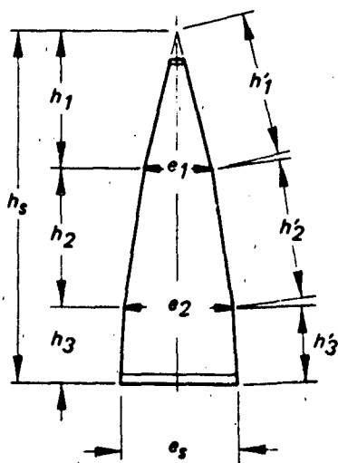
GORE LAYOUT
