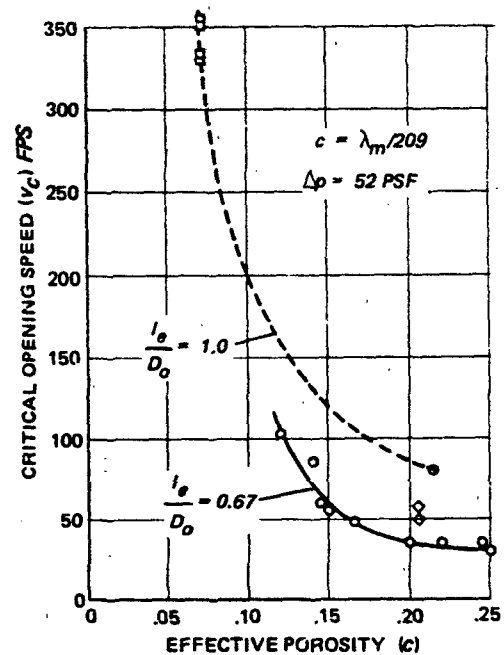
Figure 6.14 Parachute Critical Opening Speed Vs. Total Effective Porosity
