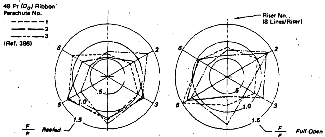
Figure 6.83 Distribution of Suspension Line-Riser Loads in Each Parachute Cluster at \Sigma F (Max.)
