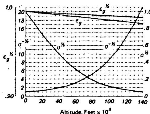
Figure 8.1 Density and Gravity Ratios as a Function of Altitude
