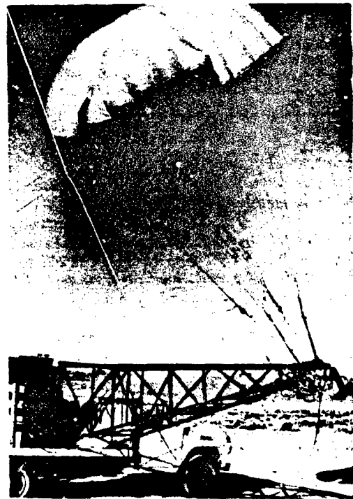
Figure 5.8 Truck Tow Test Rig for Experimental Gliding Parachute
