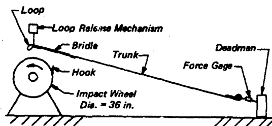
Figure 5.12 Pilot-Chute Bridle Dynamic Test Apparatus
