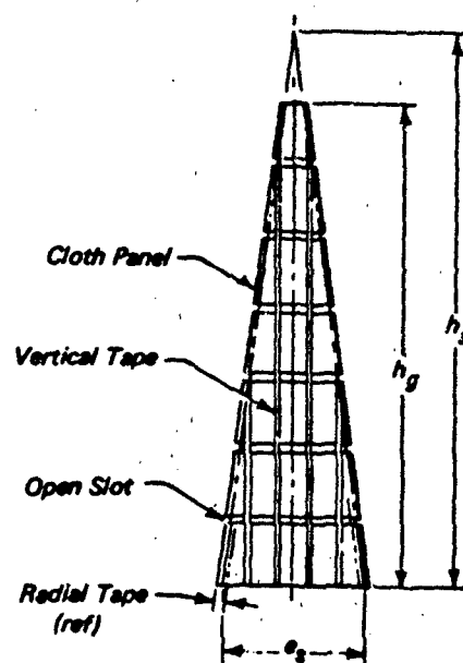
GORE LAYOUT
