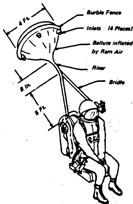
Figure 1.8 Gemini Ejection Seat with Deployed Ballute
