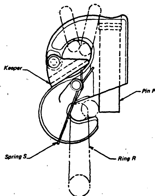
Figure 3.13 Parachute Canopy Release Assembly, Spring Actuated Hook Type
