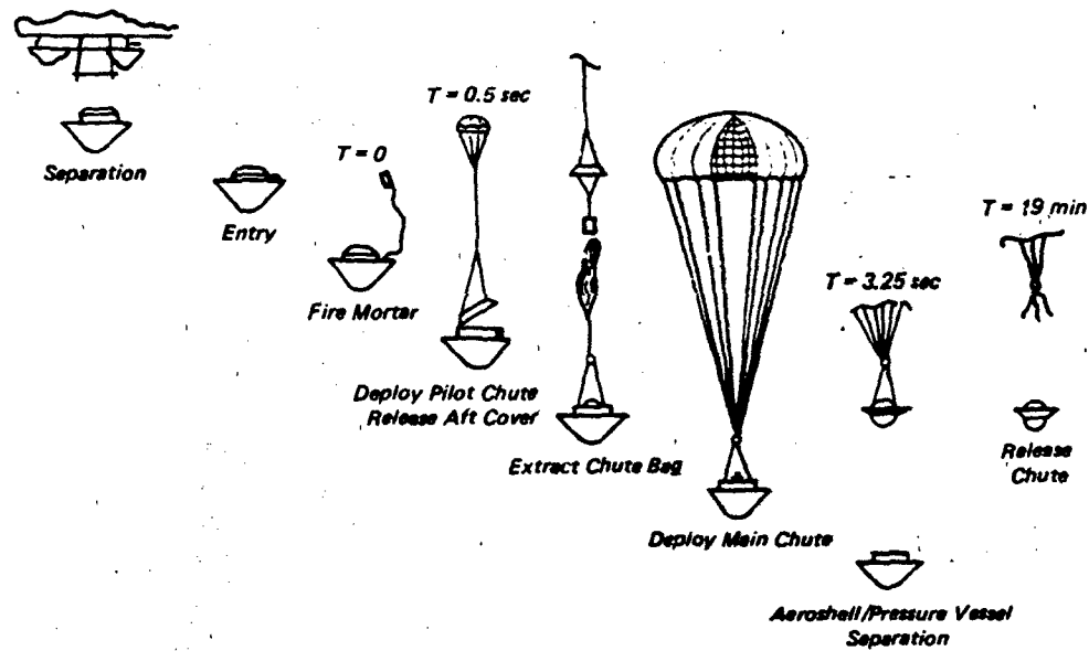
Figure 1.5 Deployment Sequence Of The Venus Probe Decelerator
