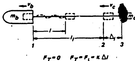
Figure 7.5 System Geometry During Deployment
