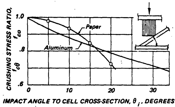
Figure 4.7 Effect of Anisotropic Honeycomb Structure on Crushing Stress with Angular Impact
