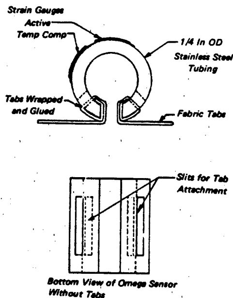
Figure 5.32. Omega Stress Transducer
