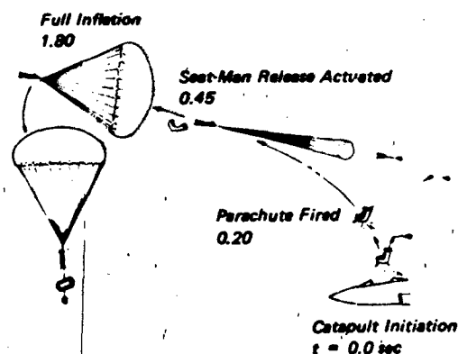
Figure 1.15 ACES II, Mode 1 Operation
