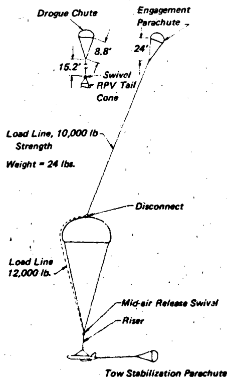
Figure 1.38 100 Ft. Tandem Engagement Parachute (GR-14) for AQM-34V
