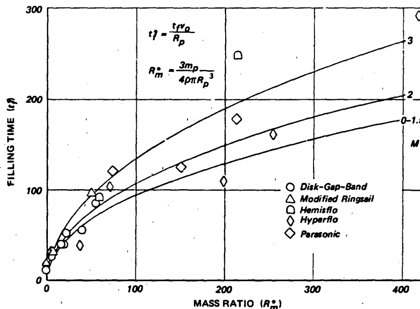
Figure 6.18 Upper Limit Effect of Compressibility on Parachute Filling Distance (Ref. 373)
