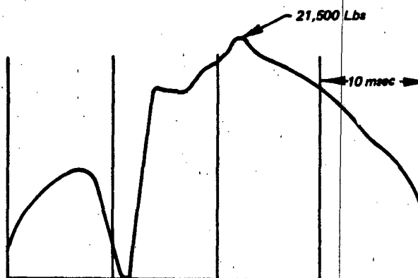
c) Reaction Time-Load History
