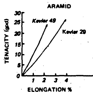
Figure 4.2 (Cont'd) Tenacity vs Elongation of Textile Fibers
