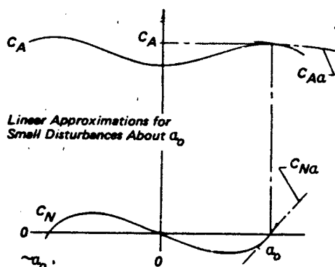
Figure 7.41 Typical Variation of Parachute Force Coefficients with a
