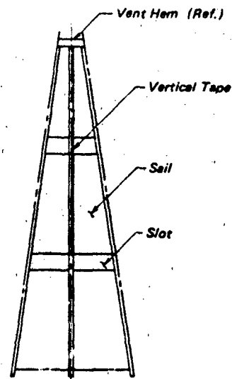
Figure 8.3 Typical Crown Slot Control Tape on Circular Canopies
