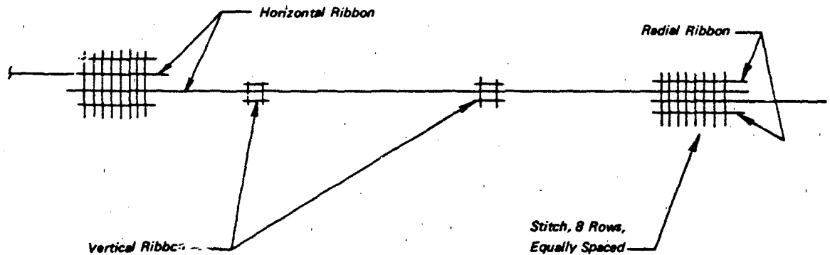
Figure 4.17 Cross-section of a Typical Ribbon Canopy Gore
