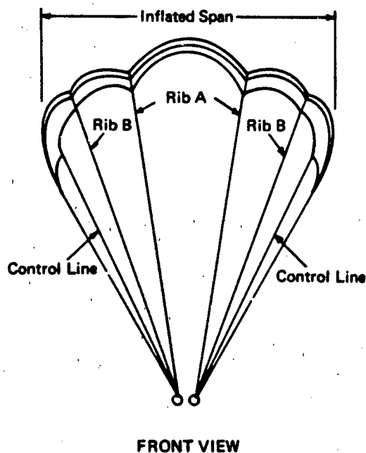
Figure 2.8 Sailwing
