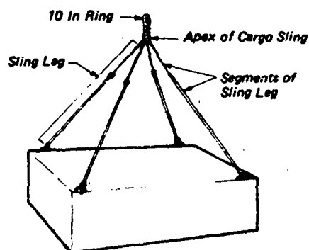
Figure 3.38 Representative Cargo Harness Assembly
