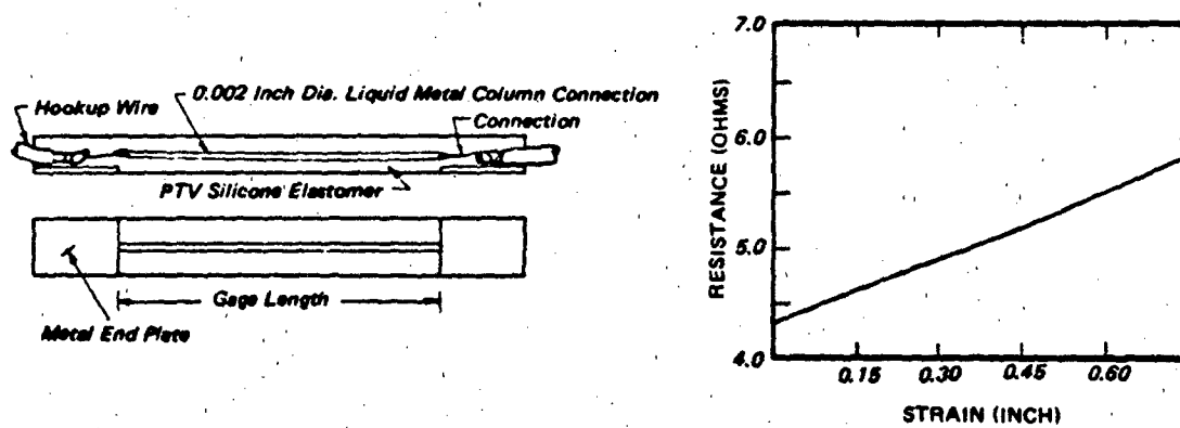
Figure 5.30 Details and Calibration of Elastomeric Strain Gauge
