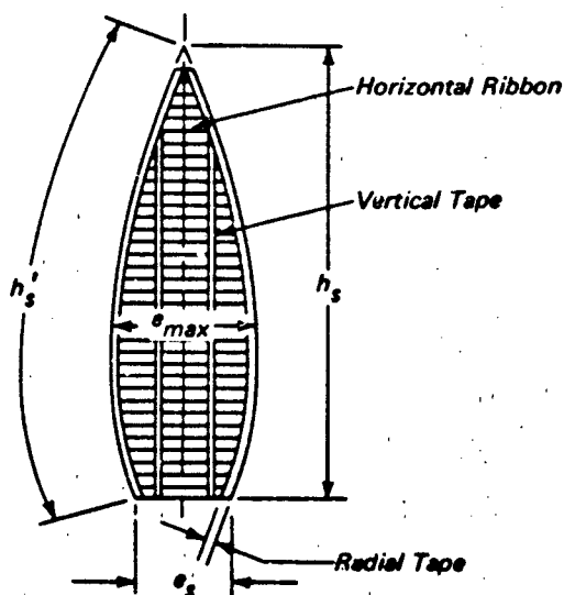
GORE LAYOUT
