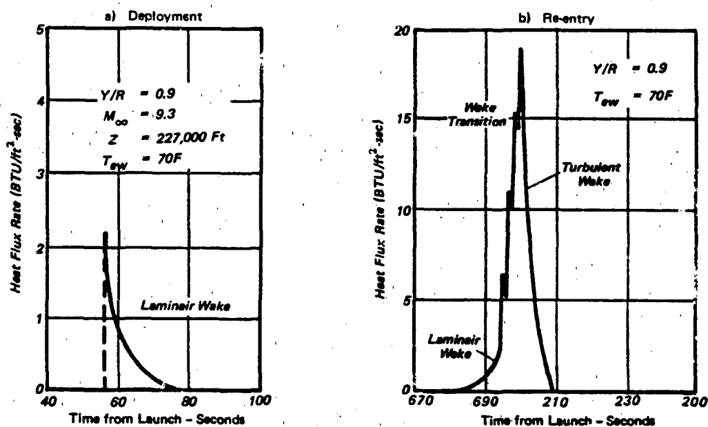
Figure 7.33 Ballute Cold Wall Heat Flux Rate (Test TB - 4)
