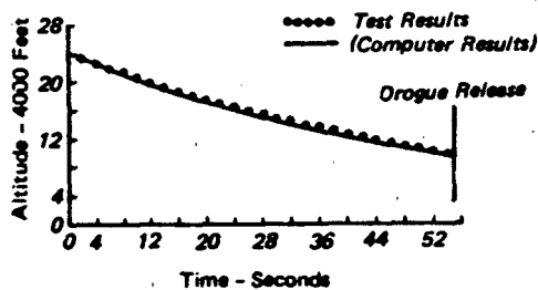
c) Vehicle Altitude Vs Time. Computer and Test Results. (Twin Drogue)
