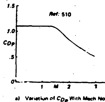
Figure 7.13 Measured and Predicted Characteristics of Disk-Gap-Band Parachute
