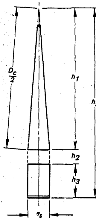
GORE LAYOUT
