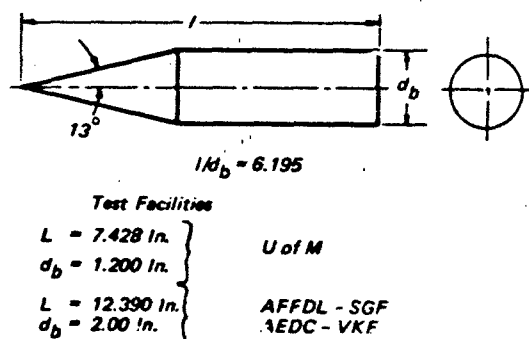
Figure 7.37 Geometry of Bodies Used for Experiments
