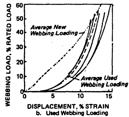
Figure 6.4A Relative Load-Flongation of Nylon Webbing from Twice Repeated Static Tests
