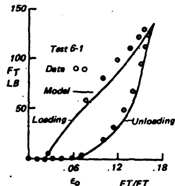
d) Worst First Cycle Load-Elongation Simulation
