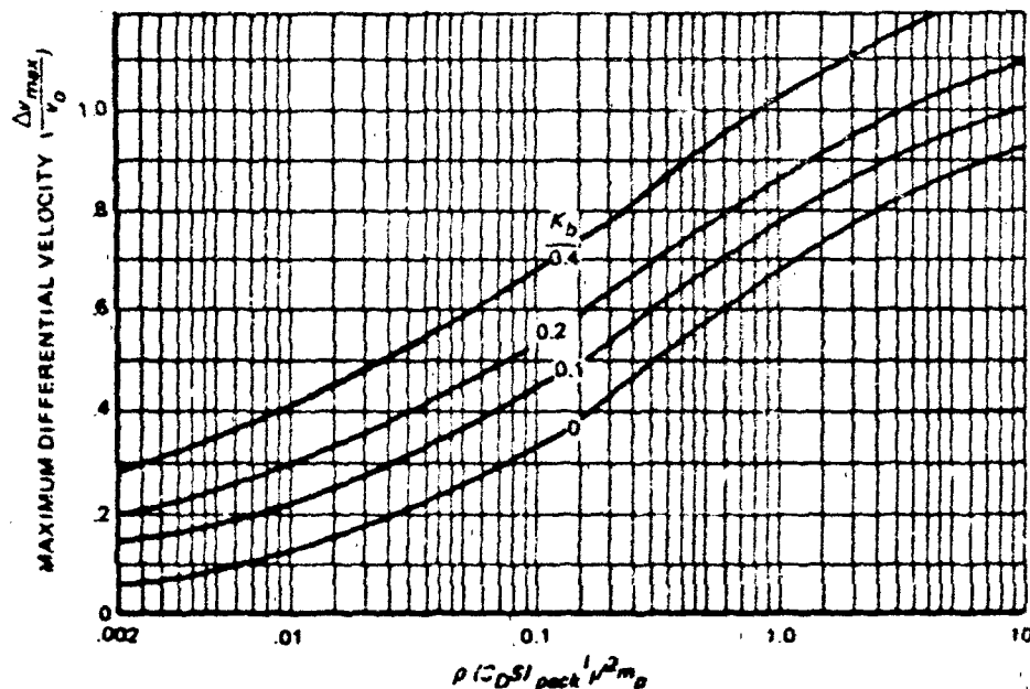
Figure 6.5 Approximate Body-Canopy Separation Velocity at Line-Stretch
