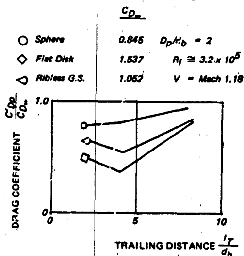
Figure 6.51 Drag Coefficient of Small Rigid Models in Wake of Simulated Ogive-Cylinder (Adapted from Ref. 433)
