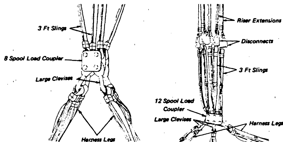
Figure 3.45 Typical Installation with Load Coupler and Large Clevises
