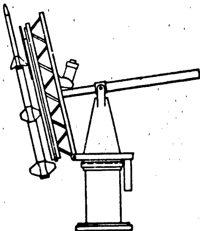
Figure 5.5 Test Vehicle Launch From Ground
