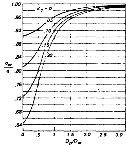
Figure 7.36 Average Dynamic Pressure on Decelerator in Body Wake
