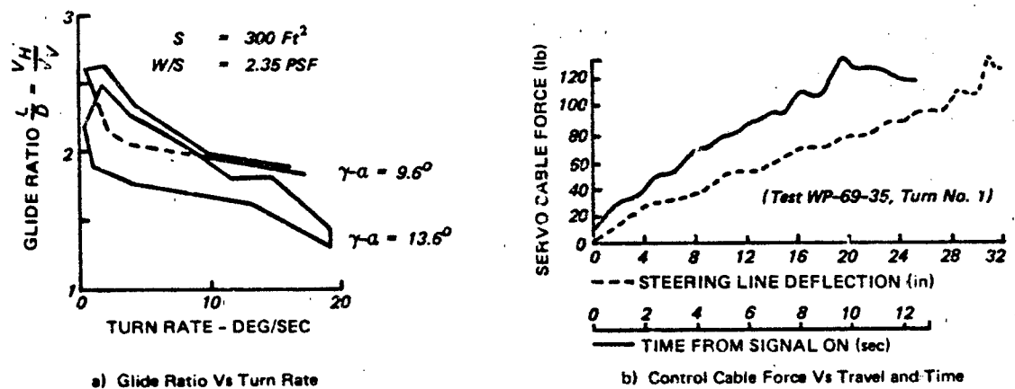
Figure 6.38 Parafoil Measured Turning Characteristics (Ref 132)
