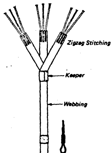
Figure 4.26 Branched Riser With Stitched Line Joints
