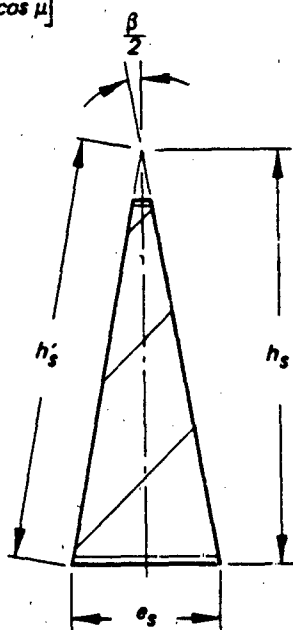
GORE LAYOUT
