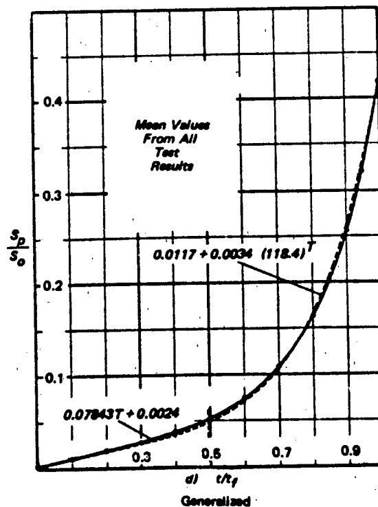
Figure 6.10A Normalized Canopy Area Growth During Inflation of 28 Ft ( D_0 ) Solid Flat Circular Parachute
