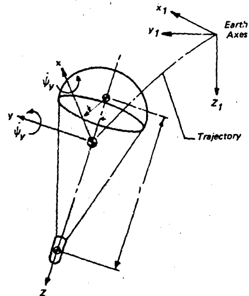
Figure 7.40 Parachute System Geometry and Coordinate System
