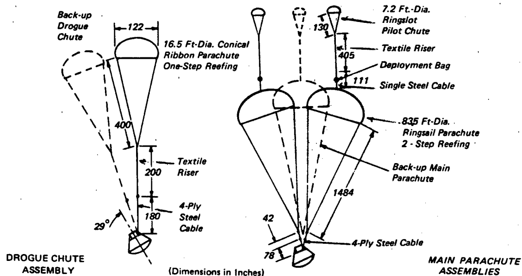
Figure 1.11 Apollo Drogue And Main Parachute Assemblies
