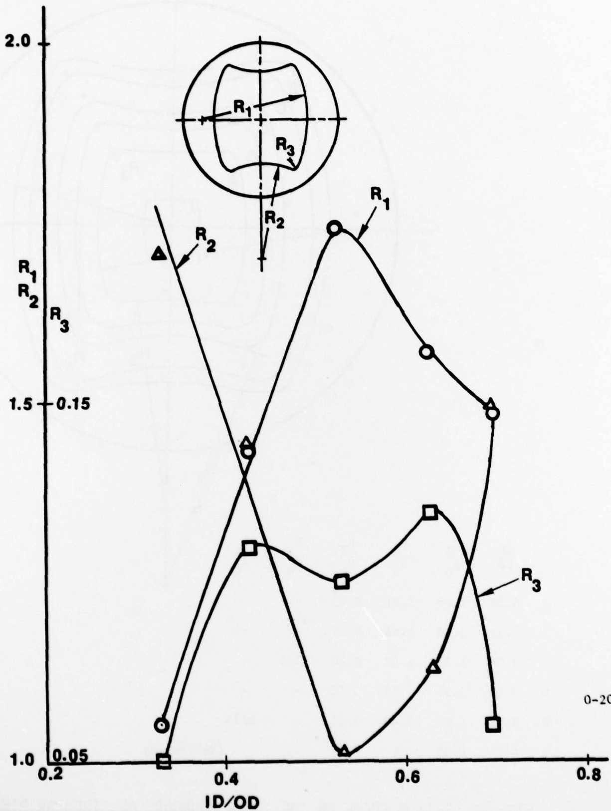
FIG. 6 RADII OF THE ELEMENTS OF HOLES PRODUCING OPTIMUM DISTRIBUTION OF STRESS IN CIRCULAR RINGS UNDER DIAMETRAL COMPRESSION.
