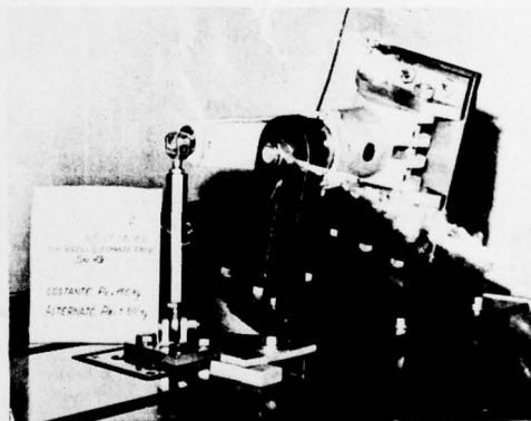
Fig. 18 - Static and fatigue test of Spacelab structure.
