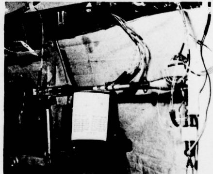
Fig. 19 - Typical fatigue tests of helicopter dynamic components at Agusta fatigue laboratory.
