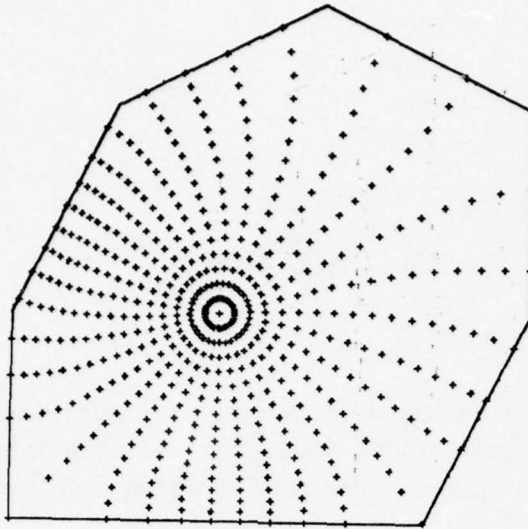
(a) 7-sided problem domain, including image of 16 \times 32 finite-difference grid in the unit disk
