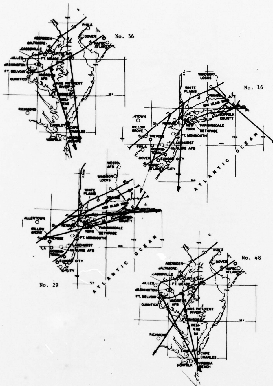
Fig. 2-1c. Angle-of-Arrival Rays for Unidentified Interrogators 16, 29, 48 and 56.
