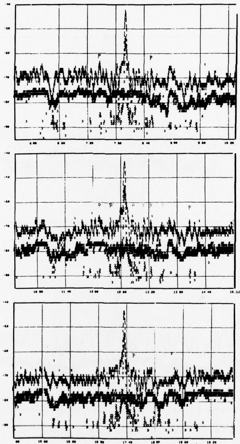
Fig. 3-2a. Antenna Pattern, Composite - Philadelphia (ASR-7), 6.00-19.20 Secs.
