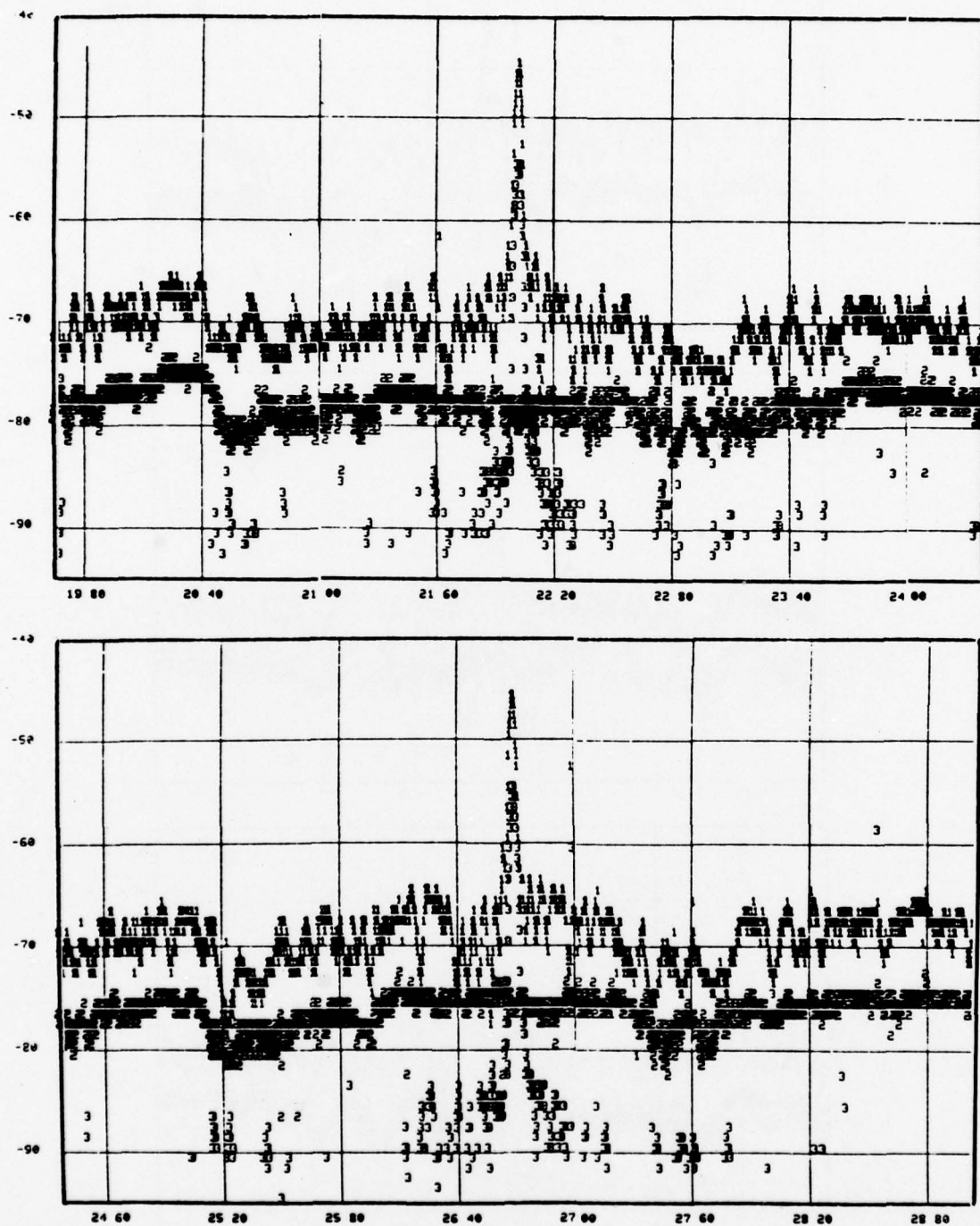
Fig. 3-2b. Antenna Pattern, Composite - Philadelphia (ASR-7), 19.80-28.80 Secs.
