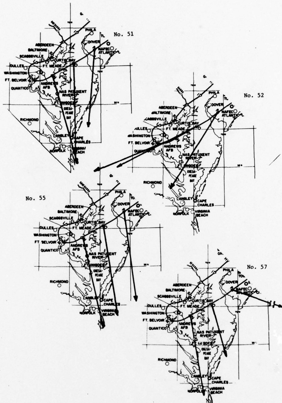
Fig. 2-ld. Angel-of-Arrival Rays for Unidentified Interrogators 51, 52, 55 and 57.
