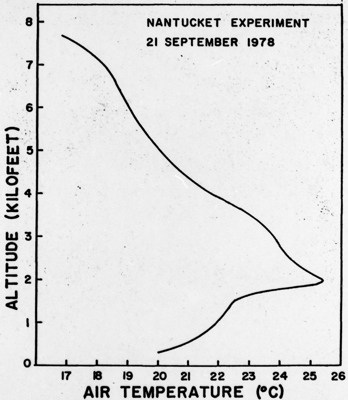
FIG.1 TEMPERATURE PROFILE
