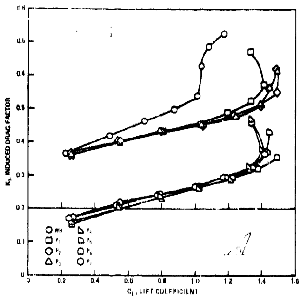
Figure 46c - Canard C_2
