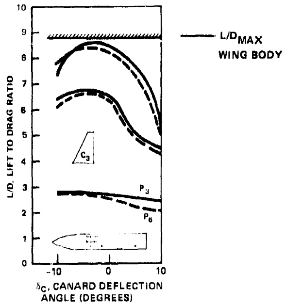
Figure 49d - Canard C_3 on 50-Degree Wing
