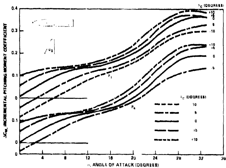
Figure 32d - Canard C_3 on 50-Degree Wing
