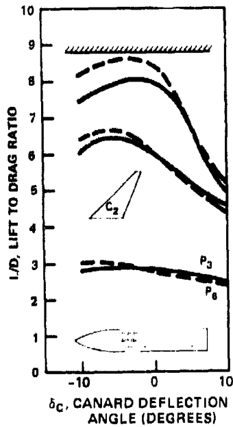
Figure 49c - Canard C_2 on 50-Degree Wing
