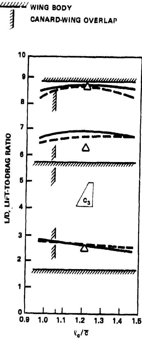
Figure 44d - Canard C_3 on 50-Degree Wing
