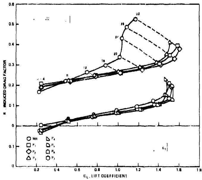
Figure 46b - Canard C_1
