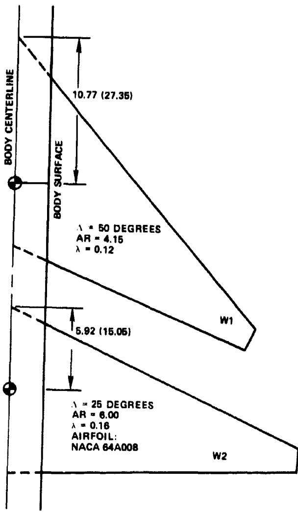
Figure 59 - Planform View of the Wings
