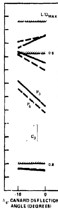
Figure 49e - Canards on 25-Degree Wing
