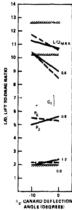
Figure 49e - Canards on 25-Degree Wing
