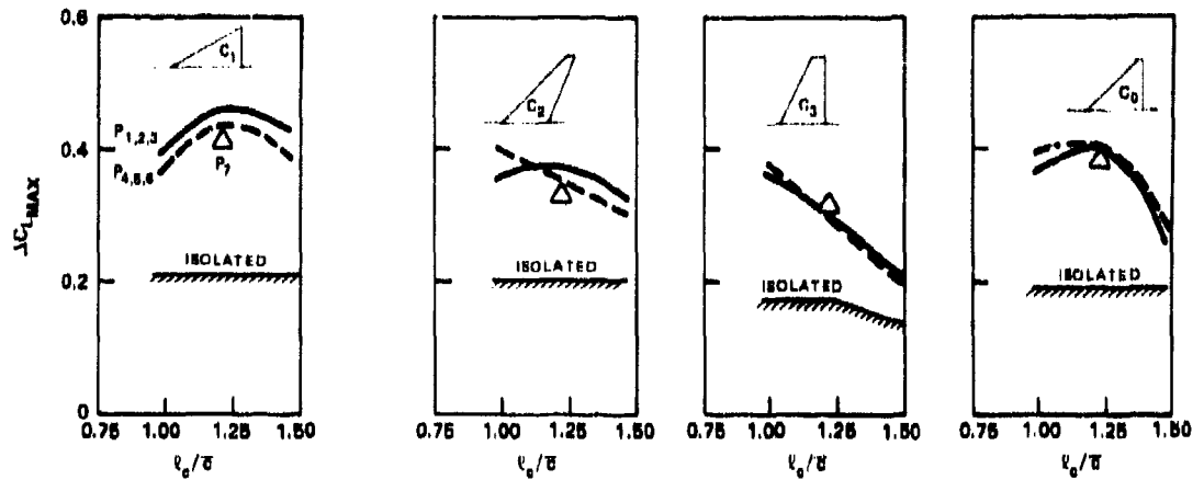
Figure 10a - Lift on 50-Degree Wing
