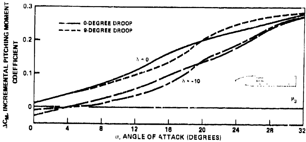
Figure 36a - Position 3
