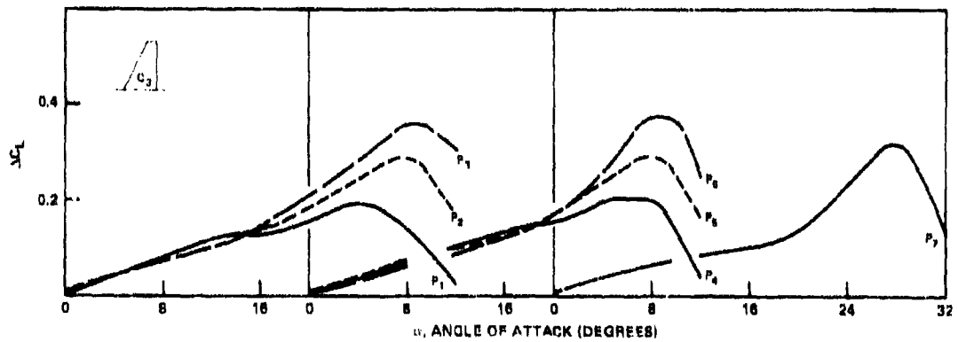
Figure 9d - Canard C_3 on 50-Degree Wing
