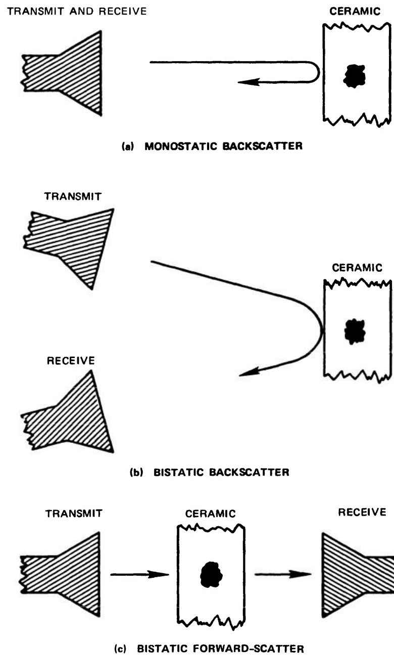
FIGURE 3 SCATTERING CONFIGURATIONS
