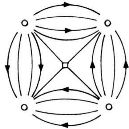
(b) QUADRIPOLE MODE
