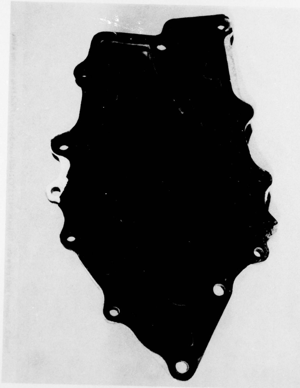
Figure 1. Aluminum water pump after 555 hours at 115.5°C (240°F) with 1.5-percent 0-I-490 Corrosion Inhibitor in corrosive water.
