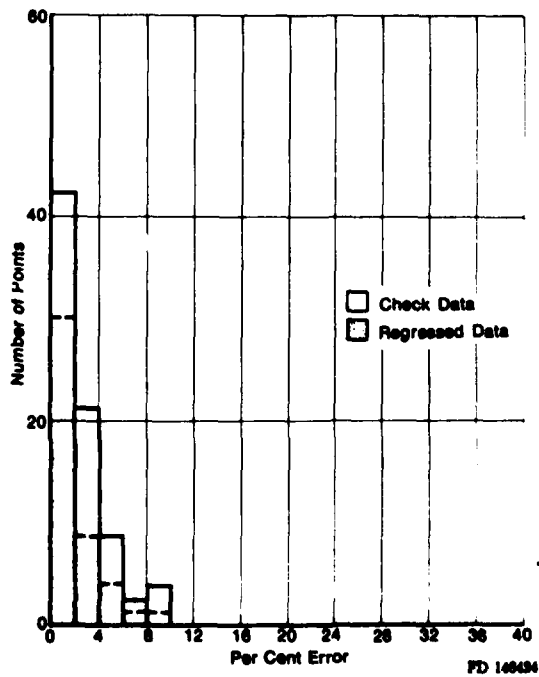
Figure 26. TOGW Error Distribution — Log Transformation 6 Variables, Half Replication
