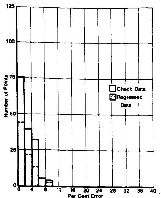
Figure 28. TOGW Error Distribution — Log Transformation 7 Variables, Half Replication
