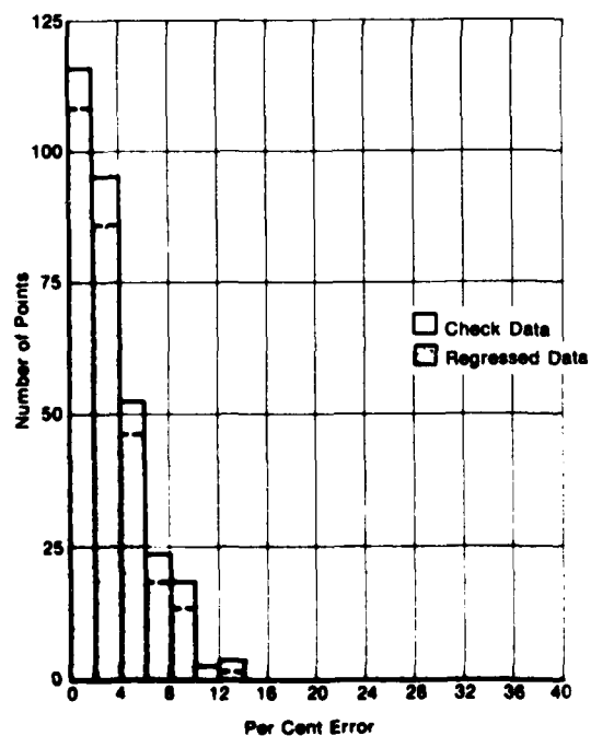
Figure 30. TOGW Error Distribution — Log Transformation 8 Variables, Half Replication
