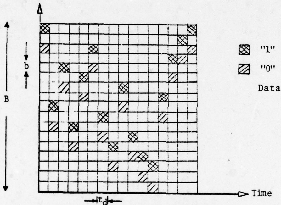
FIG. 1. FREQUENCY-TIME DIAGRAM OF A FH SYSTEM
