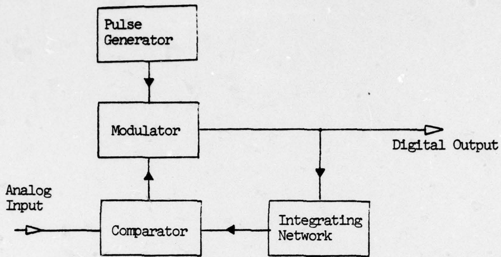
FIG. 5. BASIC DELTA MODULATION
