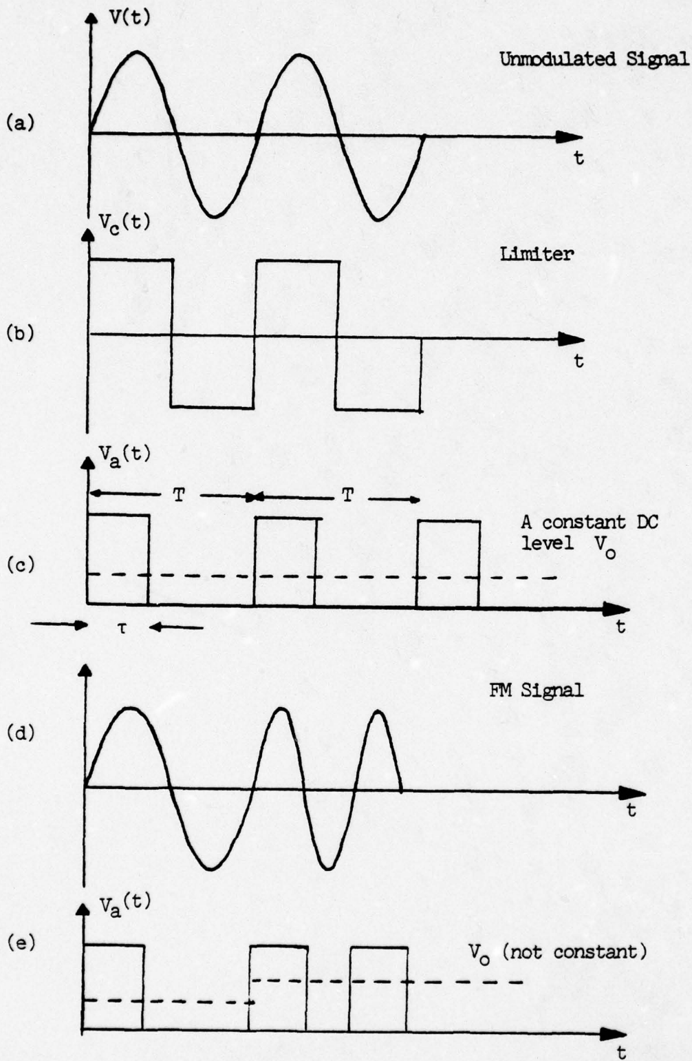
FIG. 19. PCD OPERATION
