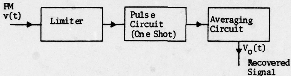
FIG. 18. PULSE COUNTING DISCRIMINATOR
