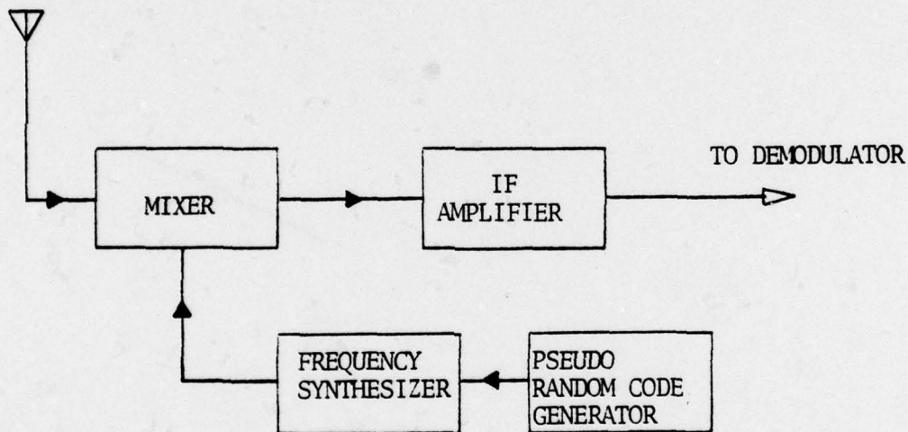
FIG. 3. A FH RECEIVING SYSTEM
