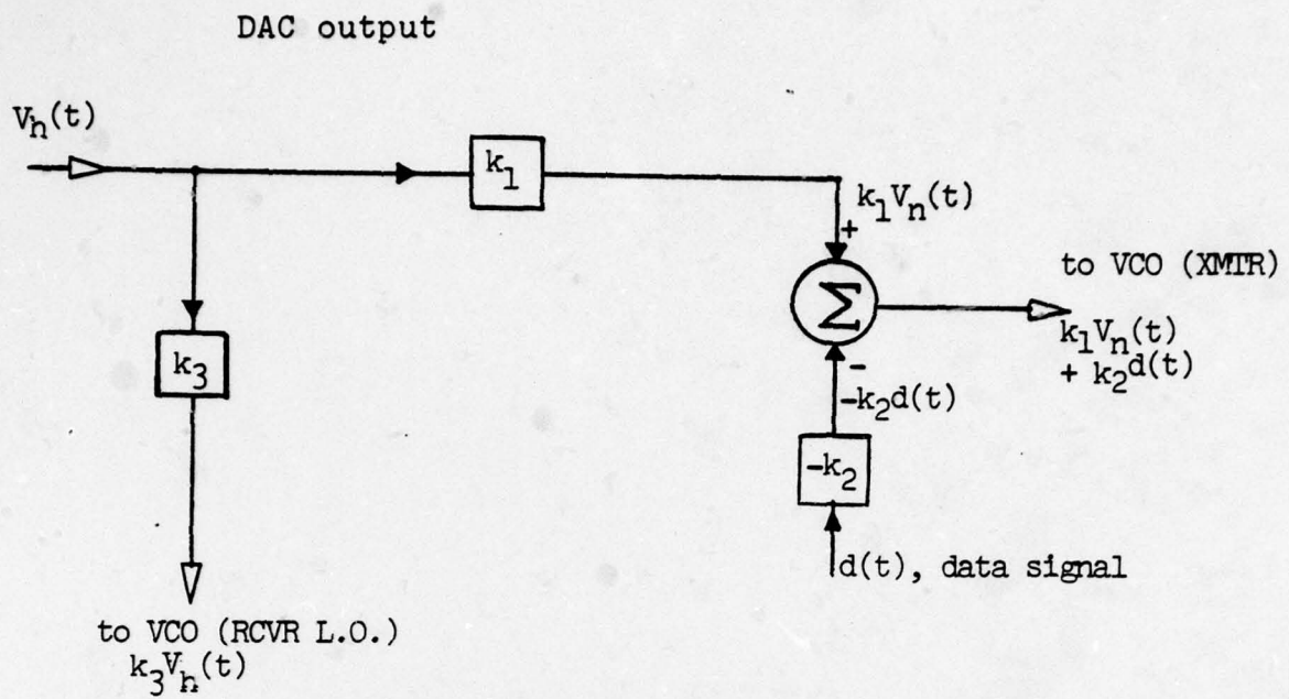
FIG. 15. MODULATION NETWORK BLOCK DIAGRAM
