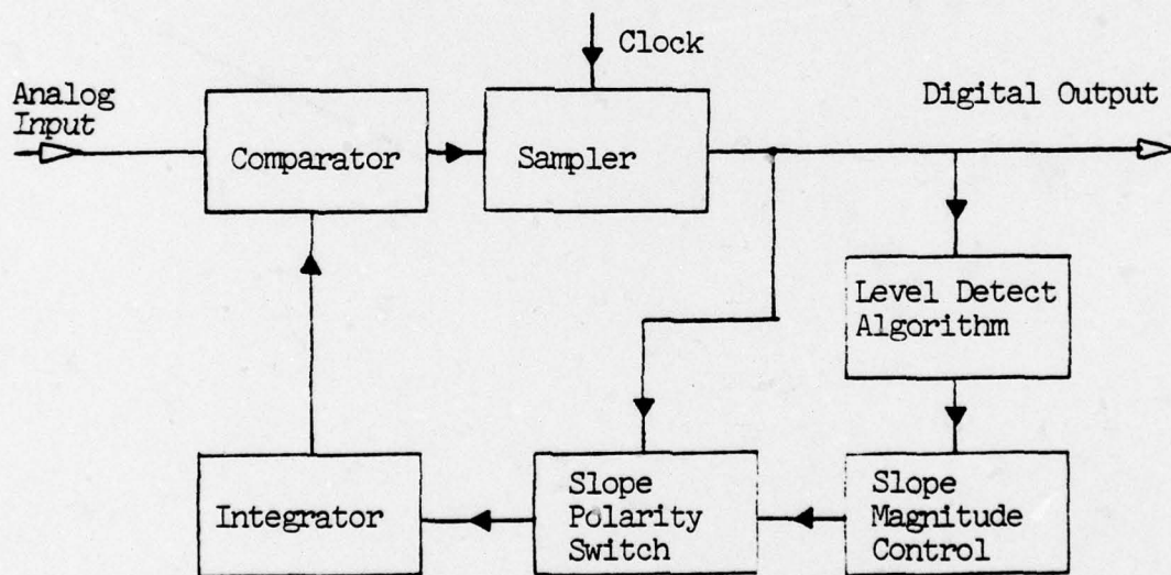
FIG. 6. CVSD MODULATOR BLOCK DIAGRAM
