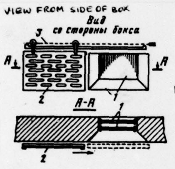
Fig. 9.2. Schematic diagram of armored shield for protecting observation booth windows: 1--armored observation booth; 2--retractable armored shield with slits; 3--cable of mechanism for moving armored shield.
