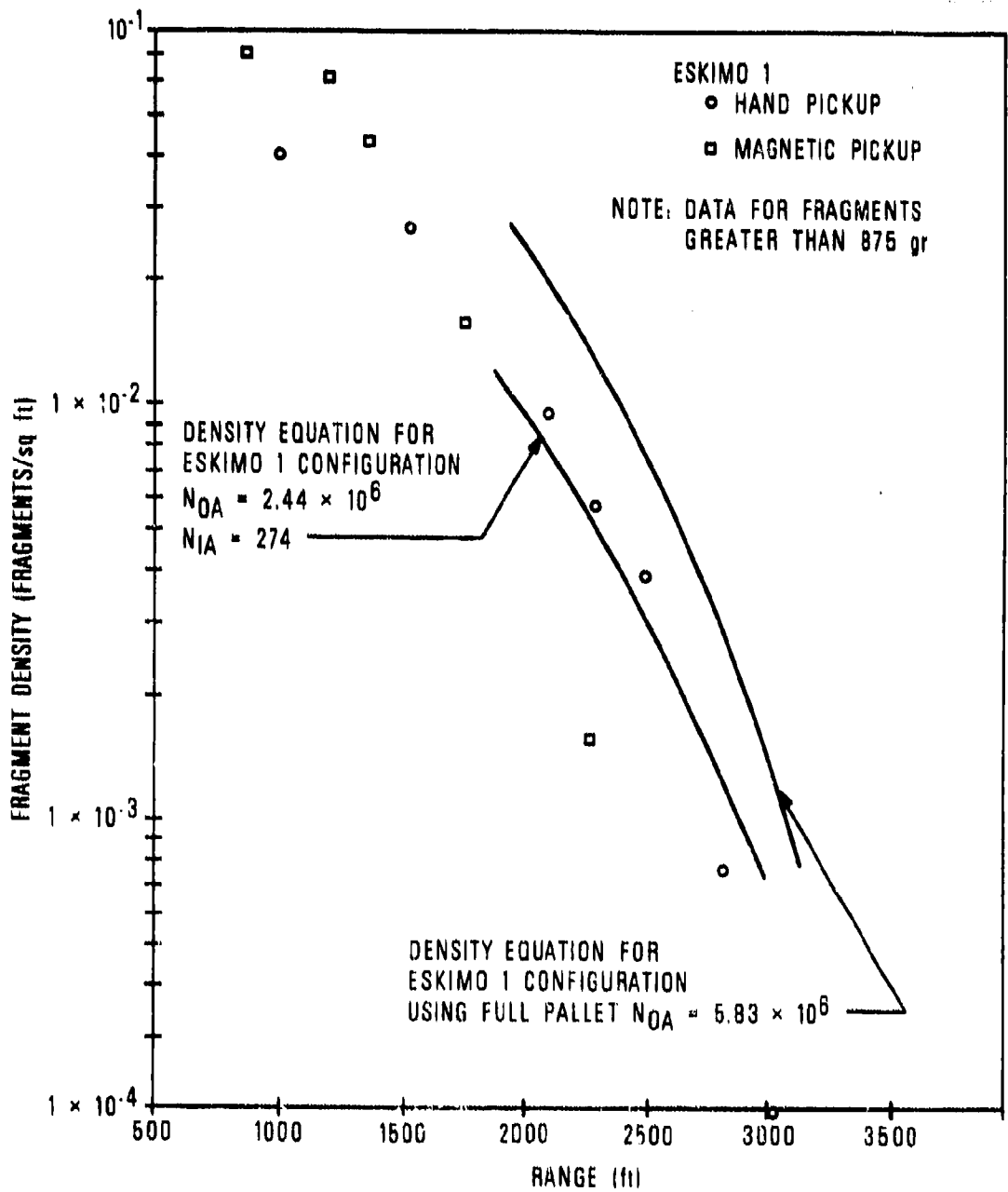
Figure 58. Far-Field Fragment Densities Versus Range for ESKIMO 1 and Test QD-155-08
