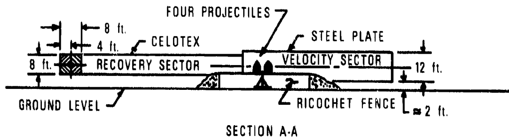
Figure 18. Azimuthal Arena Layout for Test No. QD-155-10 (Firing No. 1)
