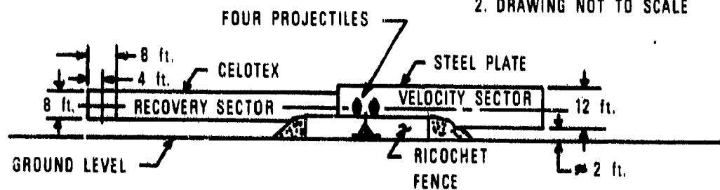
Figure 20. Azimuthal Arena Layout for Test No. QD-155-10 (Firings No. 2 and 3)
