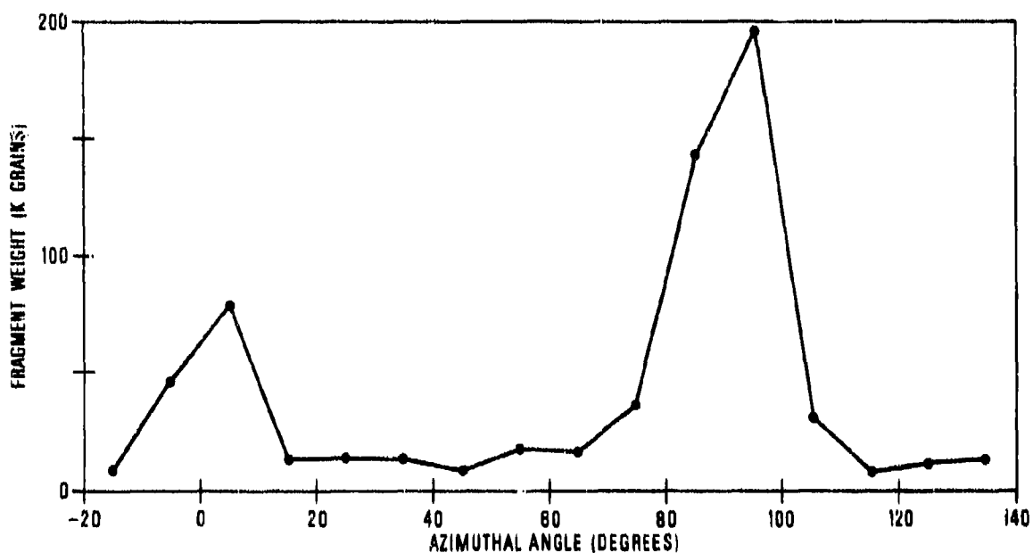
Figure 47. Fragment Weight Versus Azimuth Angle for Test QD-155-12, Polar Zones 90^\circ - 100^\circ
