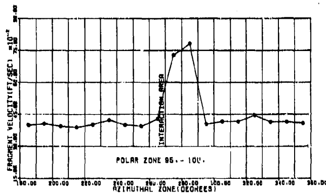
Figure 16. Fragment Velocities from Firing No. 2 for Test No. QD-155-09
