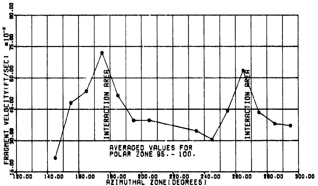
Figure 40. Average Fragment Velocities of all Firings for Test No. QD-155-10R (Polar Zone 95°-100°)
