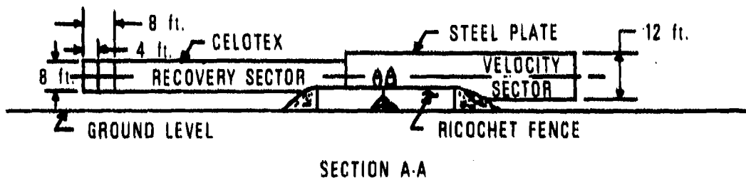
Figure 23. Azimuthal Angle Arena Layout for Test No. QD-155-12
