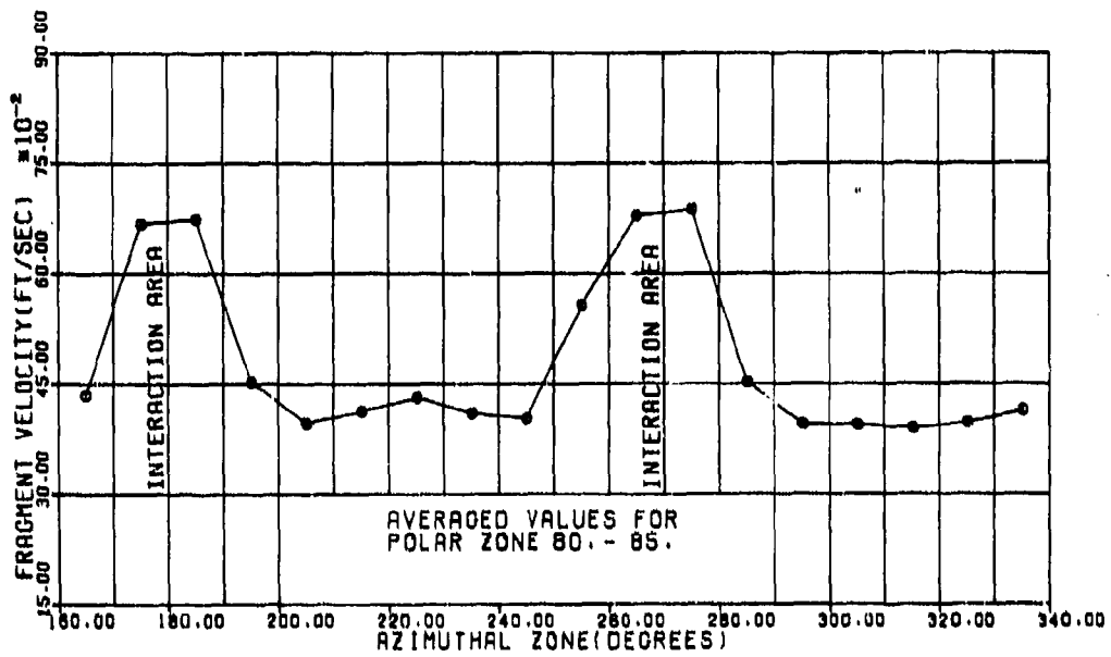
Figure 26. Average Fragment Velocities of all Firings for Test No. QD-155-12 (Polar Zone 80°-85°)
