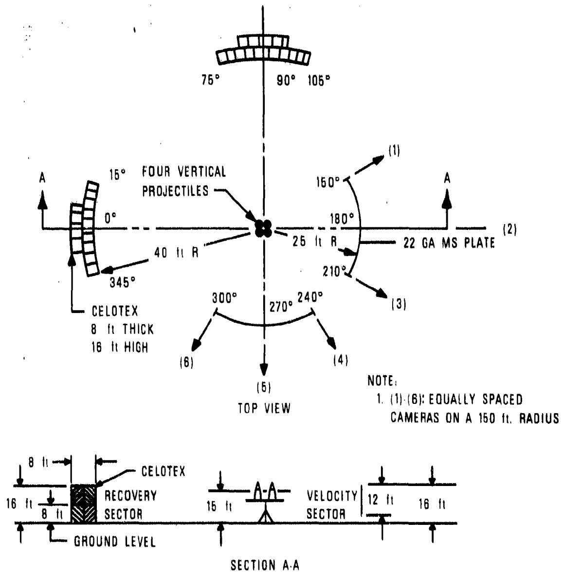
Figure 37. Azimuthal Angle Arena Layout for Test QD-155-10R
