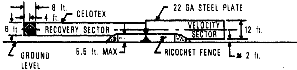
Figure 8. Pojar Angle Arena Layout for Test No. QD-155-03
