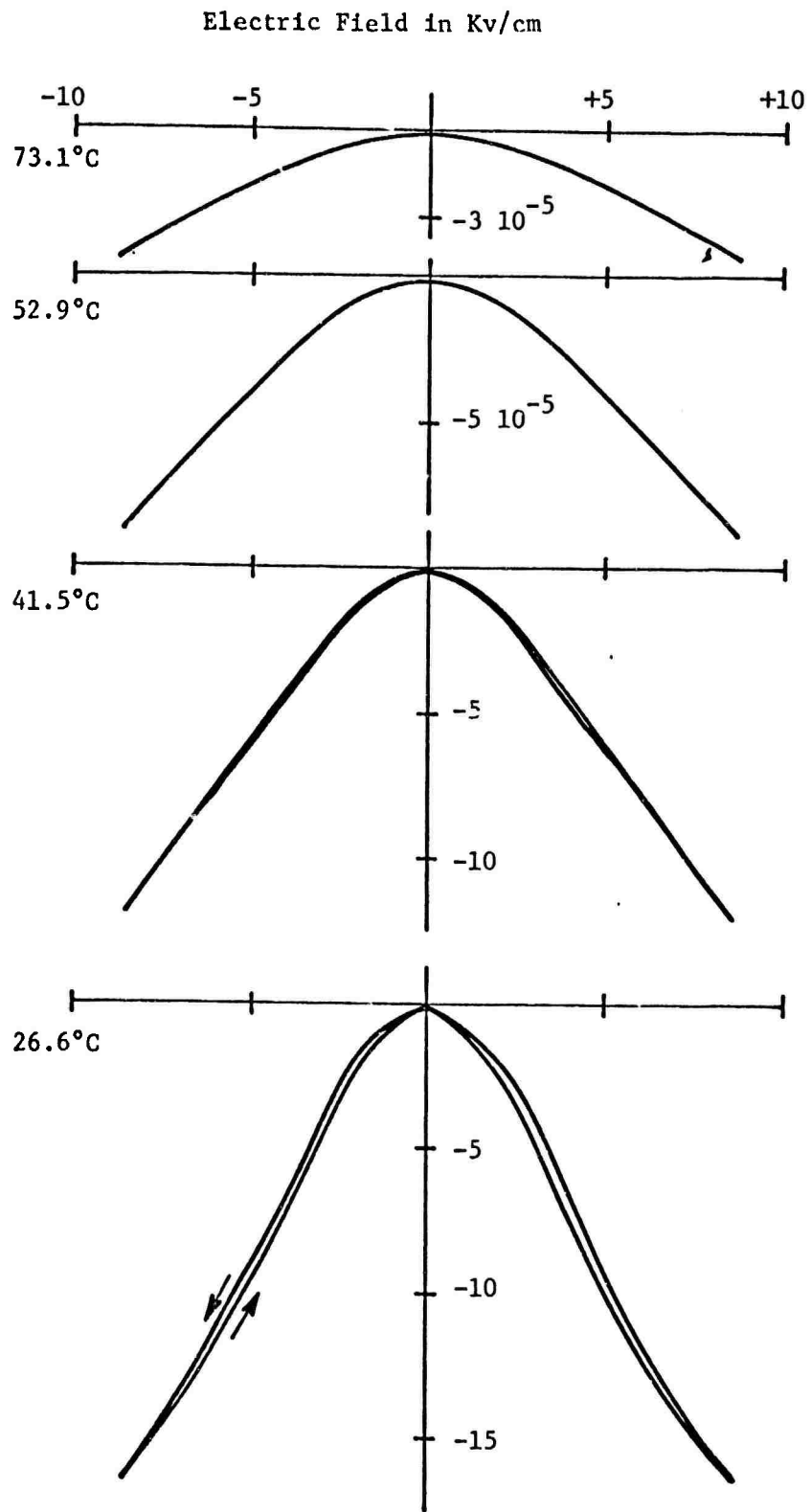
Figure 20(a) Transverse electrostrictive strain in 0.90 PMN:0.10 PT solid solution at various temperatures.
