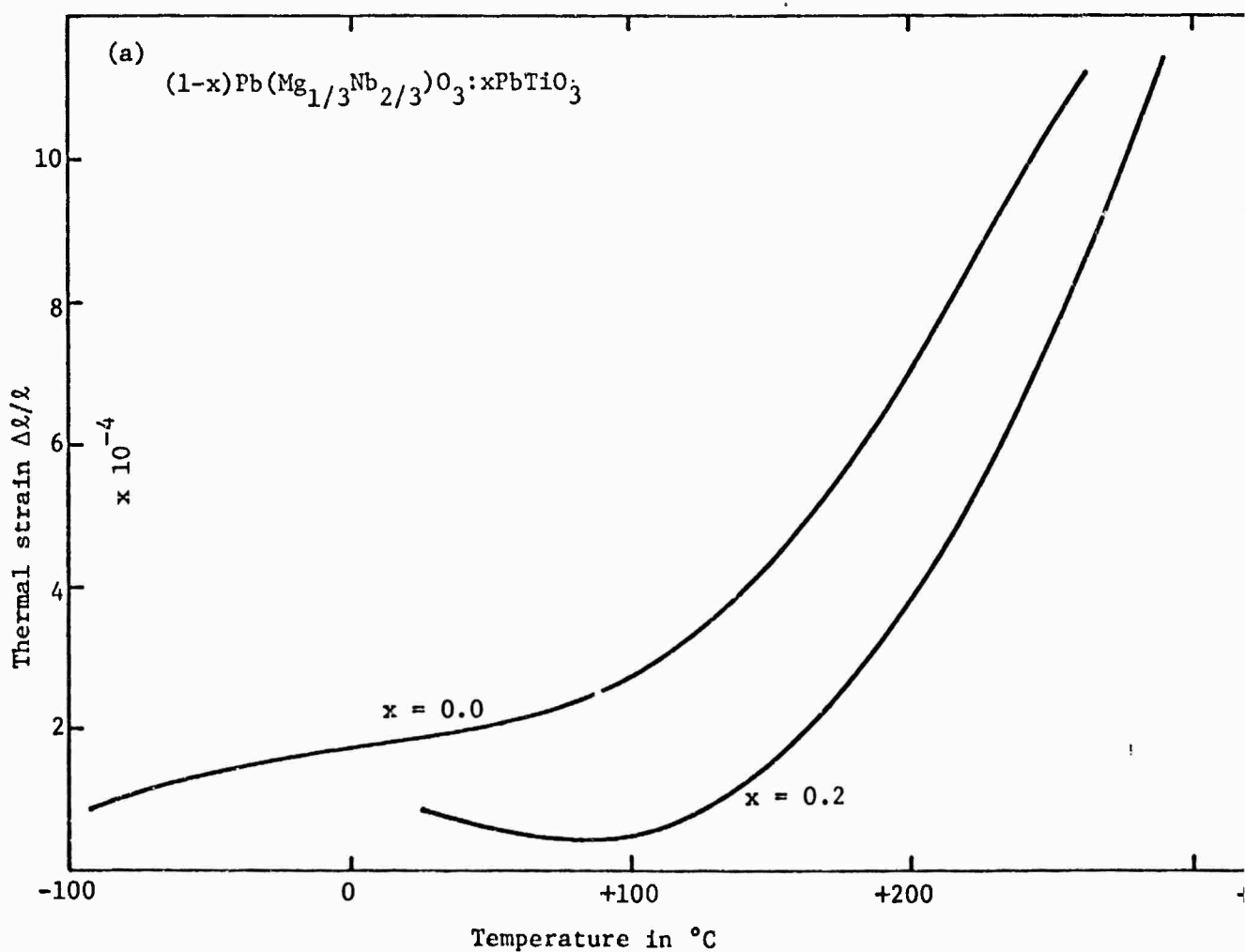
Figure 25. Thermal strain and thermal expansion coefficient \alpha in PMN:PT solid solutions.
