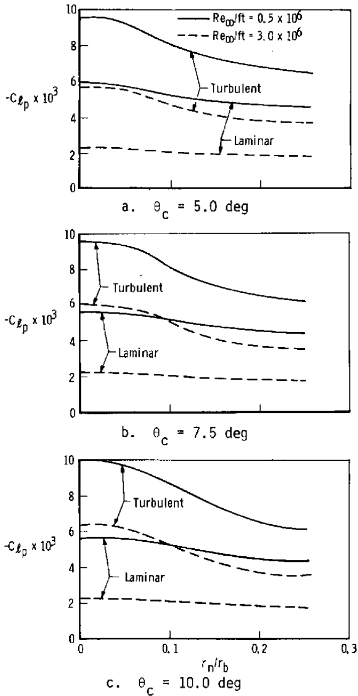
Figure 7. Roll-damping derivative versus bluntness for 5.0-, 7.5-, and 10.0-deg cones in Mach 10 flow.
