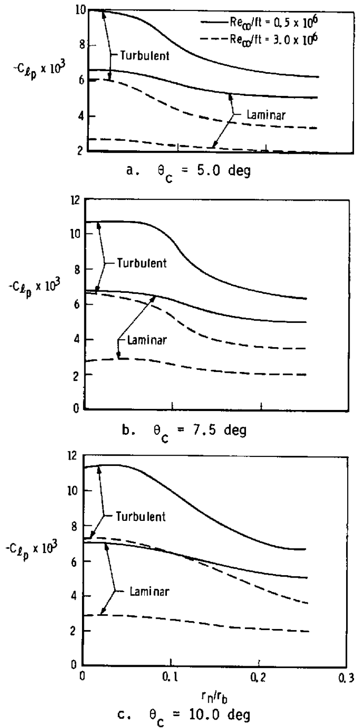
Figure 8. Roll-damping derivative versus bluntness for 5.0-, 7.5-, and 10.0-deg cones in Mach 14 flow.
