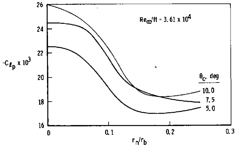
Figure 10. Roll-damping derivative versus bluntness for 5.0-, 7.5-, and 10.0-deg cones in Mach 22 flow at 200-kft altitude with laminar flow.
