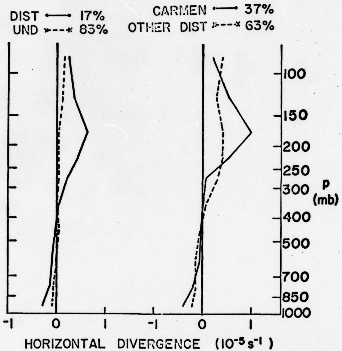
Figure 9. Same as Figure 8 except for divergence in units of 10^{-5} \text{ s}^{-1} .
