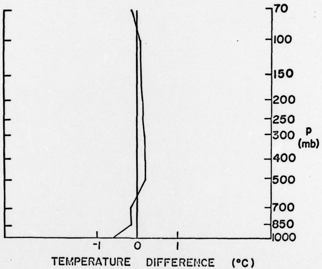
Figure 14. Vertical distribution of temperature difference between Carmen and the moving volume in units of °C.
