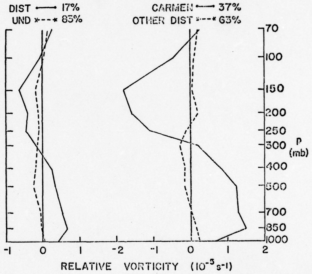
Figure 11. Same as Figure 8 except for relative vorticity in units of 10^{-5} s^{-1} .
