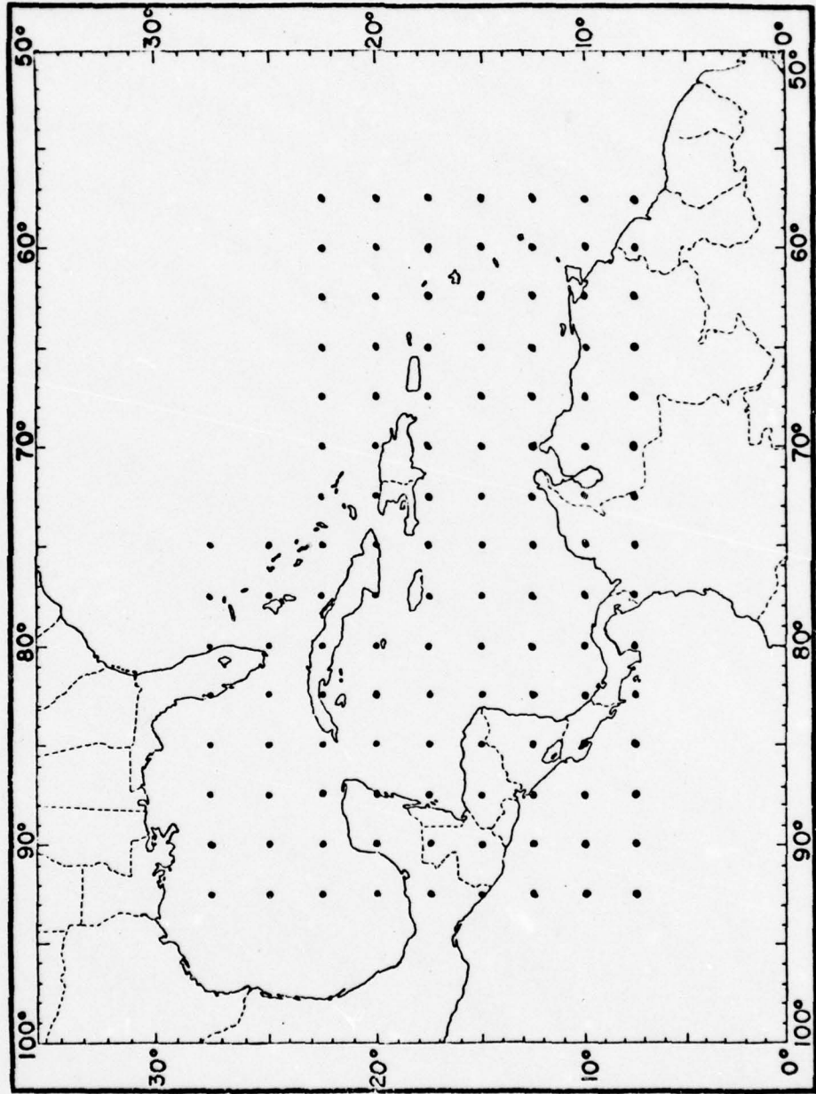
Figure 3. 2.5° latitude-longitude grid point array.
