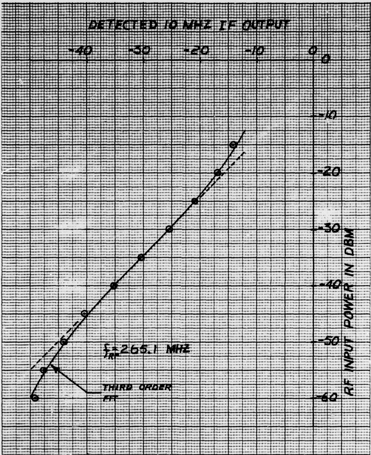
FIGURE 2. Sensor Subsystem Calibration Curve
