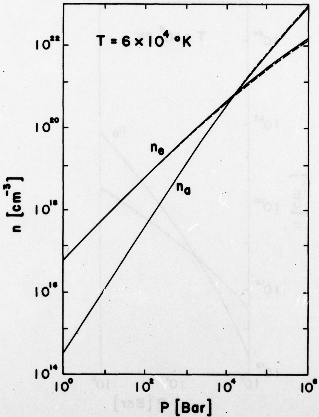
Fig. 5: n_e and n_a of H-plasma versus P for T = 6 \times 10^4 \text{ }^\circ\text{K} according to quantum statistical (—) and Saha (---) ionization equations.
