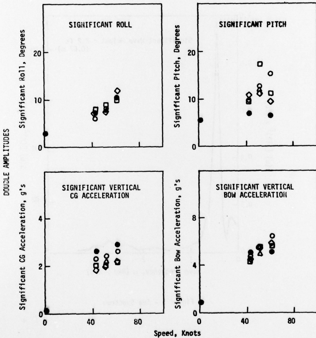
Figure 4 - Significant Double Amplitudes of Motions and Accelerations as a Function of Speed
