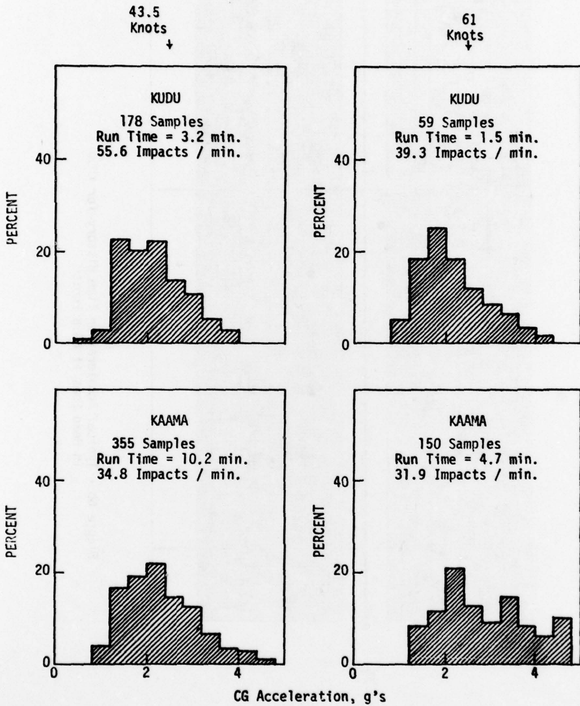
Figure 7 - Histograms of LCG Impact Accelerations
