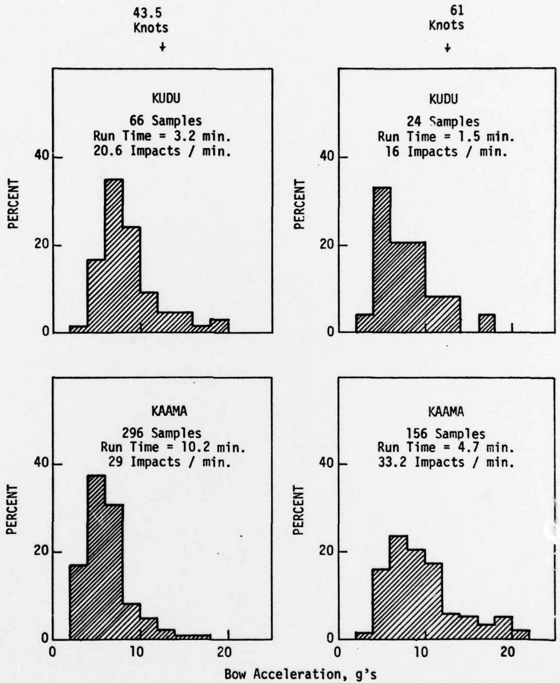
Figure 8 - Histograms of Bow Impact Accelerations
