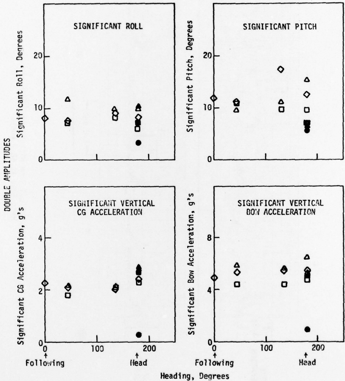
Figure 5 - Significant Double Amplitudes of Motions and Accelerations as a Function of Heading
