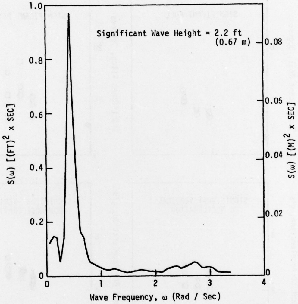
Figure 3 - Sea Spectrum
