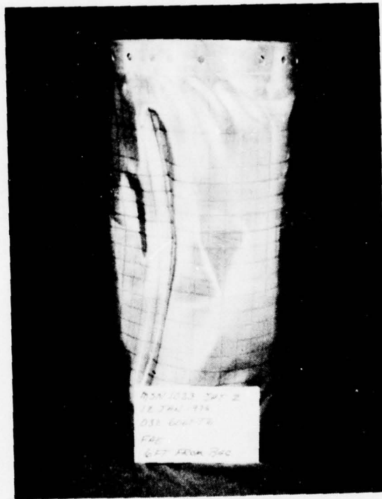
Figure 29. Cylinder for Data Point 24, Table II a/h = 188 L/D = 1.89
