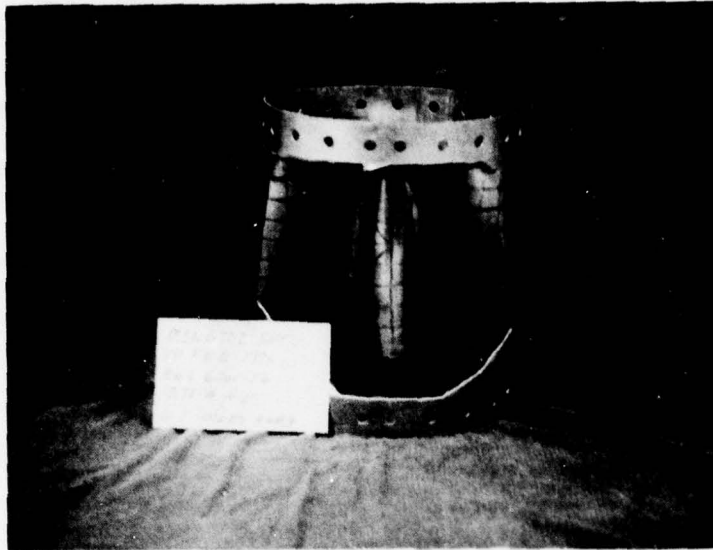
Figure 25. Cylinder for Data Point 20, Table II a/h = 95 L/D = 0.89
