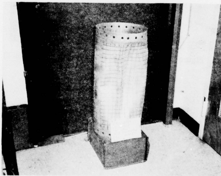
Figure 40. Cylinder for Data Point 35, Table II a/h = 85 L/D = 1.89
