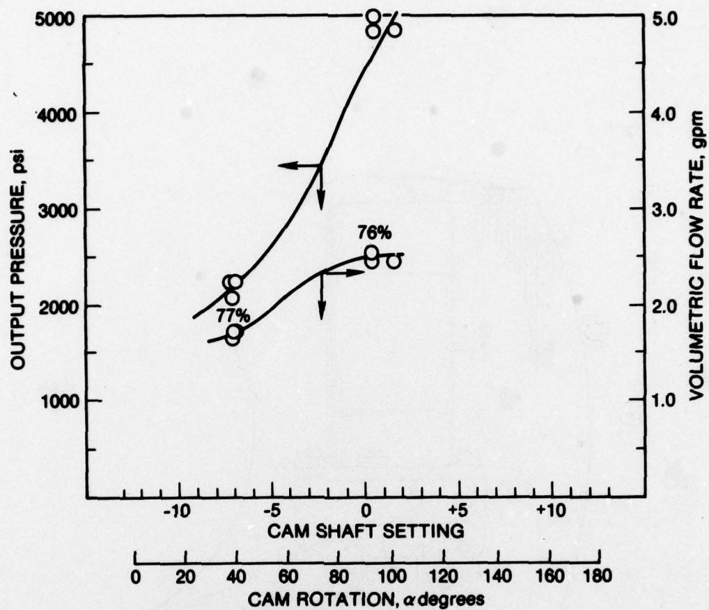
Figure 11. VD fuel pump performance (40-deg conical valve, 0.043-in. orifice), 5 May 1978.
