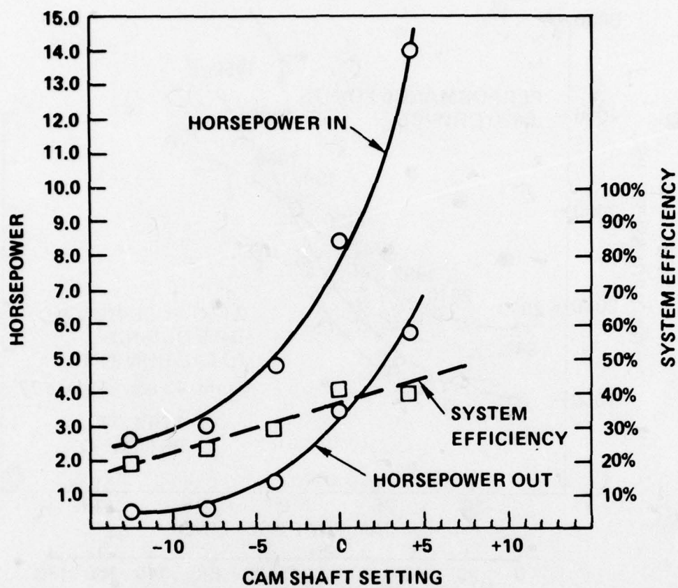
Figure 7. VD fuel pump energy analysis (40-deg conical valve, 0.0465-in. orifice).
