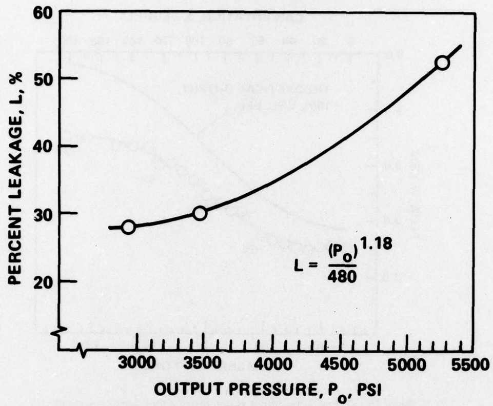
Figure 37. Internal leakage vs output pressure for 45-deg conical valve.
