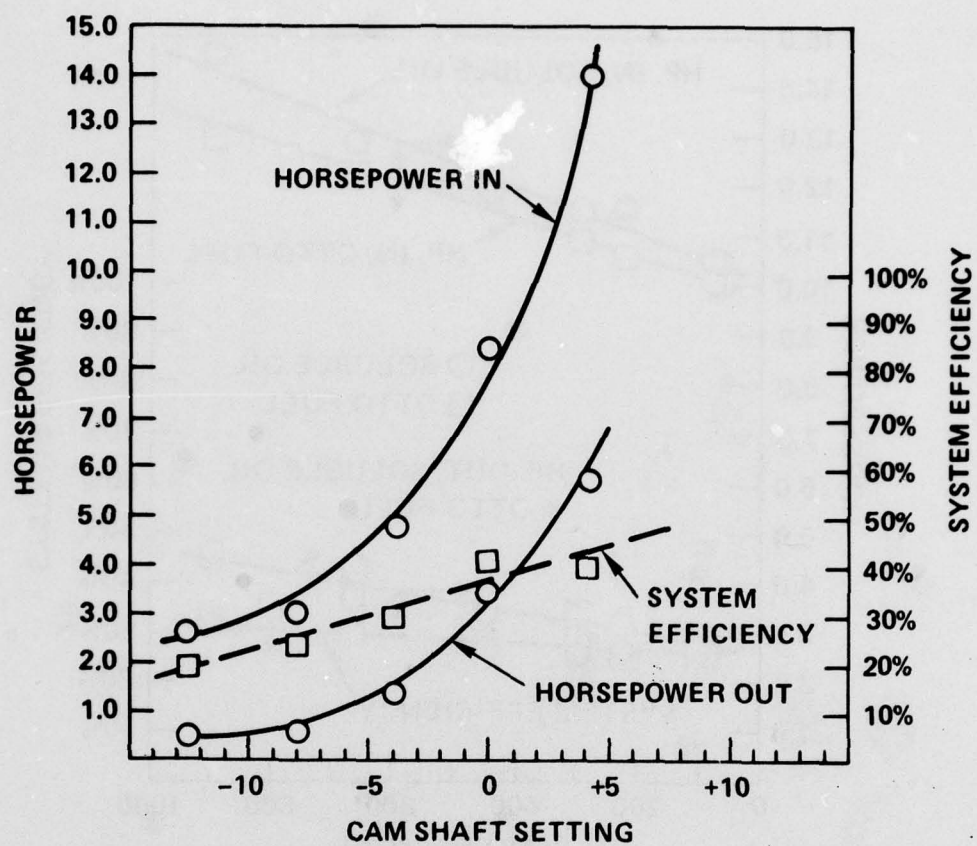
Figure 42. VD fuel pump energy analysis (40-deg conical valve, 0.0465-in. orifice).
