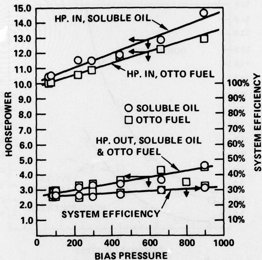
Figure 43. Equivalent fixed-displacement ALWT backup fuel pump No. 4 (0.038-in. orifice, 4100 rpm).
