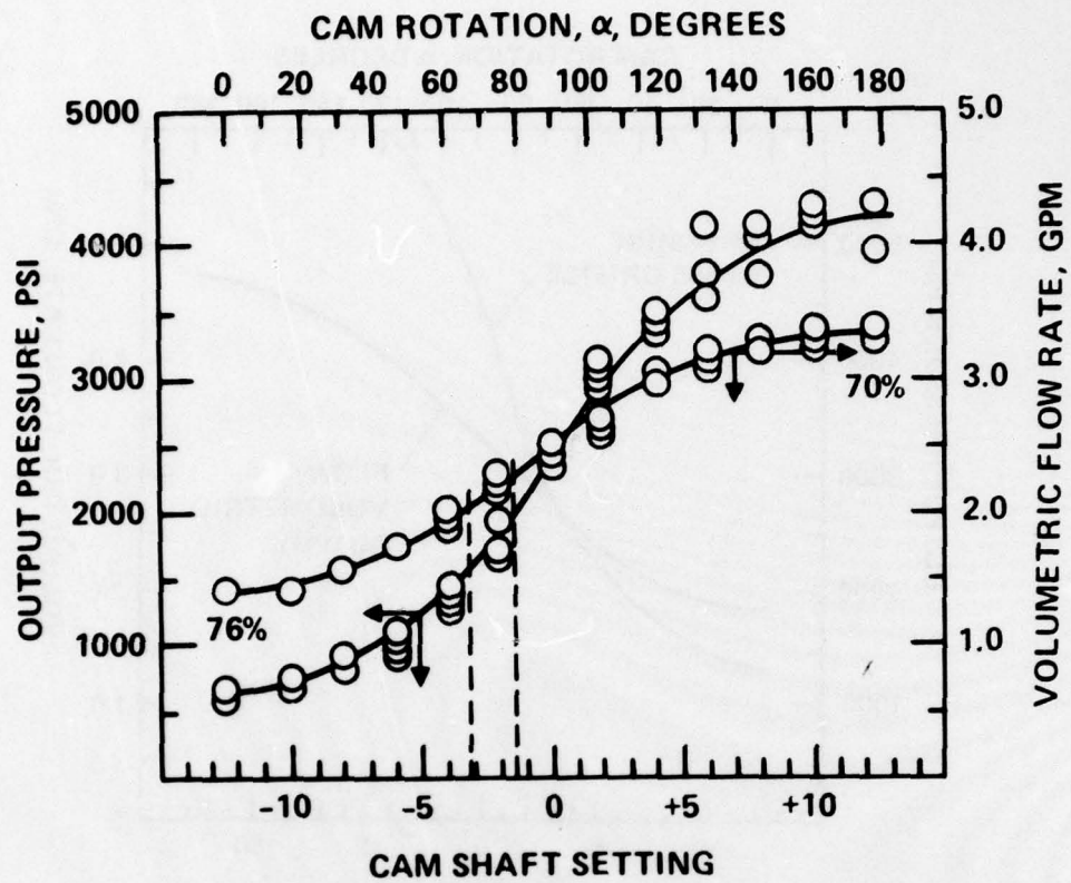
Figure 41. VD fuel pump performance (40-deg conical valve, 0.0465-in. orifice, C = 0.79 ).
