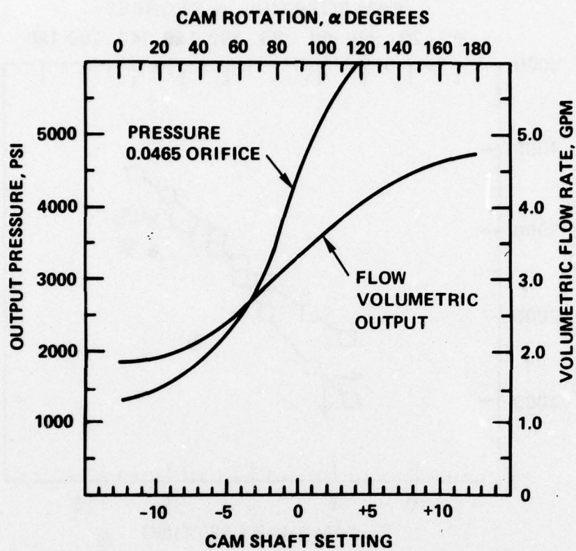
Figure 5. VD fuel pump performance (theoretical 100% efficiency).
