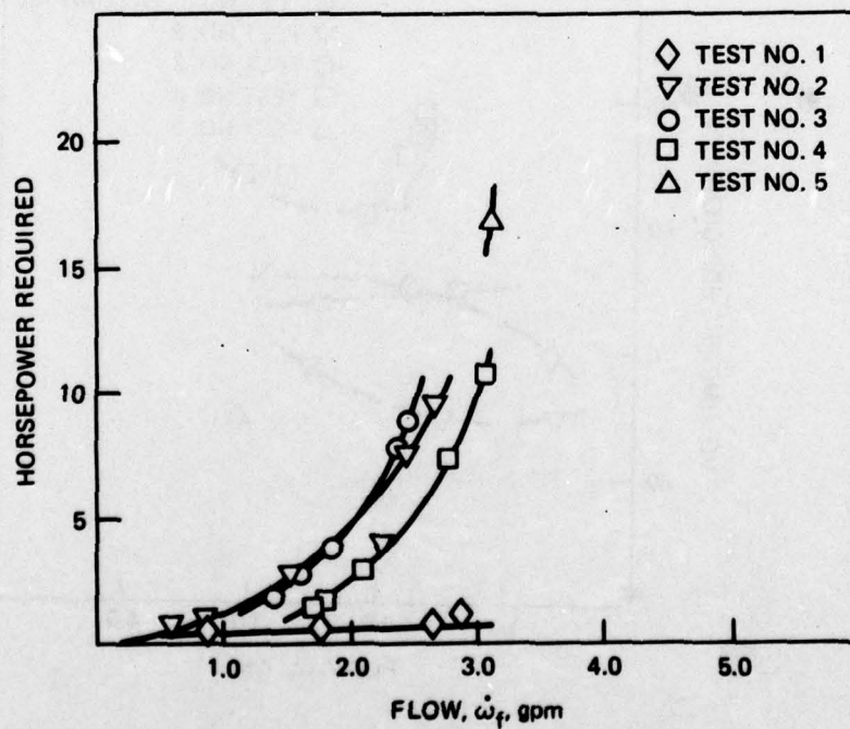
Figure 35. VD fuel pump performance, horsepower vs flow. Data of 20 June 1977.
