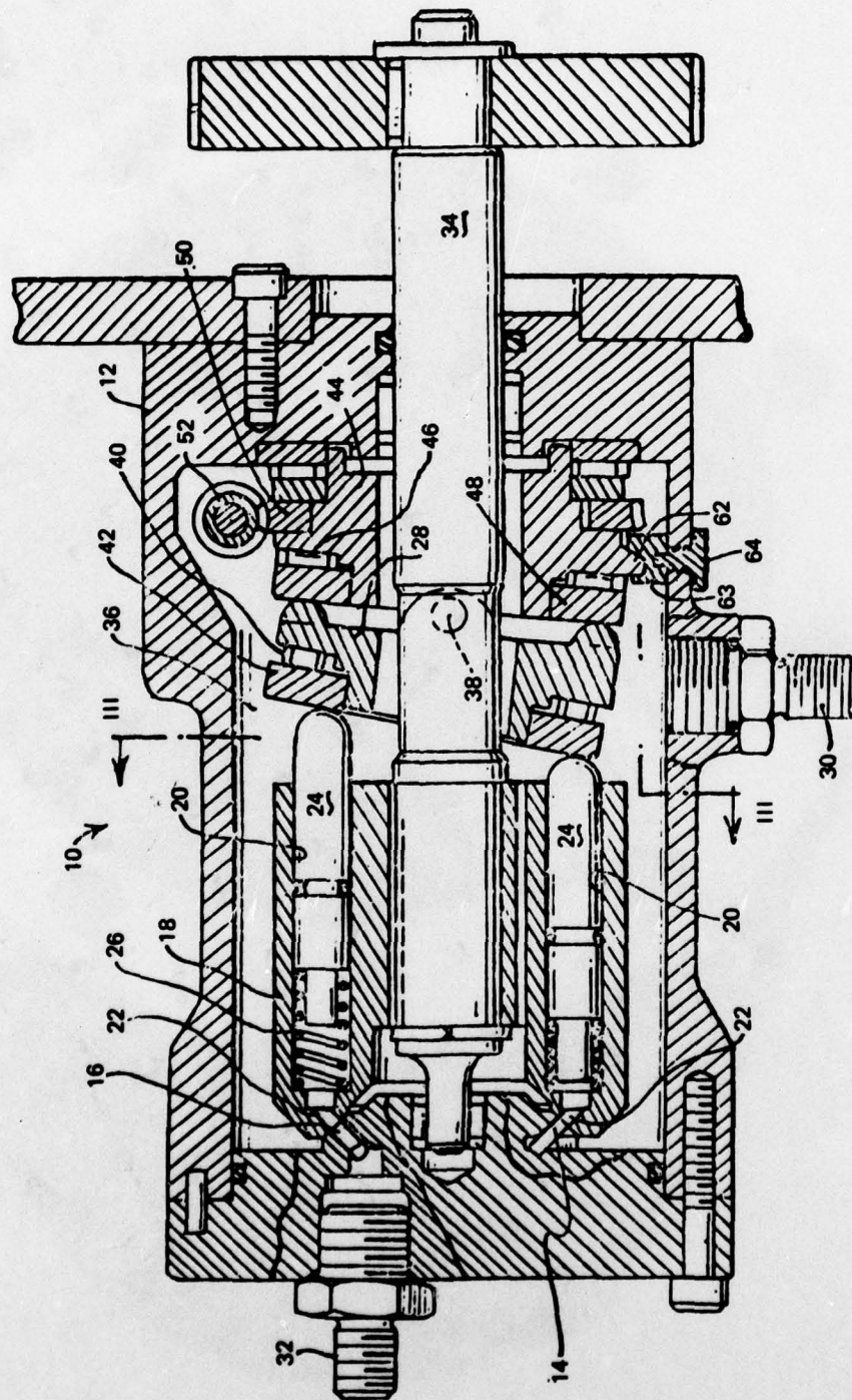
Figure 13. Cross-sectional-view of VD fuel pump.
