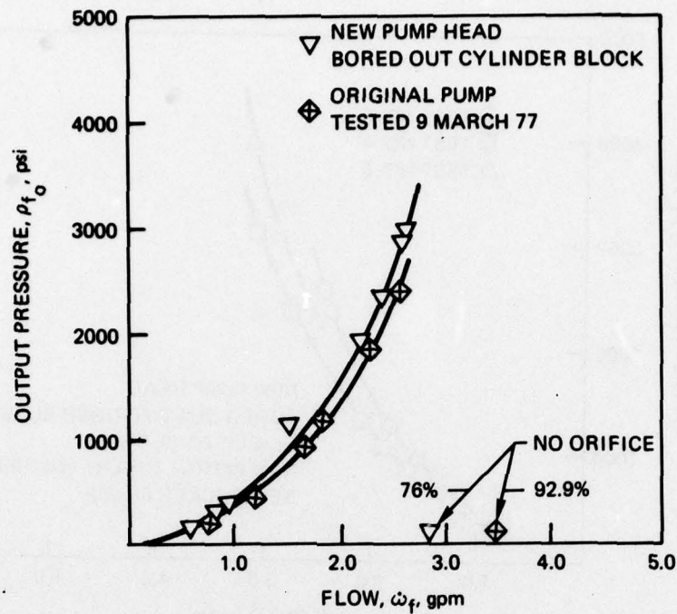
Figure 32. VD fuel pump performance (3- to 12-deg angle-plate, 0.052-in. orifice). Data of 20 June 1977.
