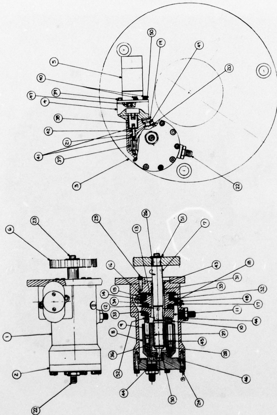
Figure 1. Assembly, VD fuel pump.
