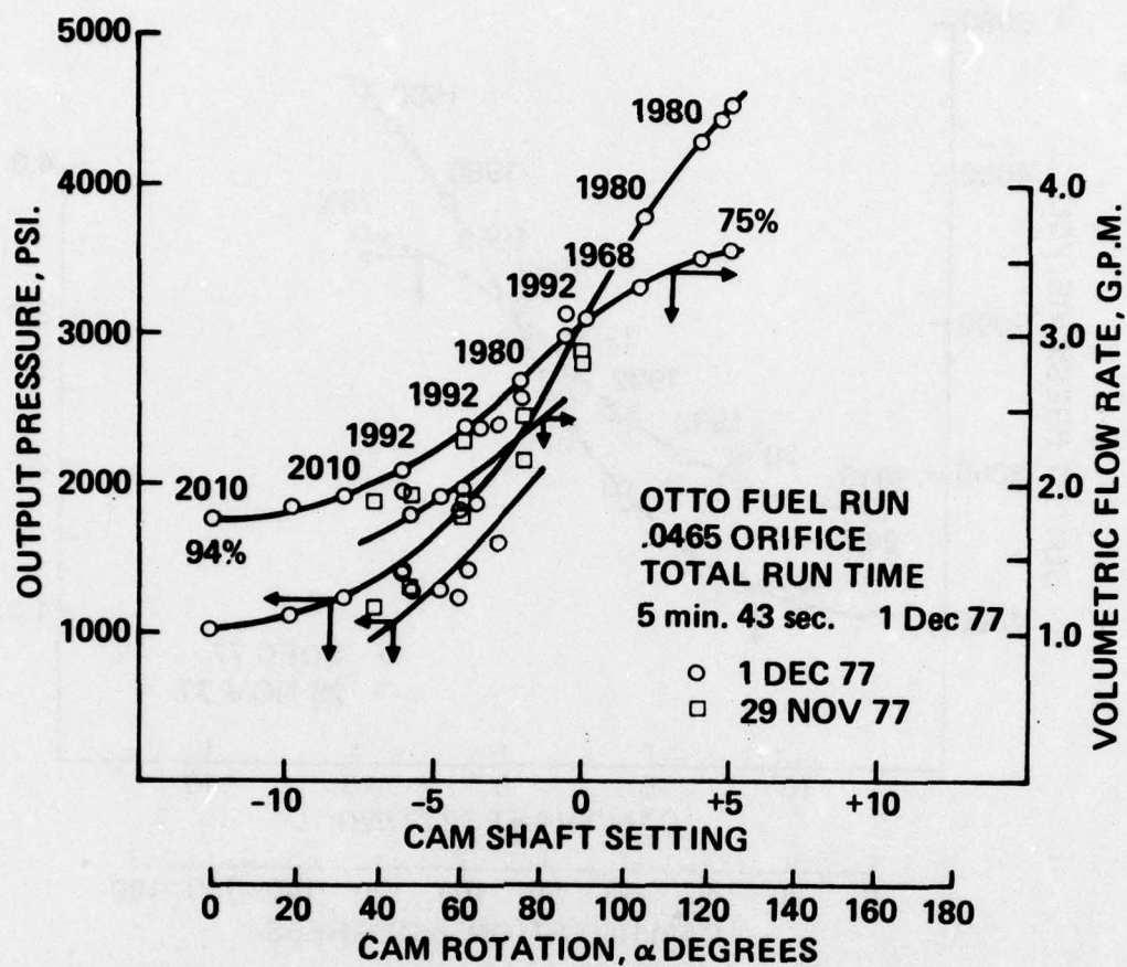
Figure 51. VD fuel pump (reworked) performance run with Otto fuel (40-deg conical valve, 0.0465-in. orifice).
