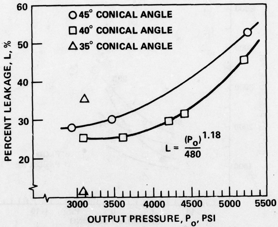
Figure 45. Internal leakage vs output pressure for valves of 35, 40, and 45 deg conical angle.
