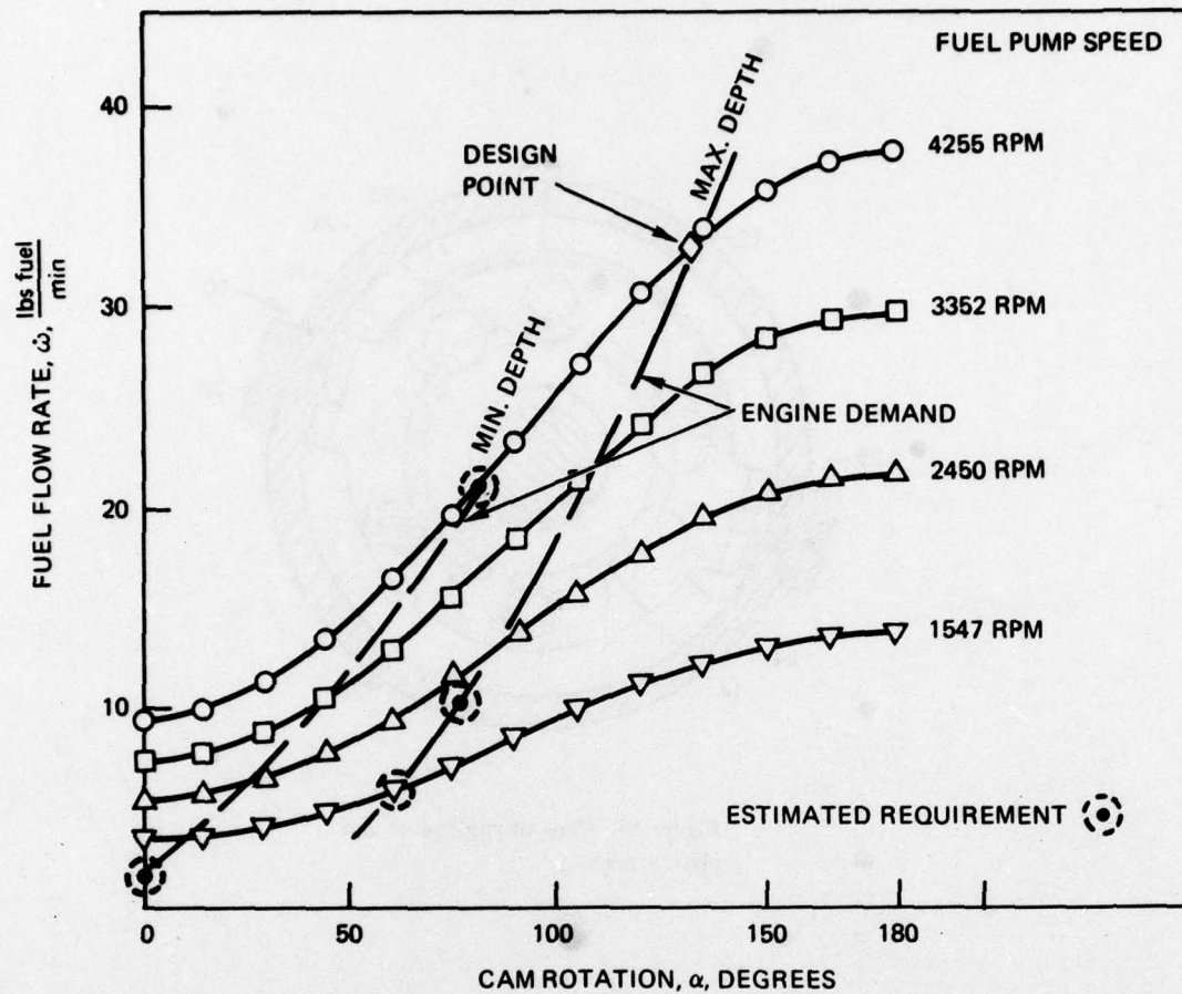
Figure 17. Theoretical performance, VD fuel pump.
