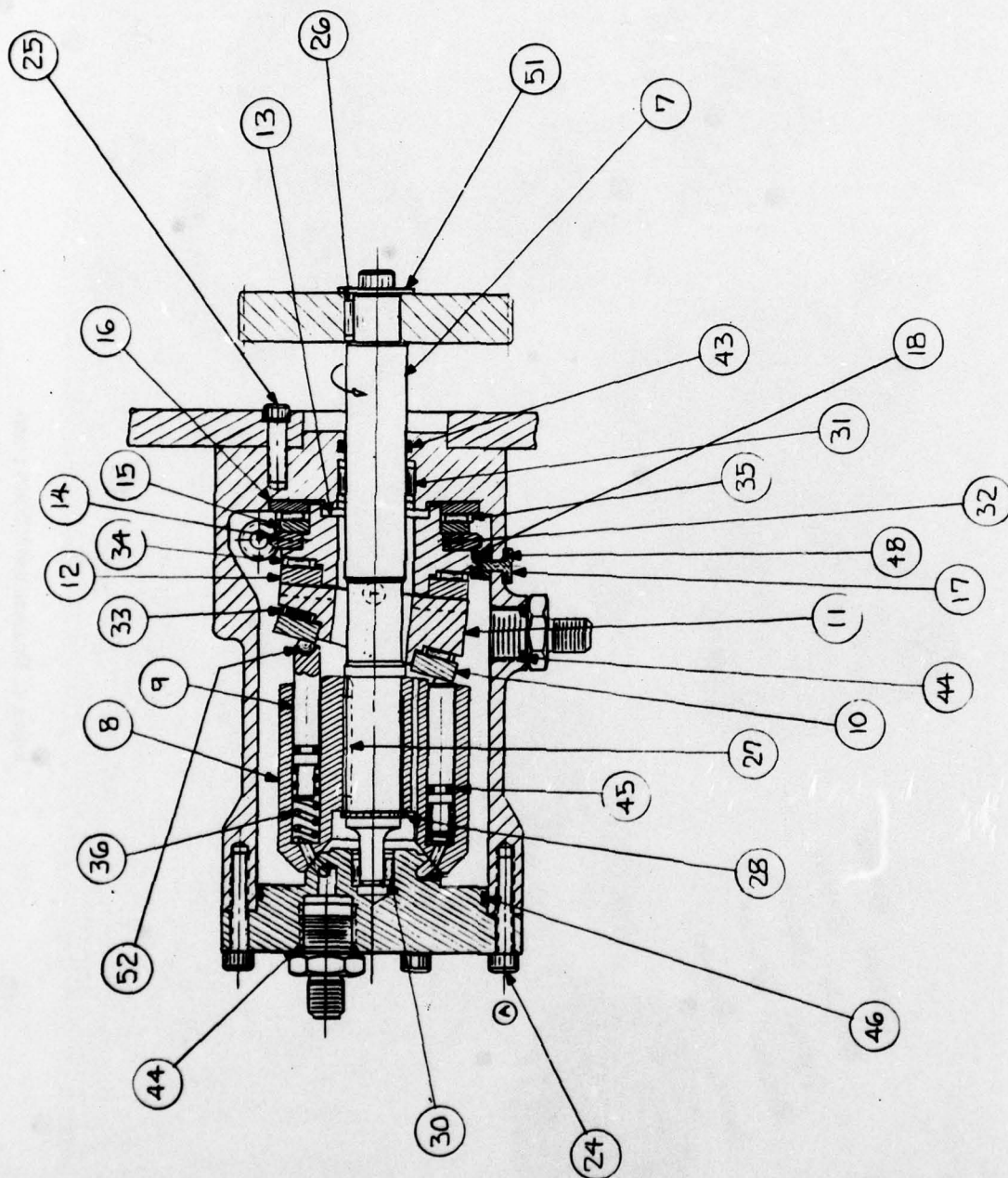
Figure 3. Assembly, VD fuel pump.
