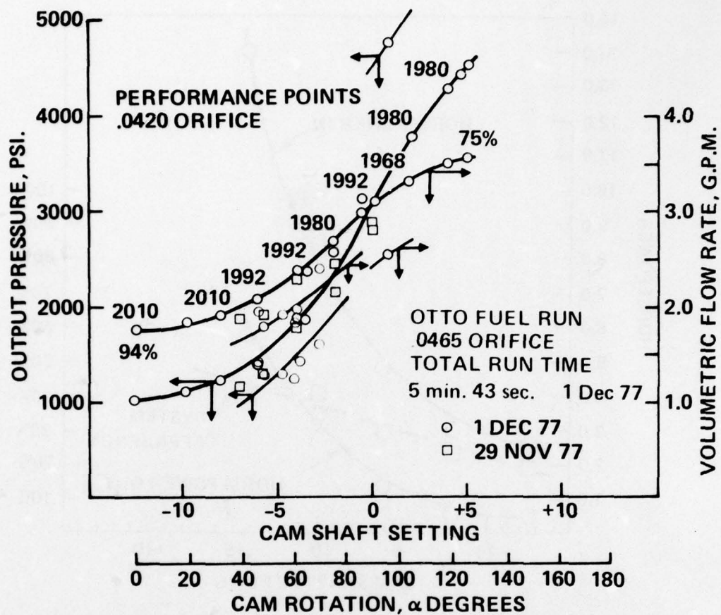
Figure 8. VD fuel pump (reworked) performance (40-deg conical valve, 0.0465-in. orifice).
