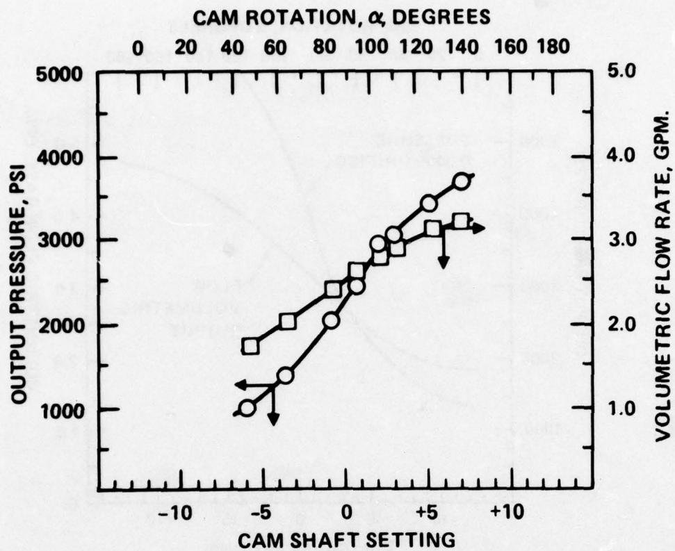
Figure 6. VD fuel pump performance (40-deg conical valve, 0.0465-in. orifice, C = 0.79 ).
