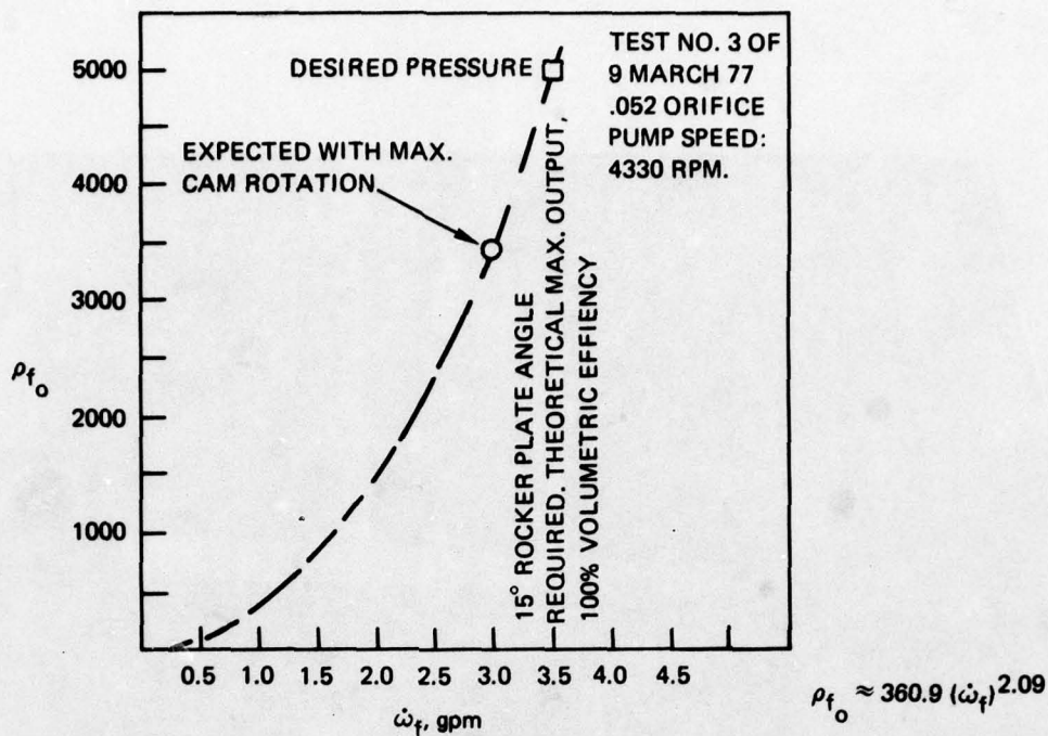
Figure 28. Theoretical analysis of VD fuel pump data of 9 and 16 March 1977.
