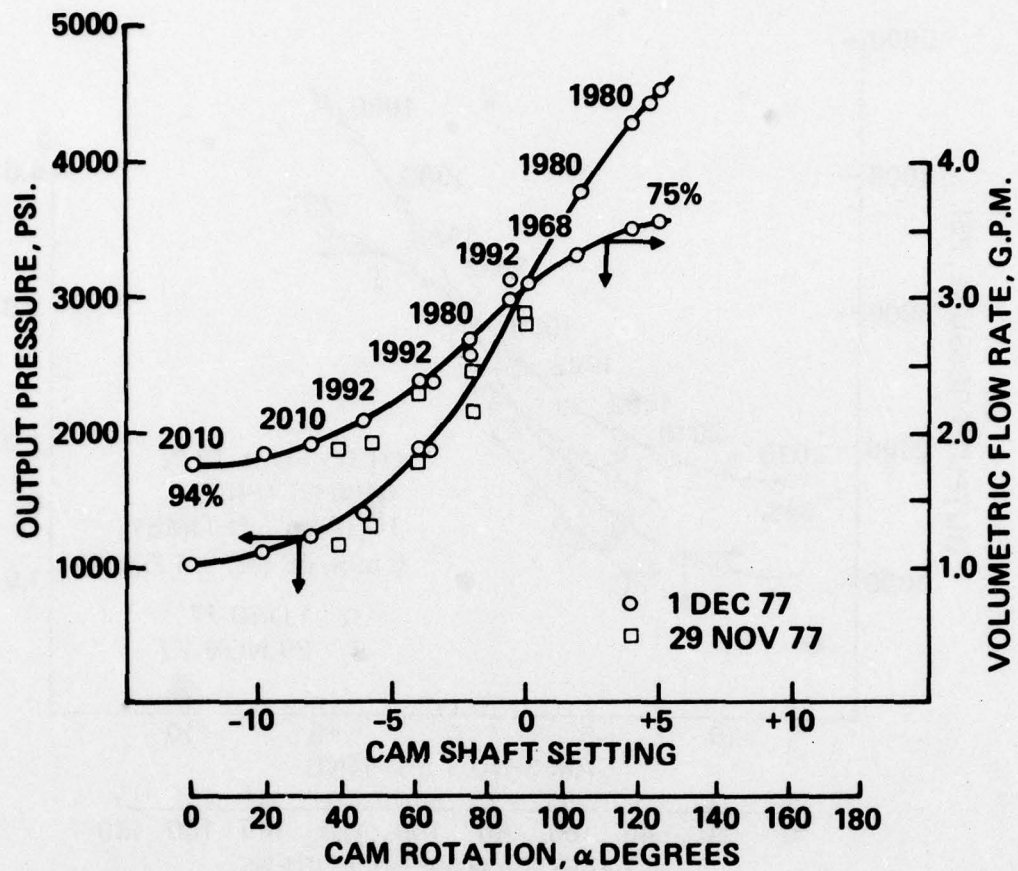
Figure 50. VD fuel pump (reworked) performance (40-deg conical valve, 0.0465-in. orifice).
