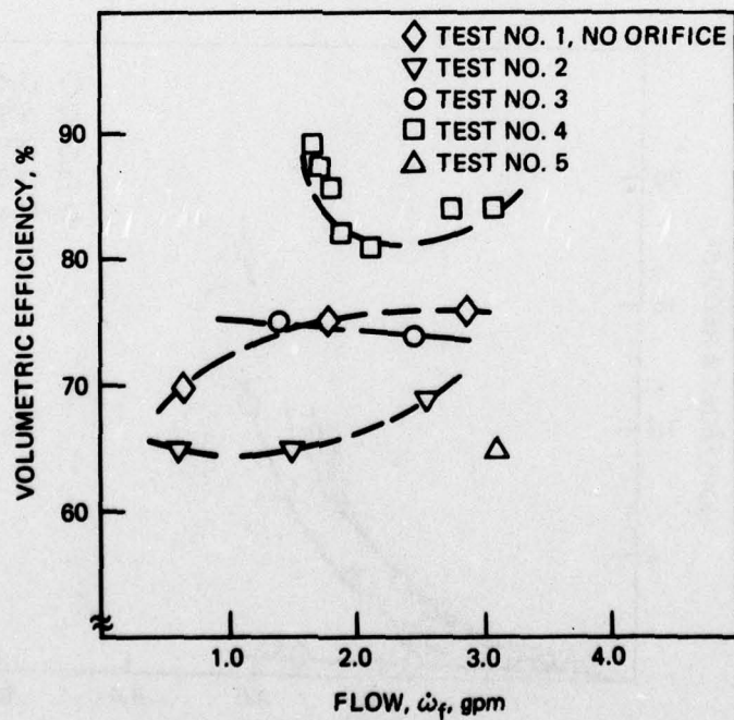
Figure 33. VD fuel pump volumetric efficiency. Data of 20-21 June, 1977.
