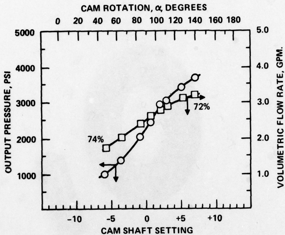
Figure 39. VD fuel pump performance (45-deg conical valve, 0.0465-in. orifice, C = 0.79 ).
