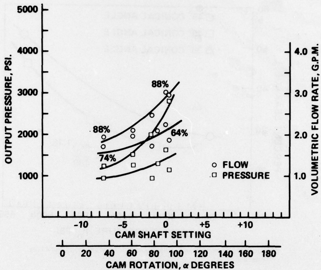
Figure 44. VD fuel pump performance (35-deg conical valve, 0.0465-in. orifice).
