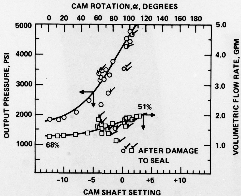
Figure 46. VD fuel pump performance (0.038-in. orifice, C = 0.64 ).
