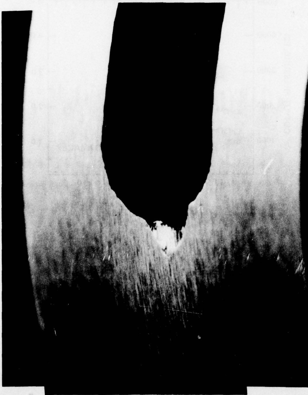
Figure 47. Damaged intake slot of pump head.
