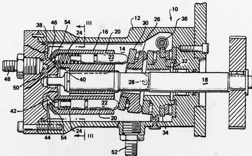
Figure 20. Conical valve design, cross-sectional view.
