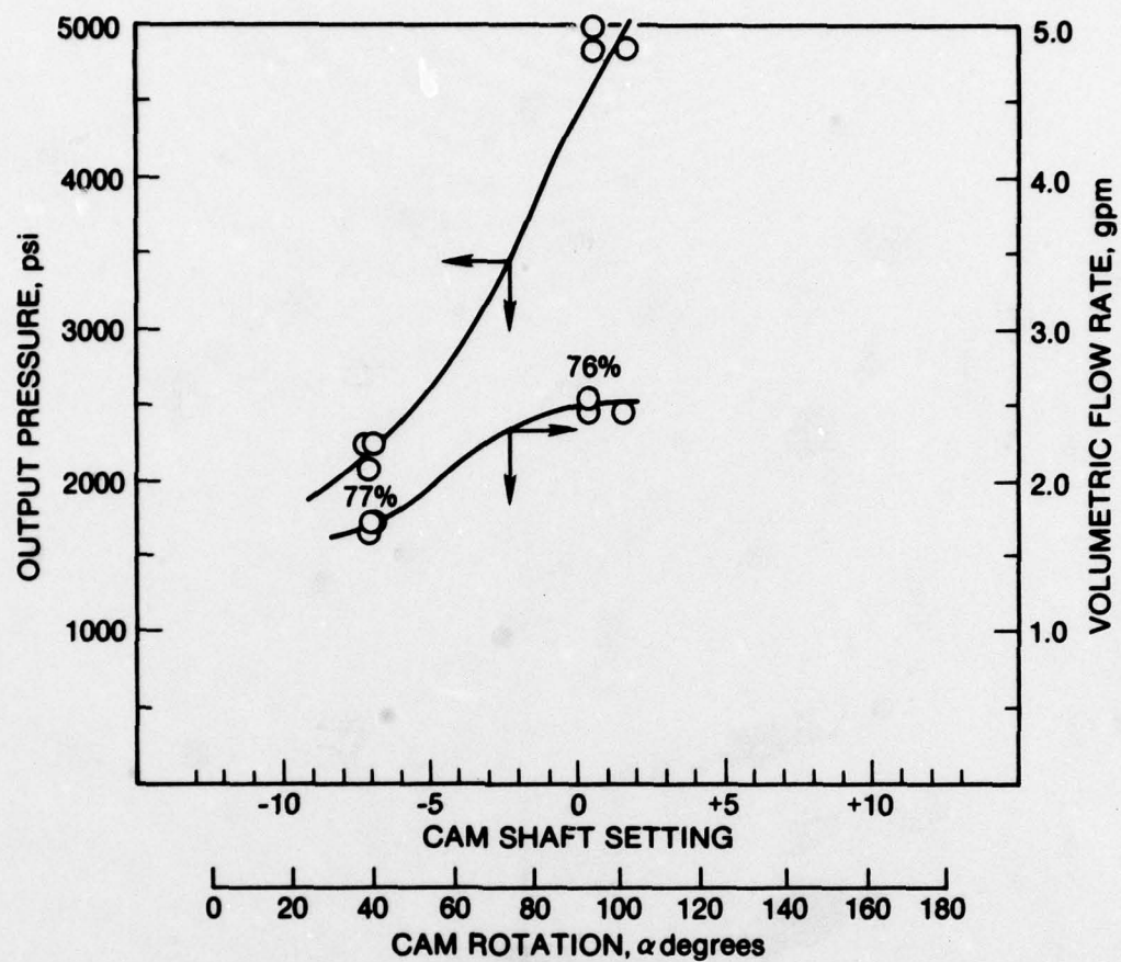
Figure 54. VD fuel pump performance (40-deg conical valve, 0.043-in. orifice). Data of 5 May 1978.
