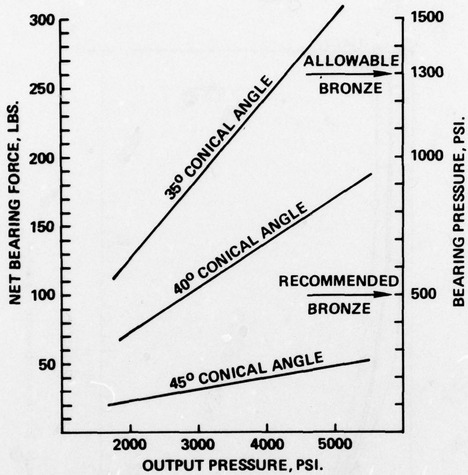
Figure 23. Bearing force and pressure vs output pressure and conical angle.
