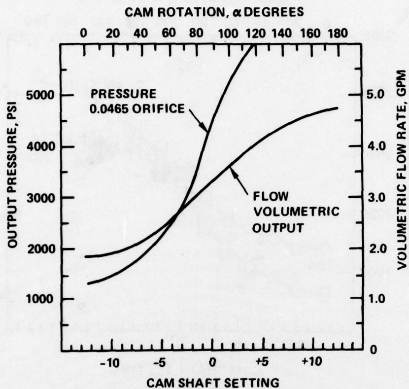
Figure 40. VD fuel pump performance, theoretical 100% efficiency.
