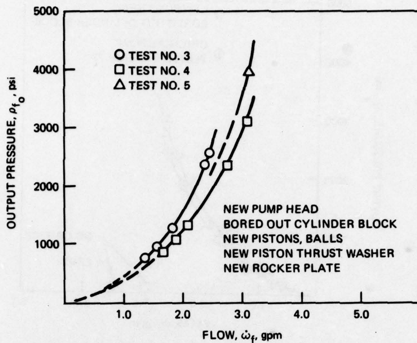
Figure 34. VD fuel pump performance (6- to 15-deg angle-plate, 0.052-in. orifice). Data of 20 June 1977.
