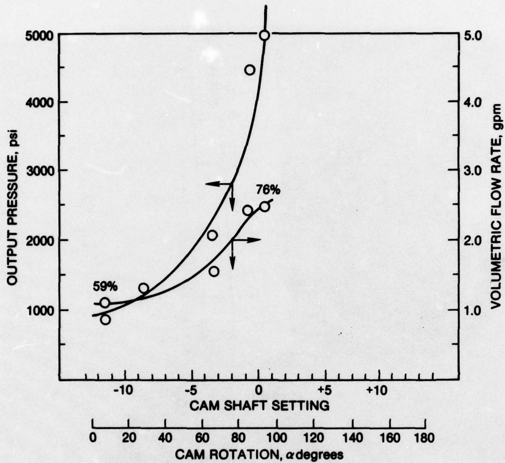
Figure 52. VD fuel pump performance (30-deg conical valve, 0.043-in. orifice). Data of 28 March 1977.
