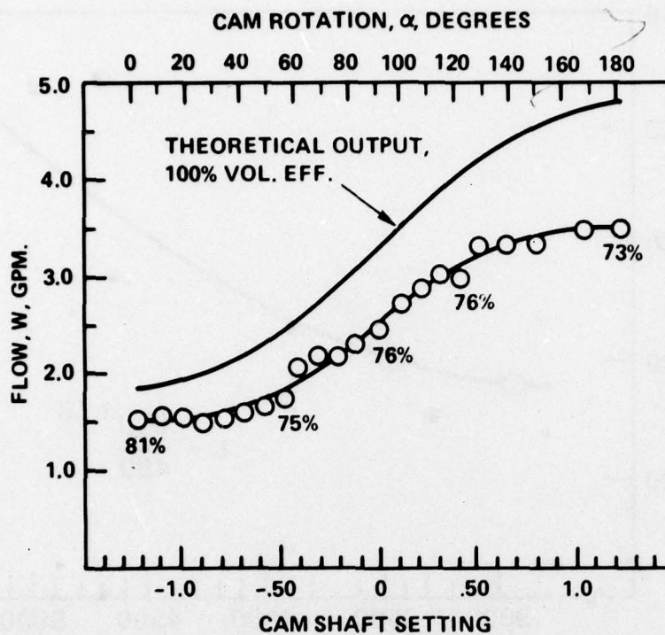
Figure 36. VD fuel pump output vs cam rotation for 45-deg conical valve, 0.052-in. orifice. Circles indicate actual data of 12 July 1977. Percentages shown are actual volumetric efficiencies. Teflon O-rings were used on the pistons.
