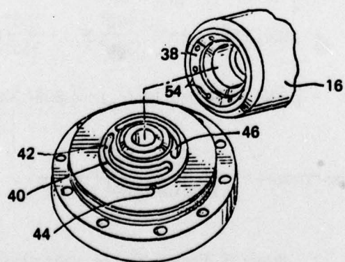
Figure 21. Conical valve design, perspective view.
