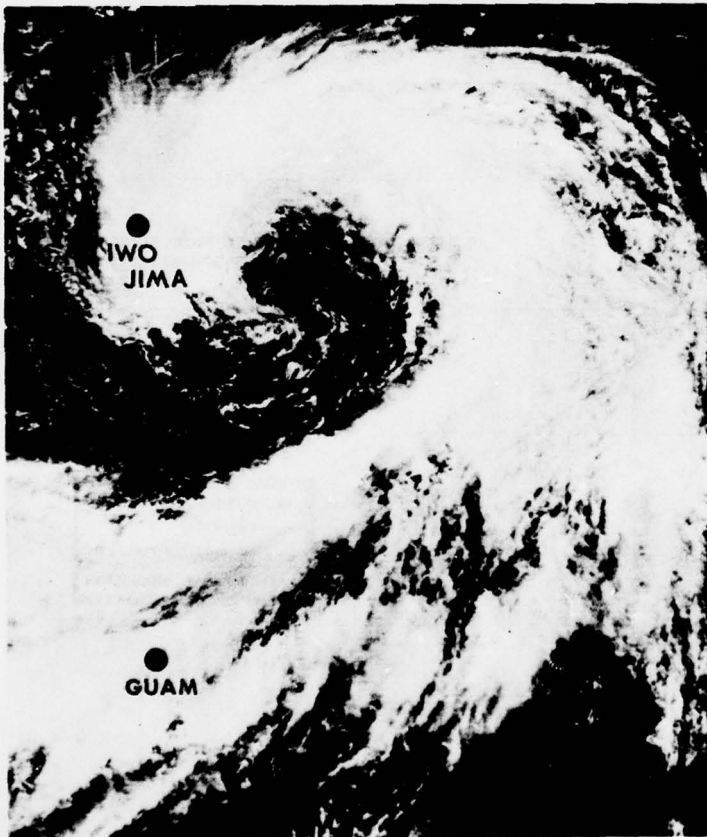
Figure 13 - Satellite view of tropical storm Mary centered 220 nm southeast of Iwo Jima, 14 August 1974 (0118 GMT). (U. S. Air Force Weather Service DMSF data)
