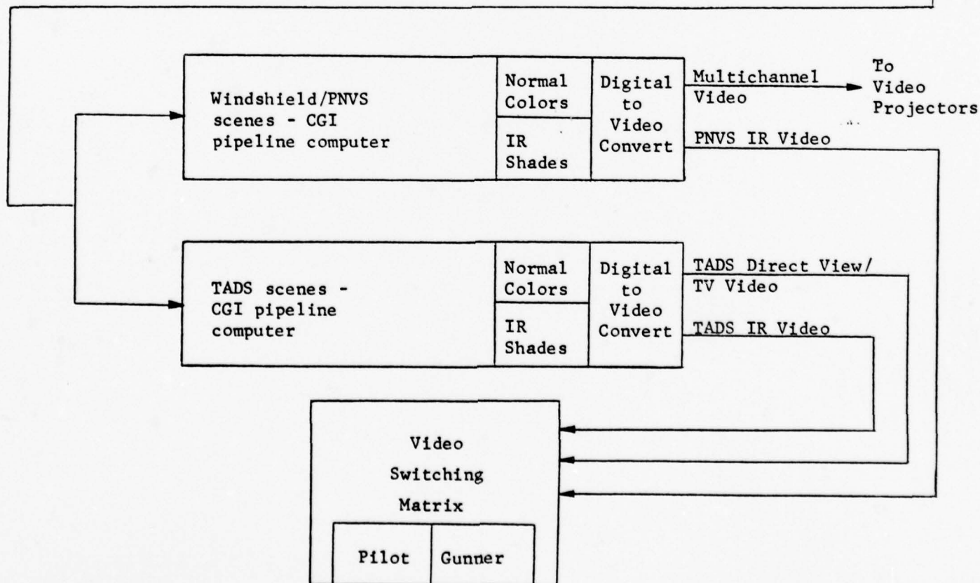
Block Diagram of Visual Module for Pilot/Gunner Trainer
