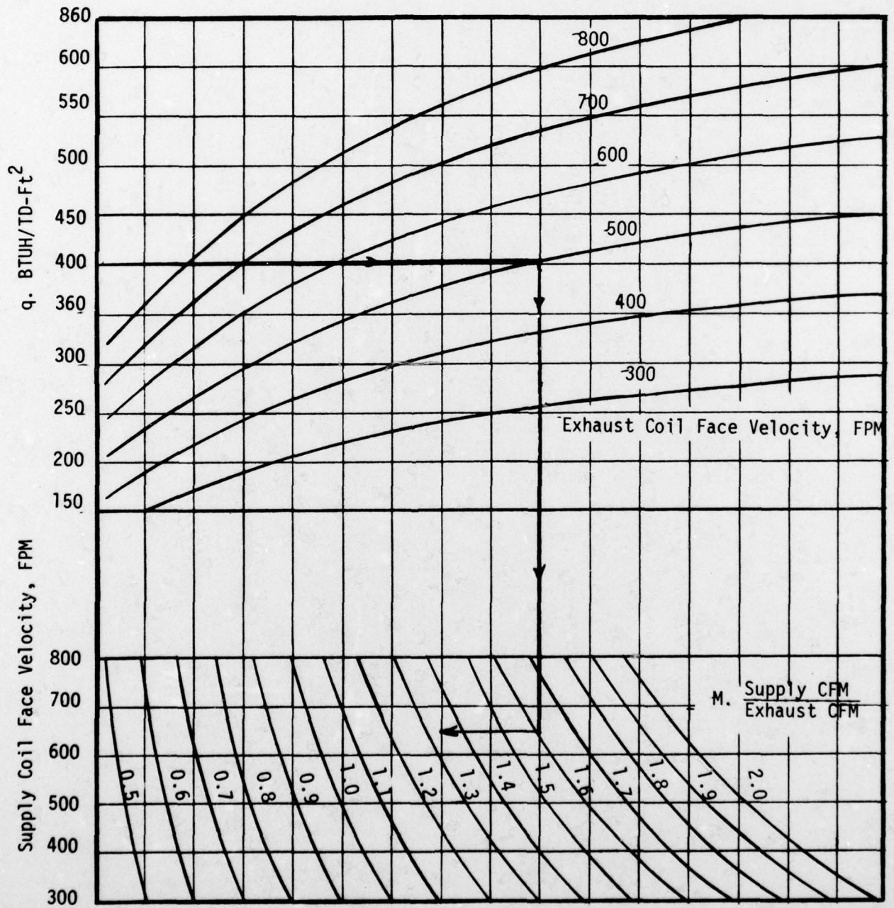
Typical Run-Around System Operating Performance.
