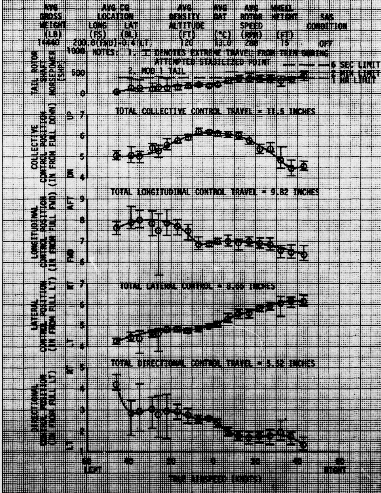
FIGURE 31 SIDEWARD FLIGHT YAN-84 USA S/N 74-22246
