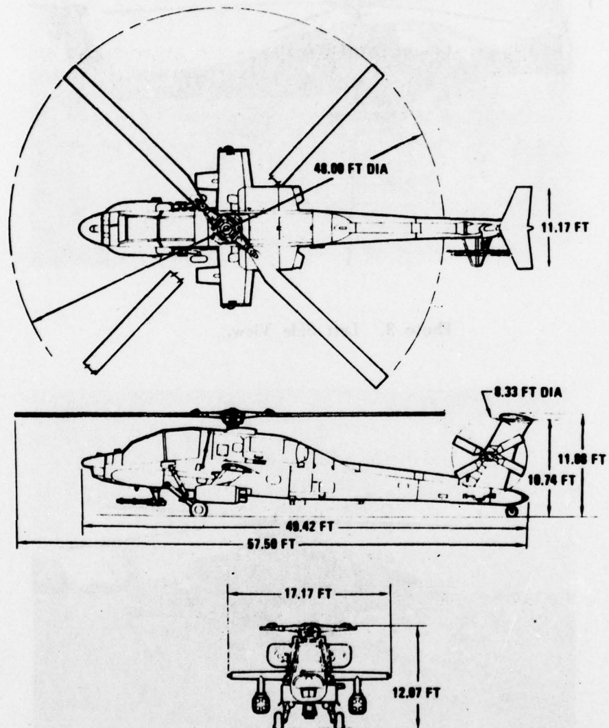
Figure 1. Dimensions.
