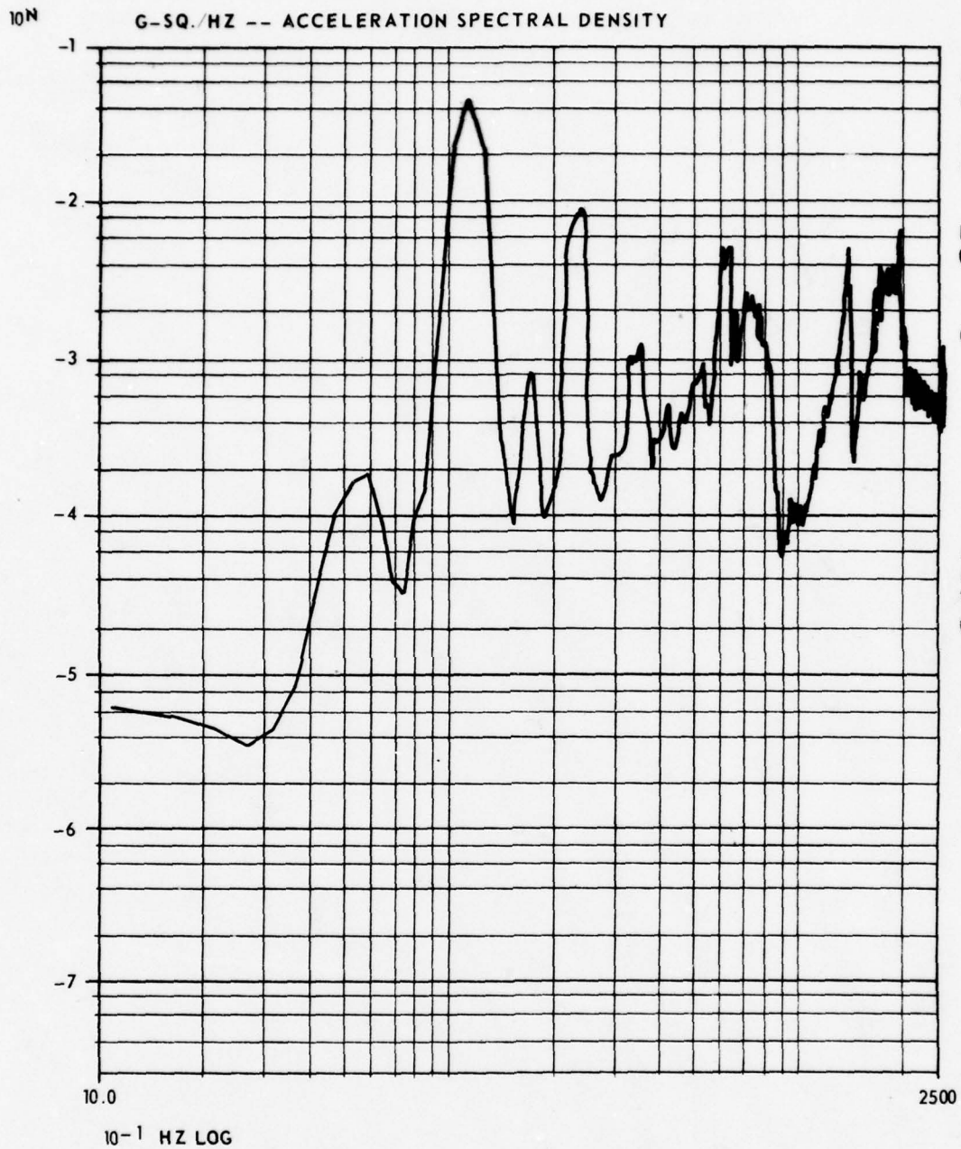
FIGURE 4-4. PSD PLOT OF MISSILE-BOTTOM-CENTER ACCELERATION RESPONSE, VERTICAL RANDOM TEST 7 WITHOUT AVI
