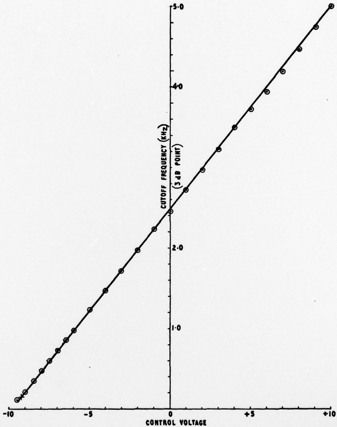
FIG. 12 FILTER CHARACTERISTIC.
