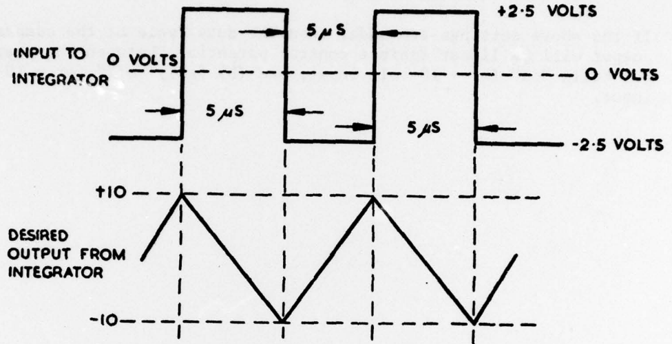
FIG. 6 IDEAL WAVEFORMS - INTEGRATOR.
